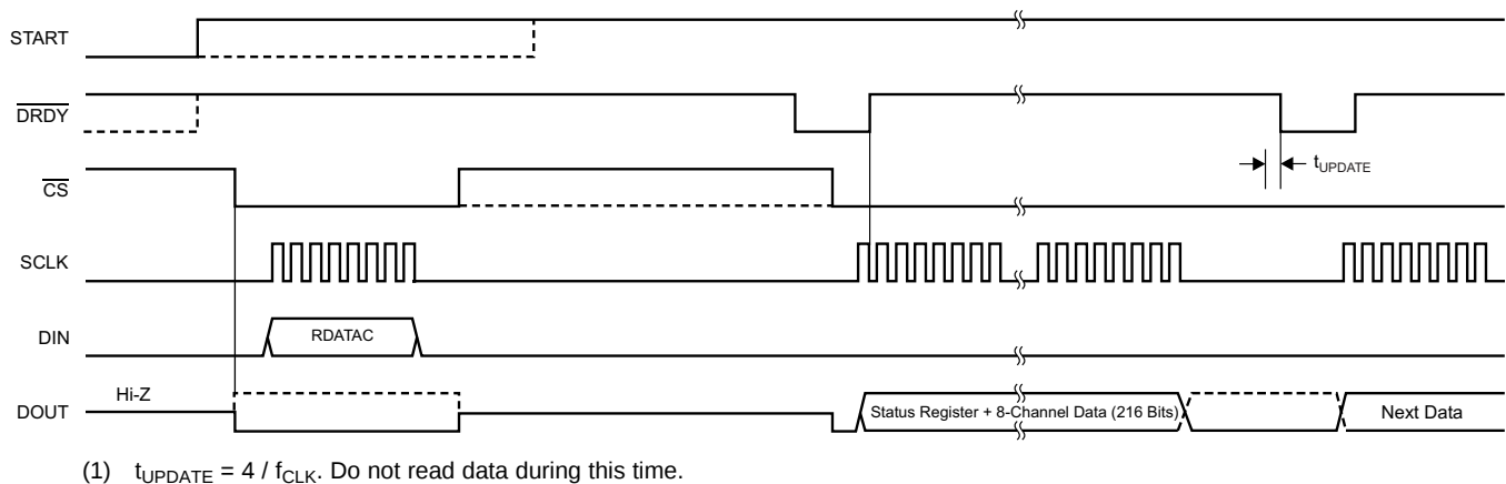
Figure 46. RDATA Usage
