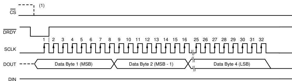
图 59. Read-Data-Continuous Mode
