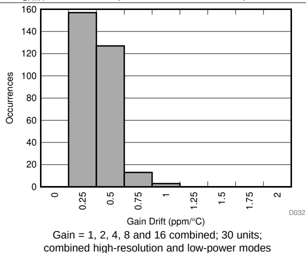
图 39. Gain Drift Histogram
