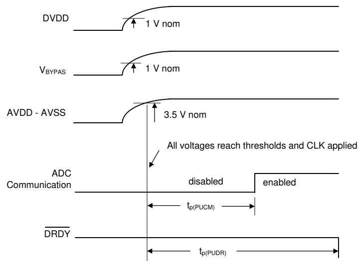
图 7. Power-Up Timing
