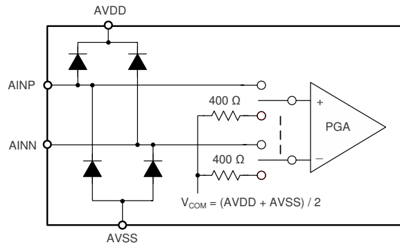
图 44. Analog Input and Multiplexer
