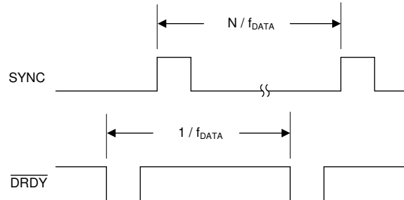
图 58. Continuous-Sync Mode
