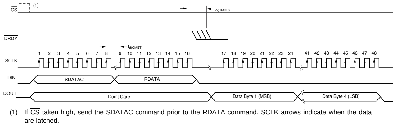
图 60. Read Data By Command Mode
