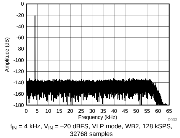
Figure 13. Output Spectrum
