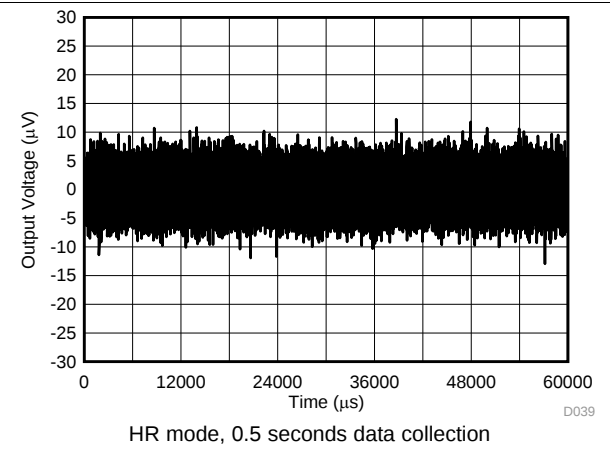
Figure 17. ADC Conversion Noise
