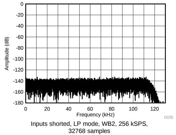
Figure 15. Output Spectrum
