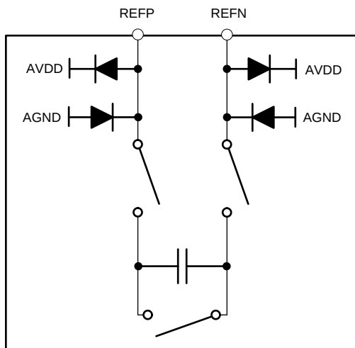
Figure 80. Equivalent Reference Input Circuitry
