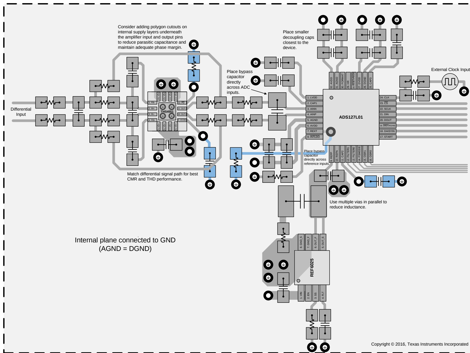
Figure 131. Layout Example
