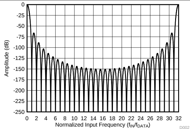
Figure 63. Low-Latency Filter Frequency Response (OSR 32) to f_{\text{CLK}}
