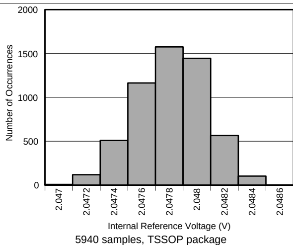
图 26. Internal Reference Voltage Histogram
