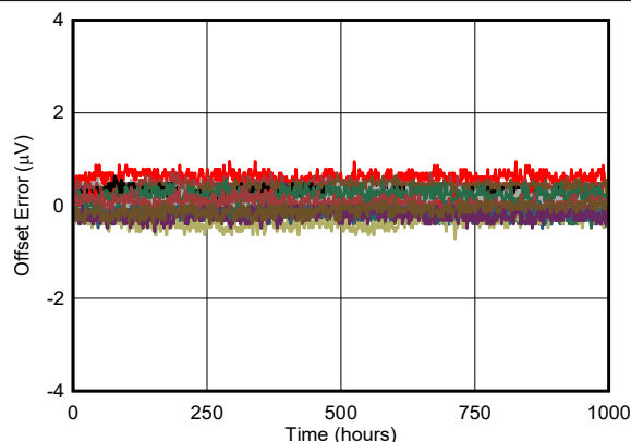
图 6-30. Long-Term Offset Drift
