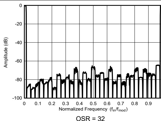
图 8-11. Wideband Filter Stop-Band Attenuation
