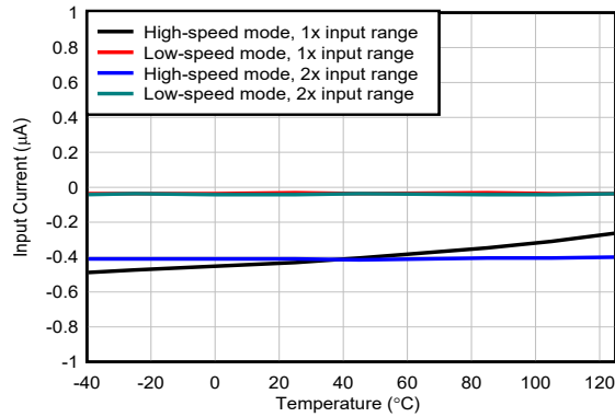
图 6-24. Input Current vs Temperature
