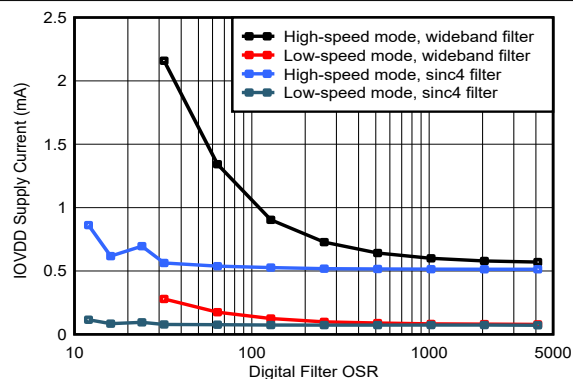
图 6-45. IOVDD Current vs Oversampling Ratio
