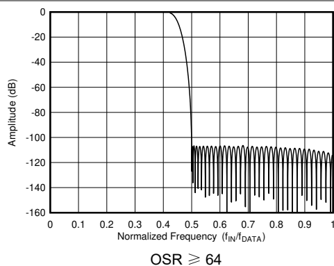
图 8-10. Wideband Filter Frequency Response
