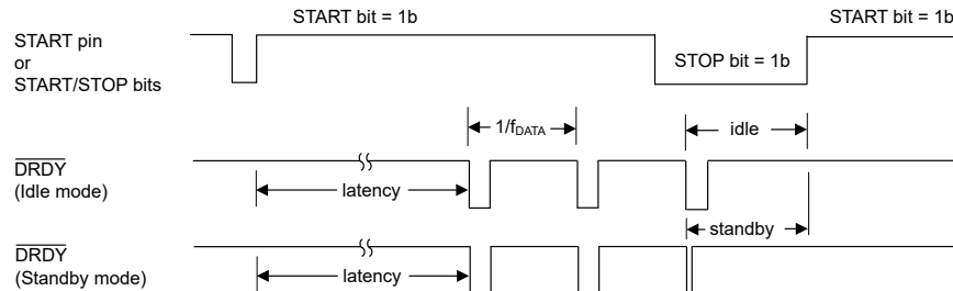
图 8-26. Start/Stop Control Mode
