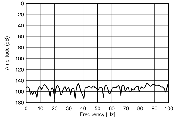
图 6-7. Shorted Input FFT (0-Hz to 100-Hz Detail)
