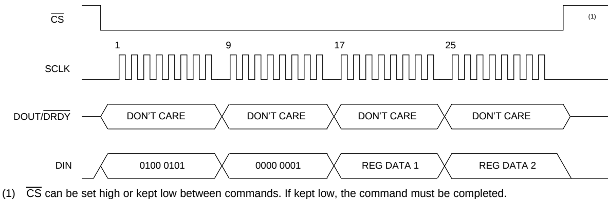
图 89. Write Register Sequence
