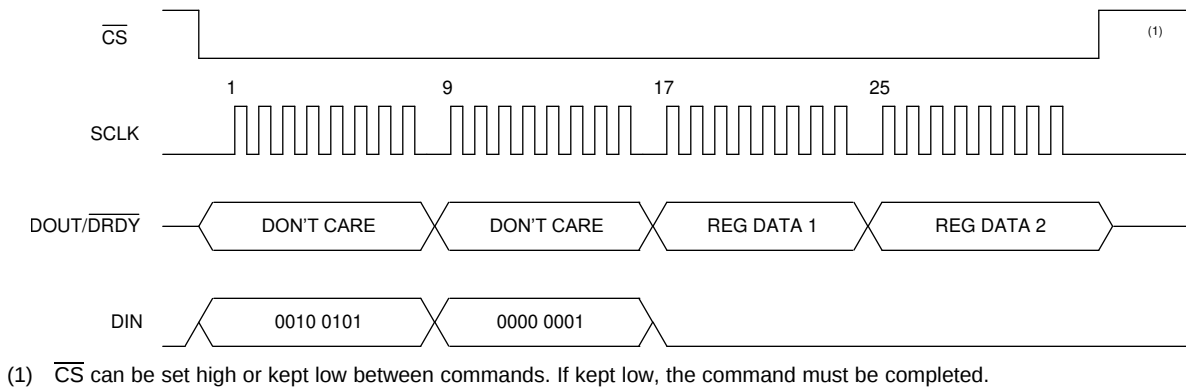
图 74. Read Register Sequence
