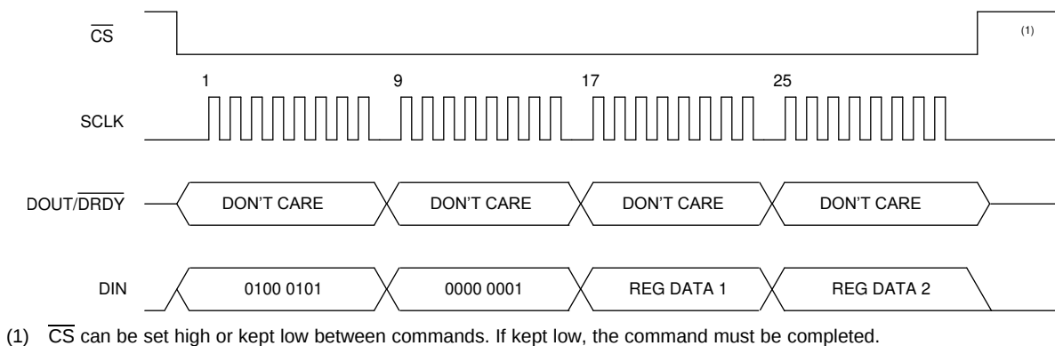
图 75. Write Register Sequence
