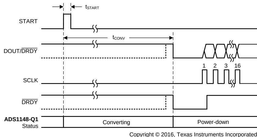
Figure 36. Timing for a Single Conversion Using the START Pin
