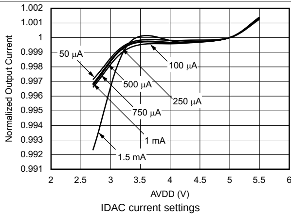
Figure 7. IDAC Line Regulation
