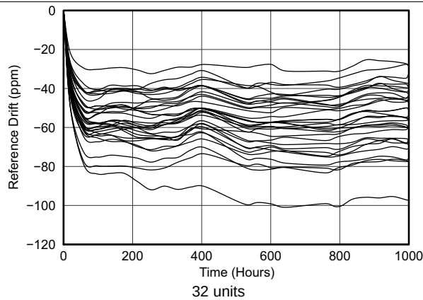
Figure 5. Internal Reference Long-Term Drift
