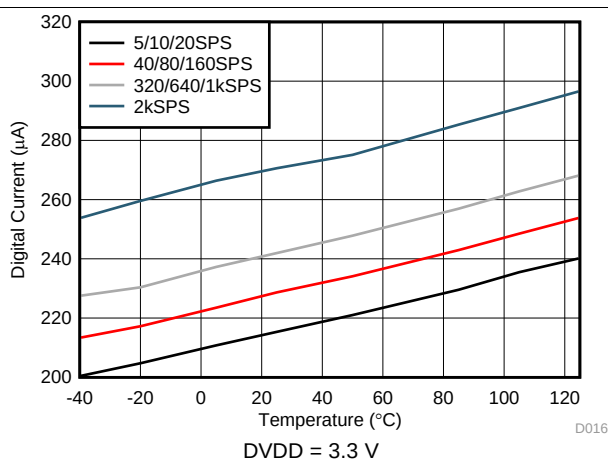
Figure 16. Digital Supply Current vs Temperature
