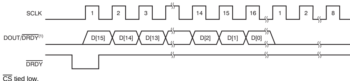
Figure 39. Data Retrieval With the \overline{\text{DRDY}} \text{ MODE} Bit = 0 (Disabled)
