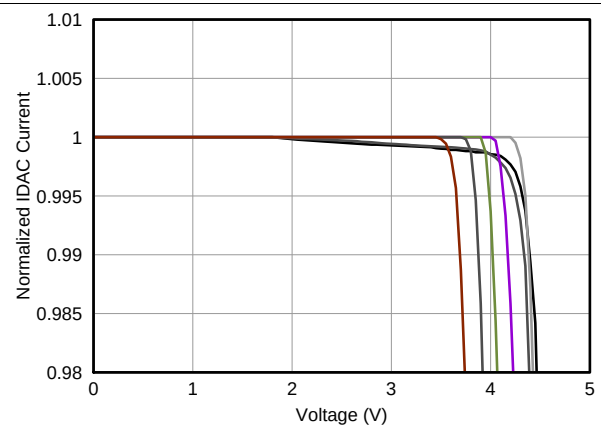
Figure 8. IDAC Drift
