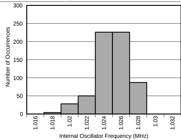
图 17. Internal Oscillator Frequency Histogram
