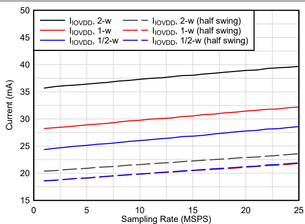
图 6-39. IOVDD Current vs Interface
