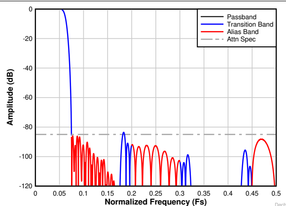
图 8-31. Decimation by 8 complex frequency response
