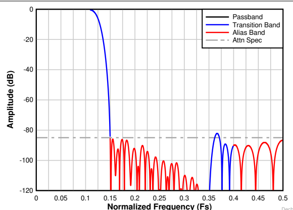
图 8-29. Decimation by 4 complex frequency response
