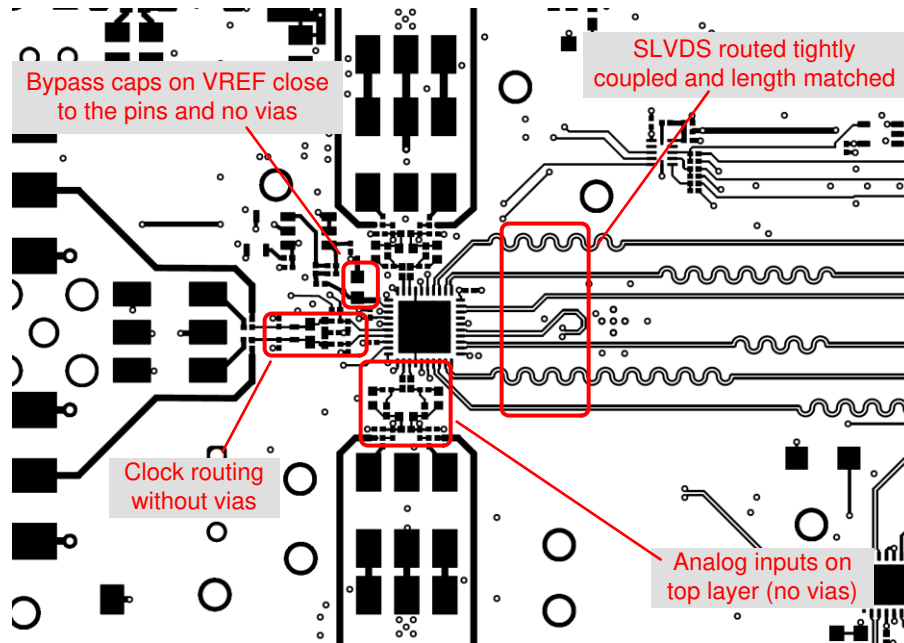
图 9-10. Layout example: top layer of ADC366x/368x EVM
