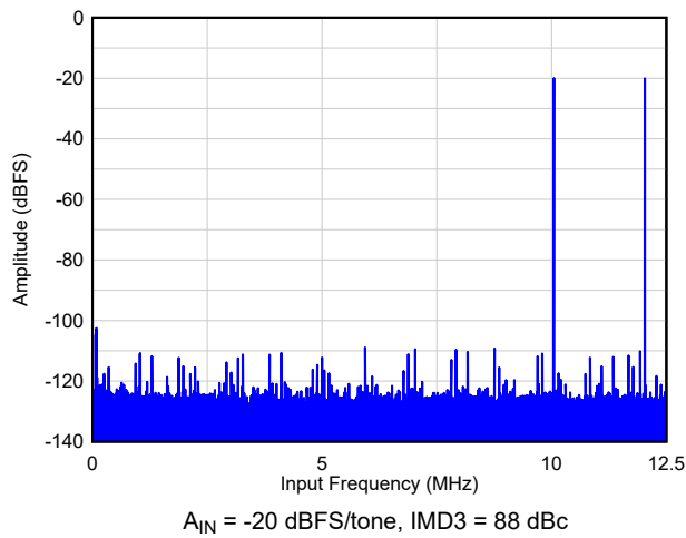
图 6-26. Two Tone FFT at F_{IN} = 10/12\text{ MHz}
