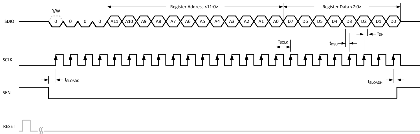
图 8-52. Serial Register Write Timing Diagram
