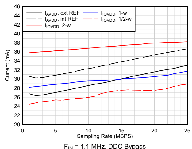
图 6-37. Current vs Sampling Rate
