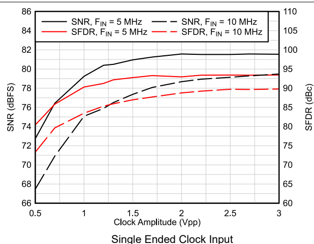
图 6-55. AC Performance vs Clock Amplitude
