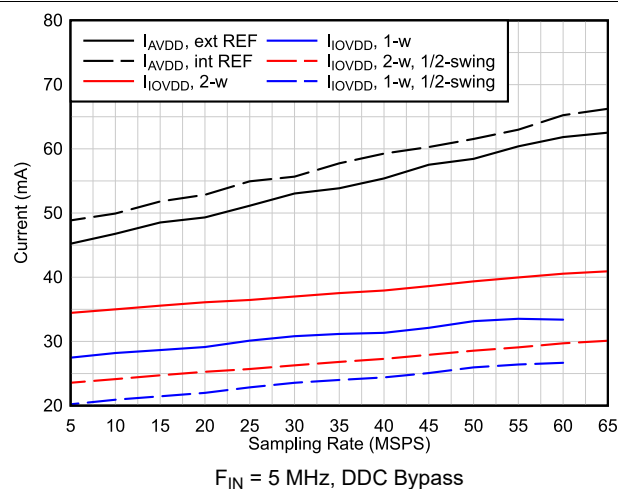
图 6-62. Current vs Sampling Rate
