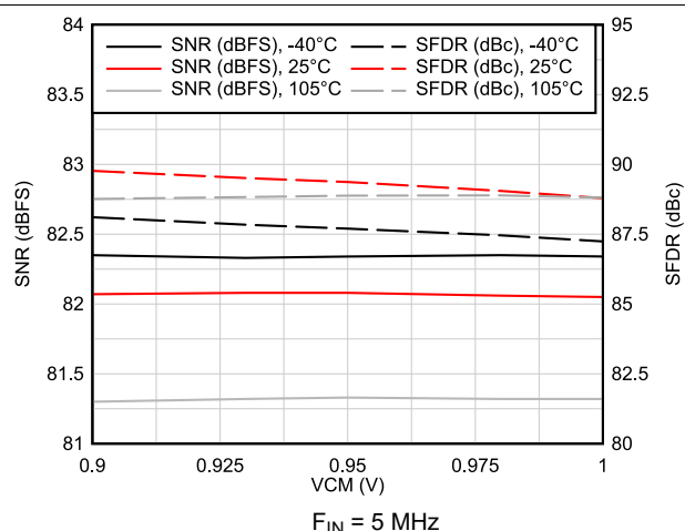
图 6-57. AC Performance vs VCM vs Temperature
