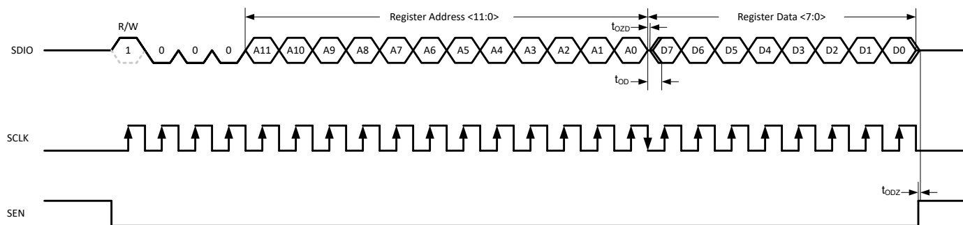
图 8-53. Serial Register Read Timing Diagram
