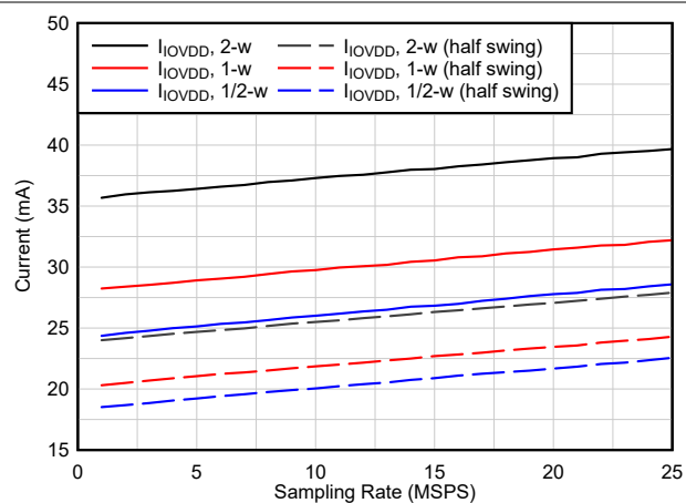
图 6-39. I_{IOVDD} Current vs Interface
