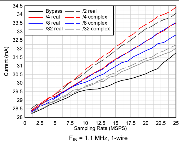
图 6-38. I_{IOVDD} Current vs Decimation
