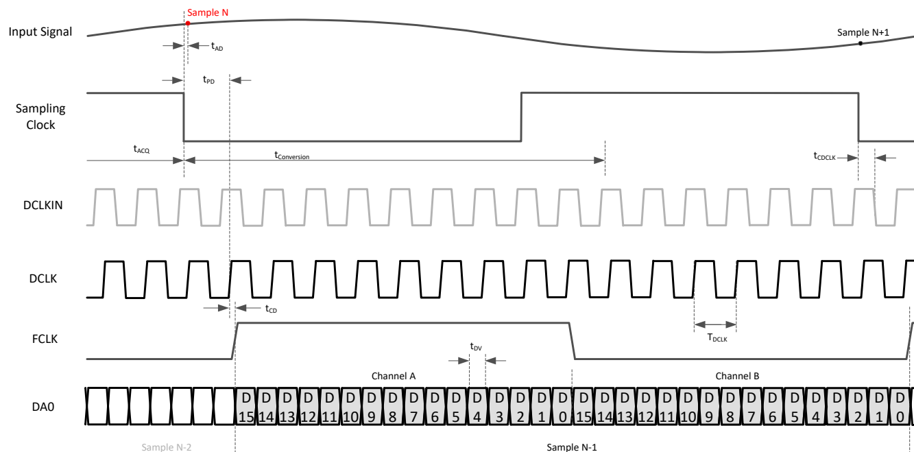
图 7-3. Timing diagram:1/2-wire SLVDS (default output bit mapper)
