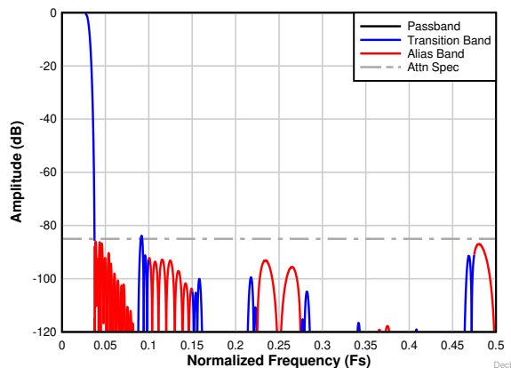
图 8-29. Decimation by 16 complex frequency response
