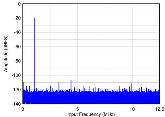
图 6-23. Single Tone FFT at F_{IN} = 1.1 \text{ MHz}
