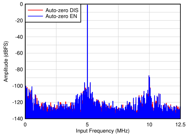
图 8-8. FFT at 25 MSPS with input frequency of 5 MHz (auto-zero feature enable vs disable, 4M point FFT)
