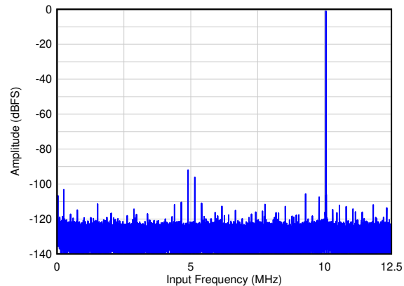
图 6-24. Single Tone FFT at F_{IN} = 10 \text{ MHz}
