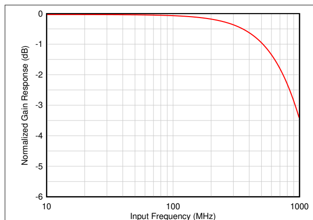
图 8-2. ADC Analog Input Bandwidth Response
