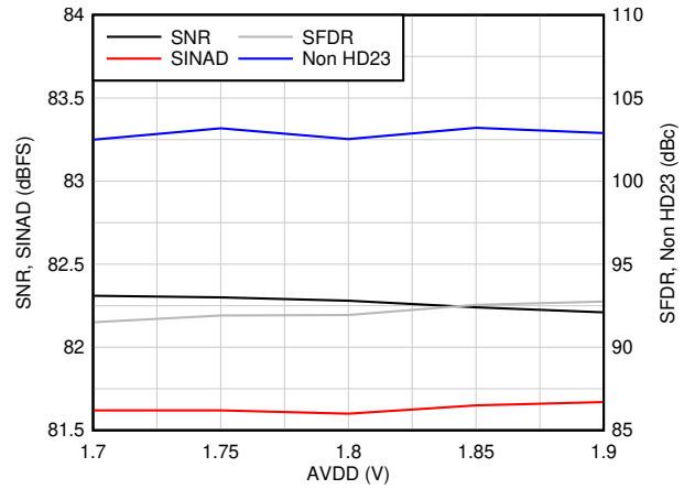
图 6-30. AC Performance vs AVDD
