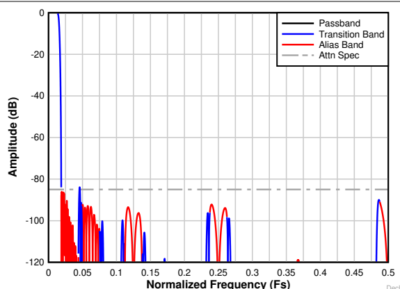
图 8-31. Decimation by 32 complex frequency response
