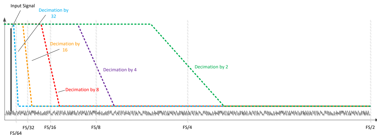
图 8-20. Real decimation illustration
