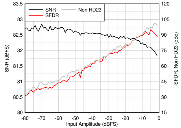
图 6-12. AC Performance vs Input Amplitude
