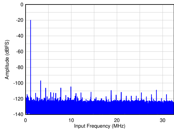
图 6-2. Single Tone FFT at F_{IN} = 1.1\text{ MHz}
