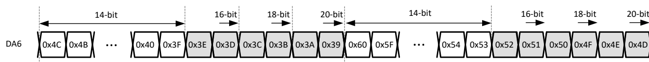
图 8-42. 1/2-wire output bit mapping
