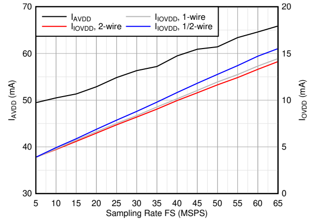
图 6-36. Current vs Sampling Rate
