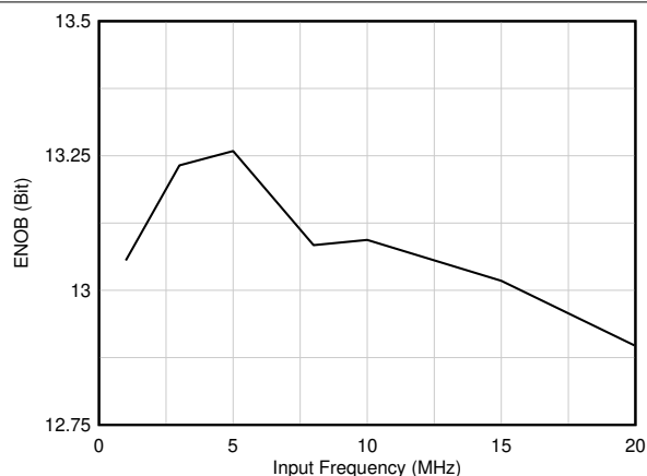
图 6-27. ENOB vs Input Frequency
