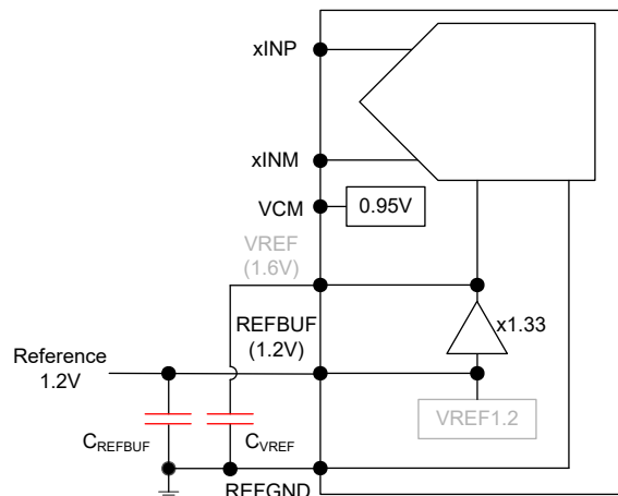
图 8-16. External 1.2V reference using internal reference buffer
