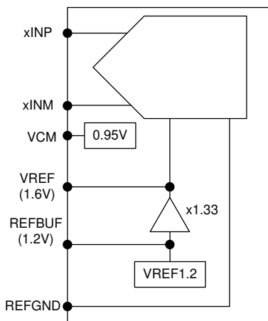
图 8-17. Different voltage reference options for ADC358x
