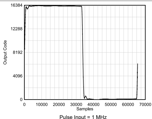
图 6-20. Pulse Response
