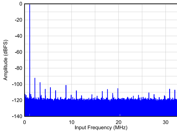
图 6-39. Single Tone FFT at F_{IN} = 1.1\text{ MHz}
