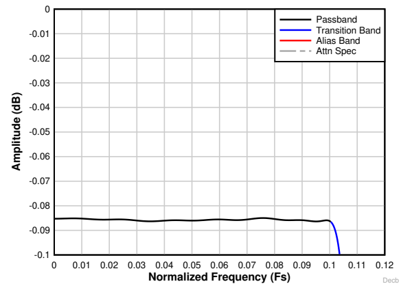
图 8-28. Decimation by 4 complex passband ripple response
