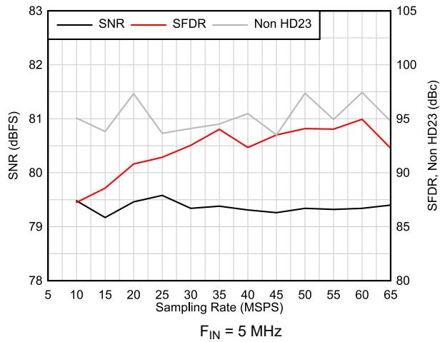
图 6-51. AC Performance vs Sampling Rate
