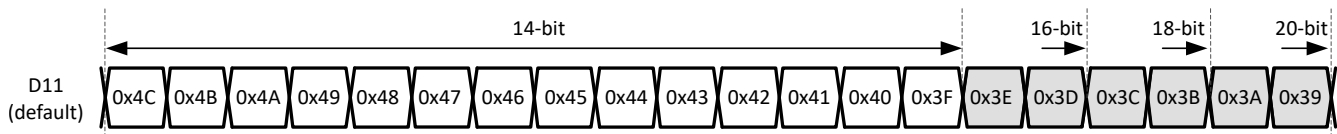
图 8-47. 1-wire output bit mapping
