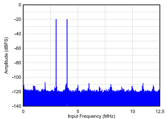
图 6-23. Two Tone FFT at F_{IN} = 3, 4 MHz
