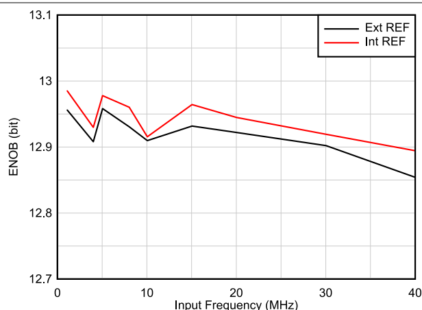
图 6-26. ENOB vs Input Frequency
