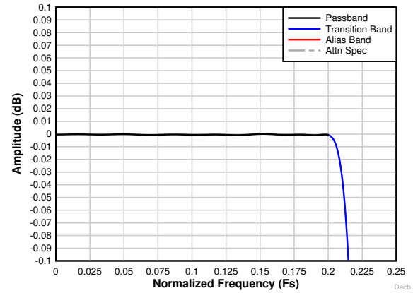
图 8-26. Decimation by 2 complex passband ripple response
