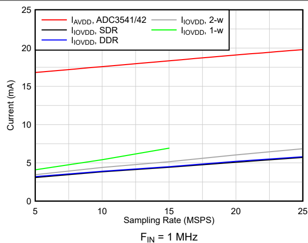
图 6-36. Current vs Sampling Rate
