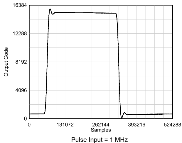
图 6-58. Pulse Response
