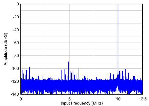
图 6-19. Single Tone FFT at F_{IN} = 10 MHz
