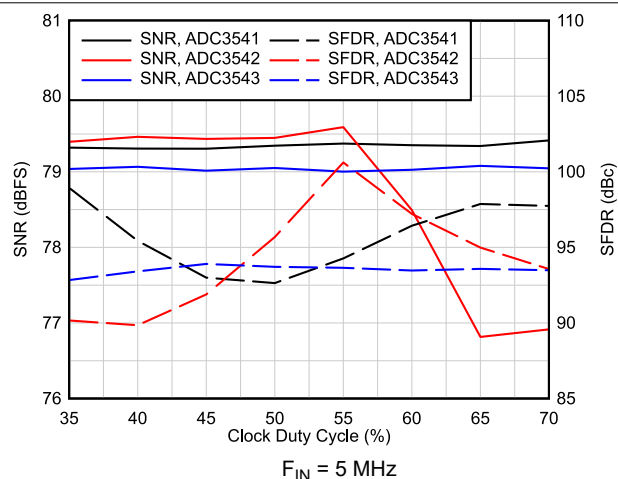
图 6-59. AC Performance vs Clock Duty Cycle
