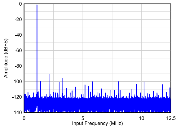
图 6-18. Single Tone FFT at F_{IN} = 1.1 MHz
