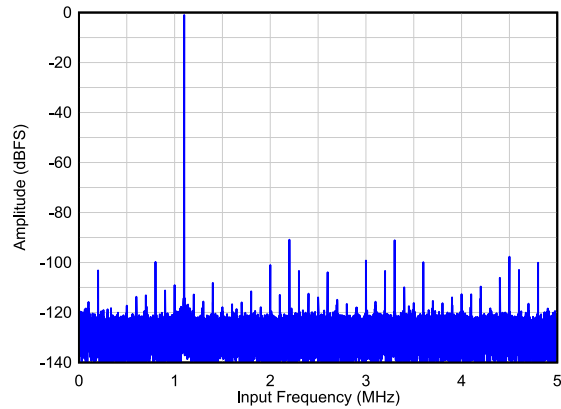
图 6-1. Single Tone FFT at F_{IN} = 1.1 MHz
