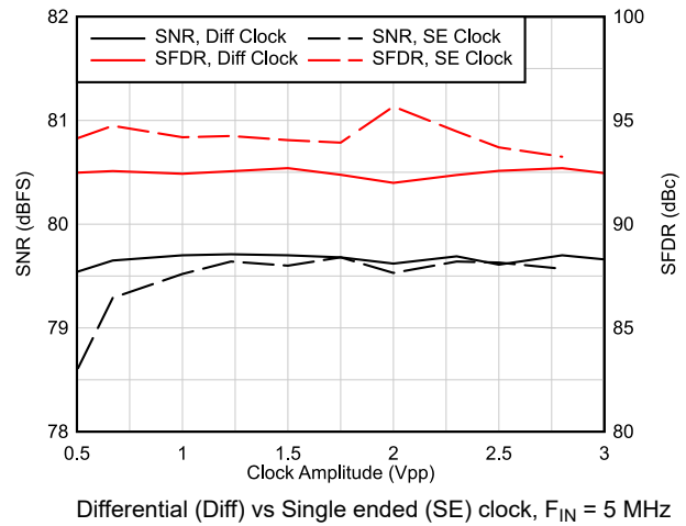
图 6-52. AC Performance vs Clock Amplitude
