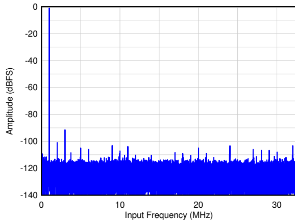
图 9-2. Single Tone FFT at F_{IN} = 1 MHz
