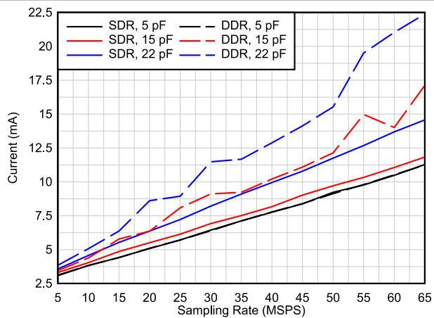
图 6-62. I_{OVDD} Current vs Output Interface
