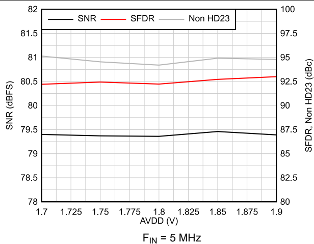
图 6-53. AC Performance vs AVDD
