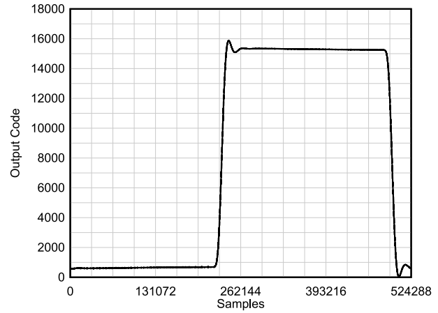
图 6-14. Pulse Response
