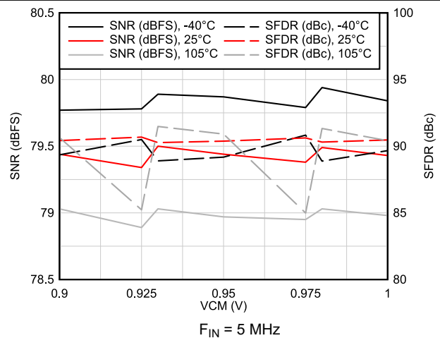
图 6-54. AC Performance vs VCM vs Temperature
