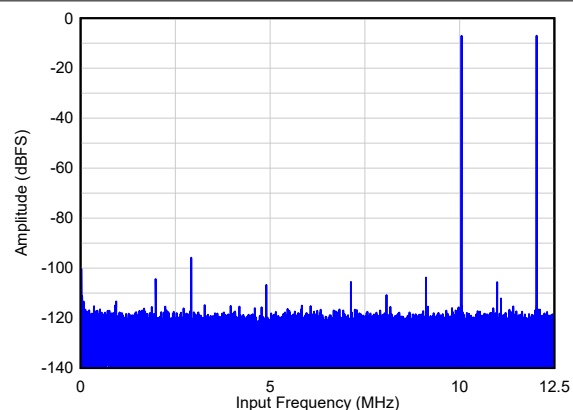
图 6-24. Two Tone FFT at F_{IN} = 10, 12 MHz
