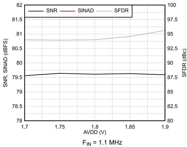
图 6-30. AC Performance vs AVDD
