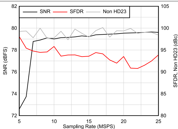
图 6-28. AC Performance vs Sampling Rate
