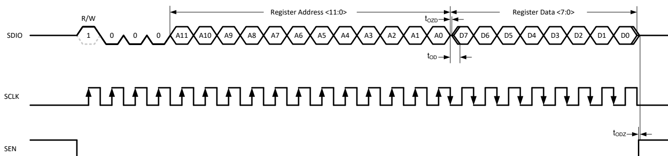
图 8-51. Serial Register Read Timing Diagram
