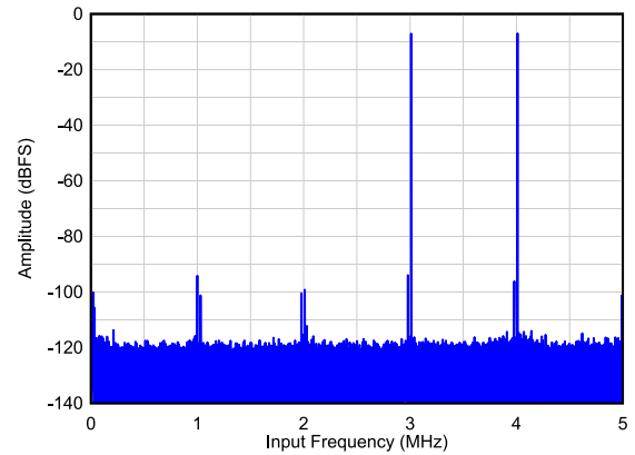
图 6-2. Two Tone FFT at F_{IN} = 3,4 MHz
