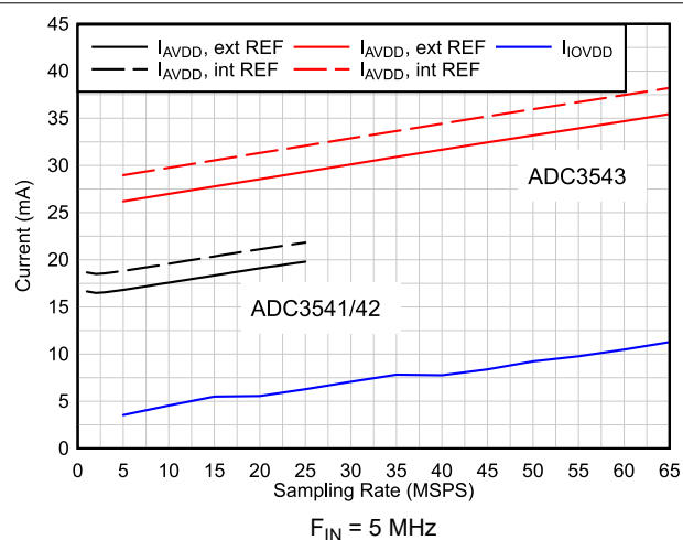
图 6-60. Current vs Sampling Rate
