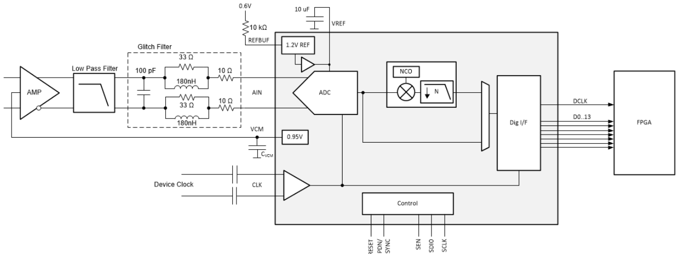
图 9-1. Typical configuration for a spectrum analyzer with DC support
