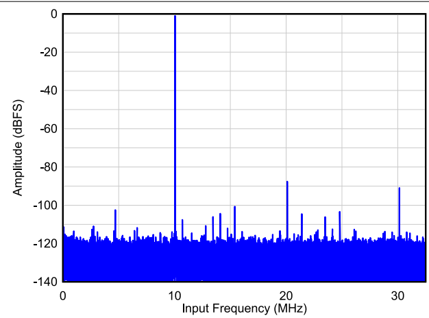
图 6-40. Single Tone FFT at F_{IN} = 10\text{ MHz}
