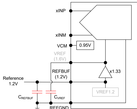
图 8-19. External 1.2 V reference using internal reference buffer
