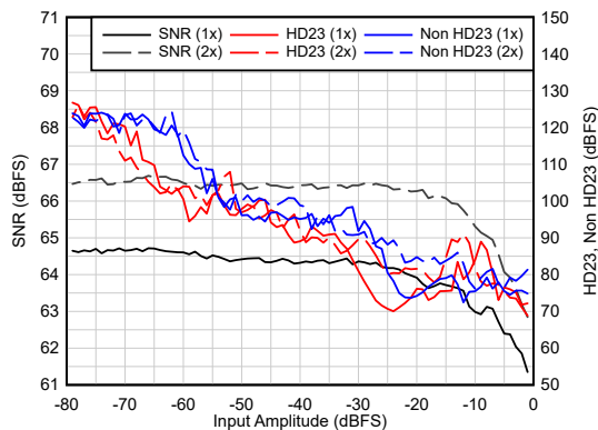
图 5-25. Dither Spur vs A_{IN} F_{IN} = 900 MHz,
