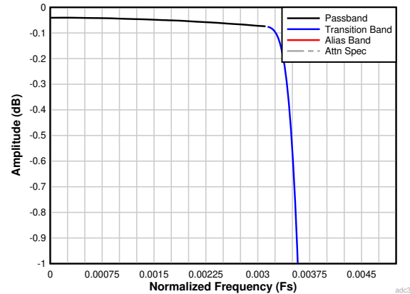
图 6-37. Decimation by 128 Passband Ripple Response
