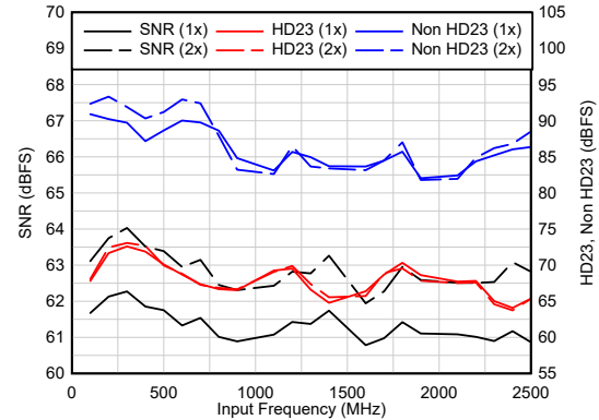
图 5-24. AC Performance vs F_{IN} A_{IN} = -4 dBFS, Dither = EN
