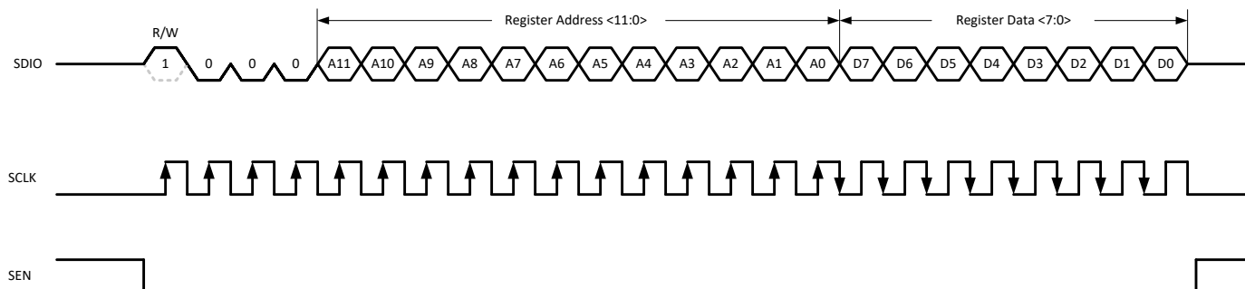
图 6-47. Serial Register Read Timing Diagram
