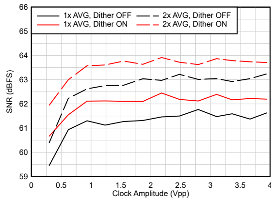
图 7-9. SNR vs Clock Amplitude ( F_{IN} = 900 MHz)
