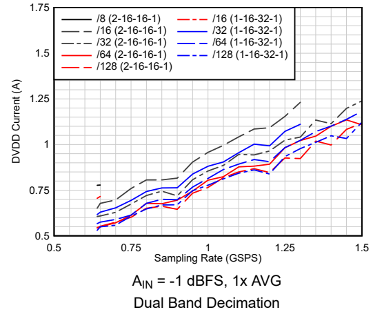
图 6-50. Current vs Sampling Rate vs Complex Decimation
