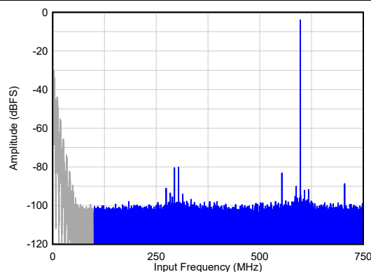
图 6-4. Single Tone FFT at F_{IN} = 600\text{ MHz}
