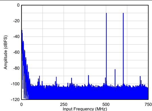
图 6-20. Two Tone FFT at F_{IN} = 900, 1000 MHz
