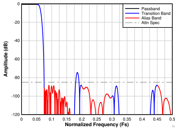
图 7-23. Complex Decimation by 8 Filter Response
