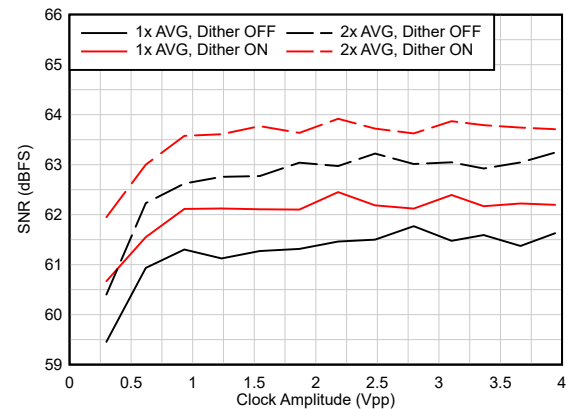
图 7-10. SNR vs Clock Amplitude ( F_{IN} = 1800 MHz)
