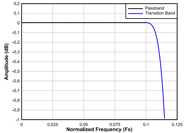
图 7-22. Decimation by 4 Passband Ripple Response
