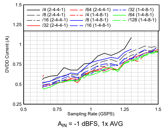
图 6-46. Current vs Sampling Rate vs Real Decimation
