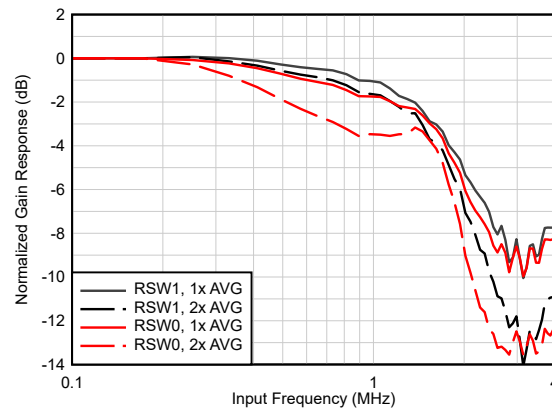
图 7-2. Full power input bandwidth (100 \Omega )
