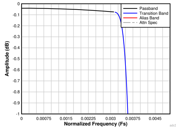
图 7-34. Decimation by 128 Passband Ripple Response
