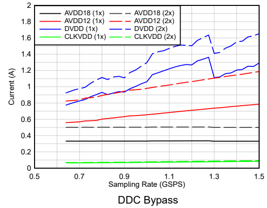
图 6-44. Current vs Sampling Rate vs Averaging
