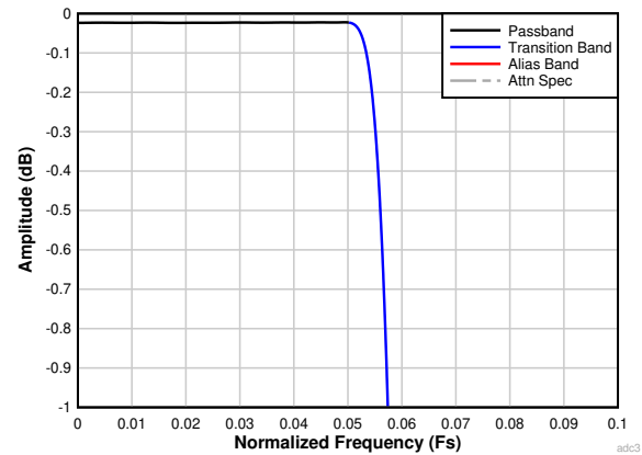
图 7-24. Decimation by 8 Passband Ripple Response
