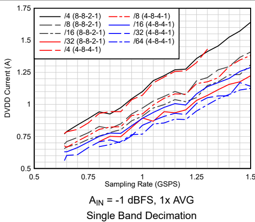
图 6-47. Current vs Sampling Rate vs Complex Decimation
