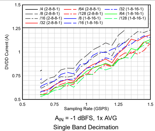
图 6-48. Current vs Sampling Rate vs Complex Decimation
