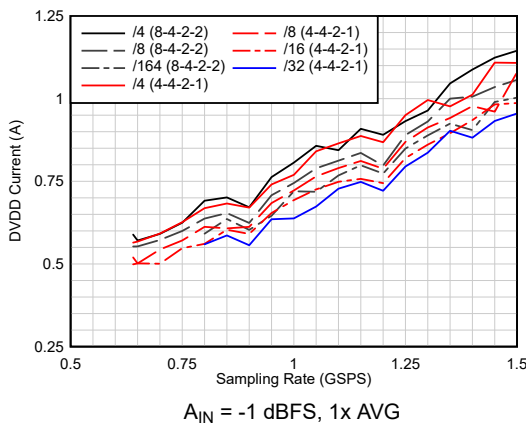
图 6-45. Current vs Sampling Rate vs Real Decimation
