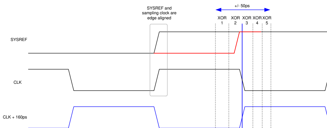
图 7-17. Detection of SYSREF Transition Within Capture Window
