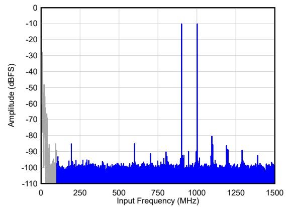
IMD3 = 70 dBc A_{IN} = -10 dBFS/tone, 1x AVG, Dither = EN 图 6-79. Two Tone FFT at F_{IN} = 900/1000 MHz
