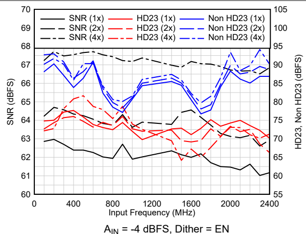
图 6-28. AC Performance vs F_{IN}
