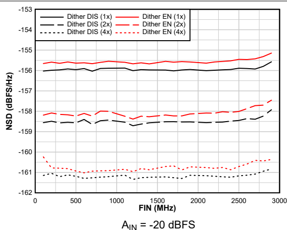
图 6-85. NSD Performance vs F_{IN}
