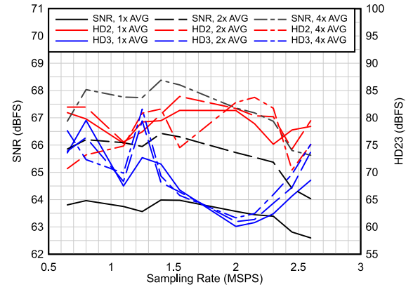
图 6-36. AC Performance vs F_s
