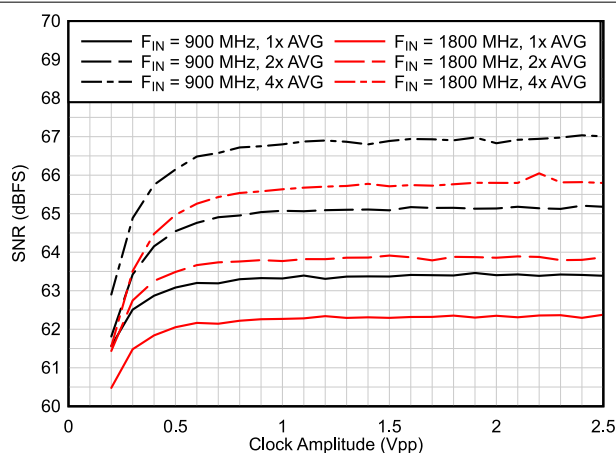
图 8-3. SNR vs Clock Amplitude (dither off)
