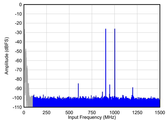
IMD3 = 71 dBc A_{IN} = -26 dBFS/tone, 1x AVG, Dither = EN 图 6-81. Two Tone FFT at F_{IN} = 900/1000 MHz
