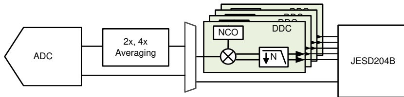
图 7-20. Digital Decimation Filter Options
