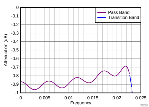
Figure 91. Divide-by-18 Filter Response (Zoomed)
