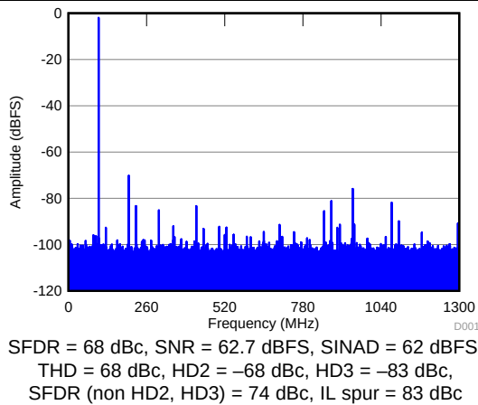
Figure 3. FFT for 100-MHz Input Signal
