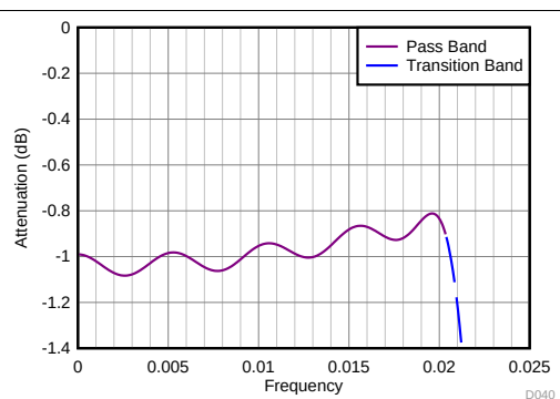
Figure 93. Divide-by-20 Filter Response (Zoomed)
