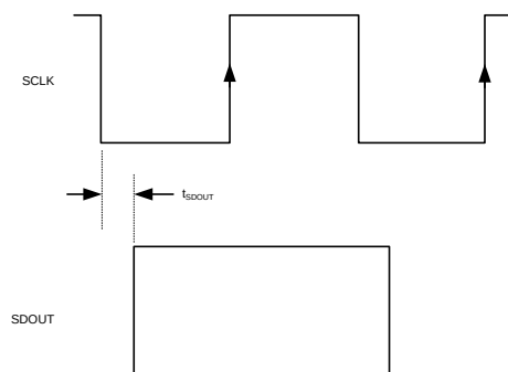
Figure 81. SDOUT Timing
