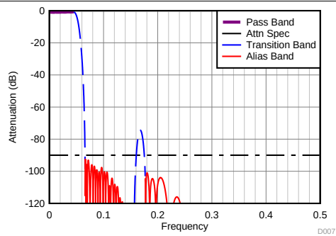
Figure 57. Filter Response Decimate-by-9
