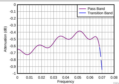
Figure 54. Filter Response Decimate-by-6 (Zoomed)
