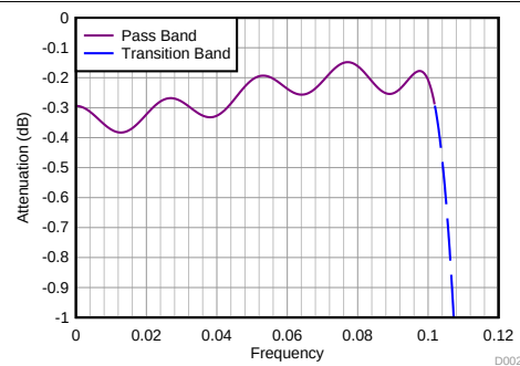
Figure 52. Filter Response Decimate-by-4 (Zoomed)
