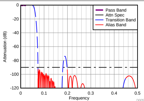
Figure 55. Filter Response Decimate-by-8
