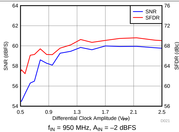
Figure 23. Performance vs Clock Amplitude
