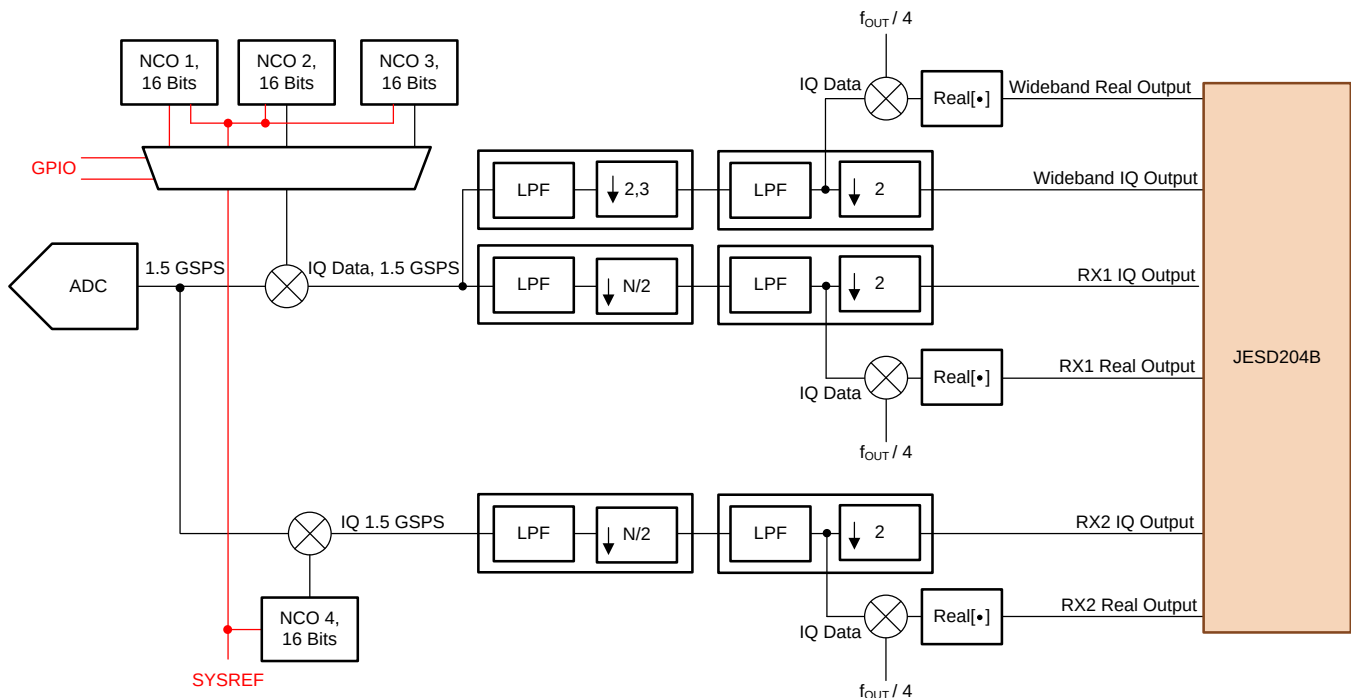
Figure 46. DDC Chains Overview (One ADC Channel Shown)
