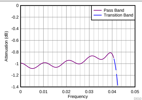
Figure 60. Filter Response Decimate-by-10 (Zoomed)
