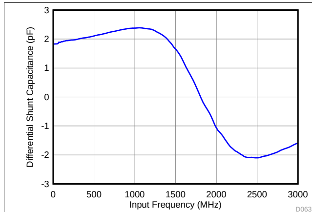
Figure 35. Differential Input Capacitance vs Input Frequency
