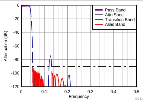
Figure 61. Filter Response Decimate-by-12
