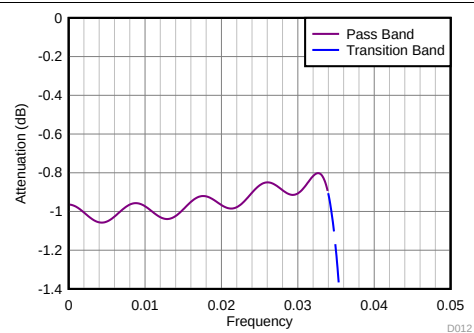
Figure 62. Filter Response Decimate-by-12 (Zoomed)
