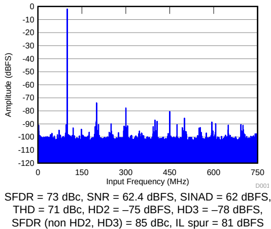
Figure 3. FFT for 100-MHz Input Signal
