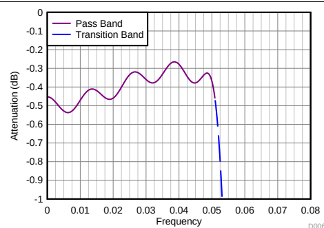
Figure 56. Filter Response Decimate-by-8 (Zoomed)
