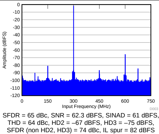
Figure 5. FFT for 300-MHz Input Signal
