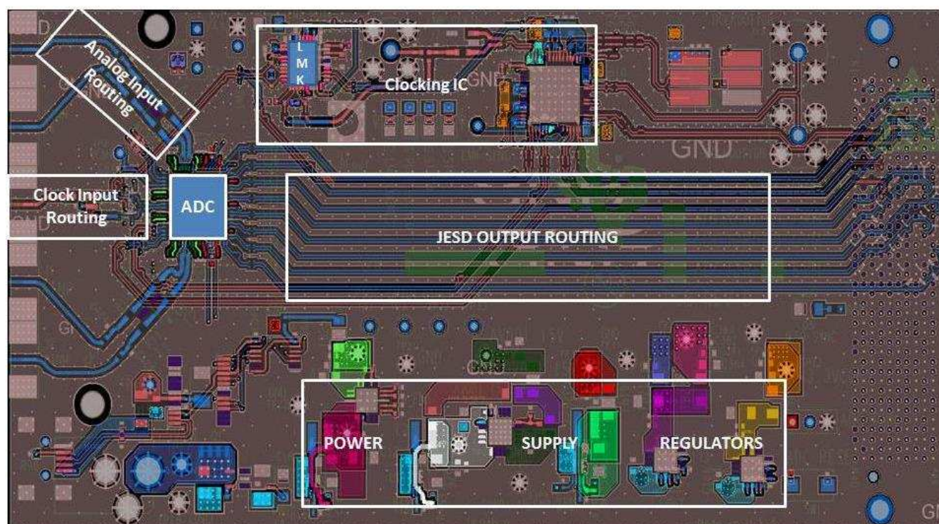
Figure 212. ADC32RF42EVM Layout
