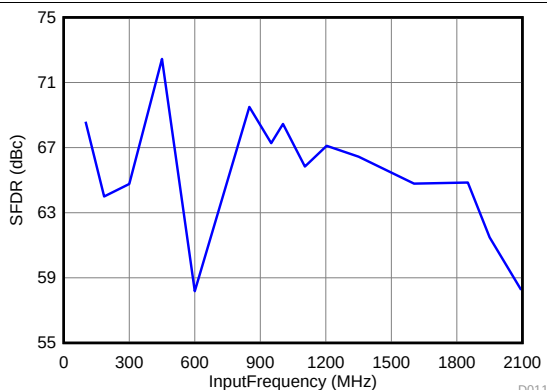
Figure 13. Spurious-Free Dynamic Range vs Input Frequency
