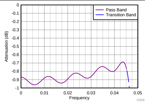
Figure 58. Filter Response Decimate-by-9 (Zoomed)
