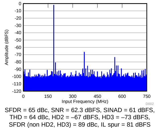
Figure 4. FFT for 185-MHz Input Signal
