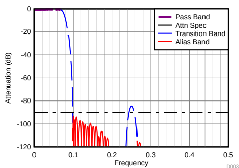
Figure 53. Filter Response Decimate-by-6
