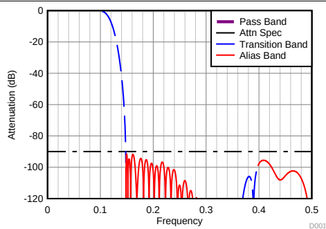
Figure 51. Filter Response Decimate-by-4
