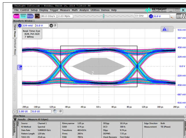
Figure 68. Data Eye at 5 Gbps
