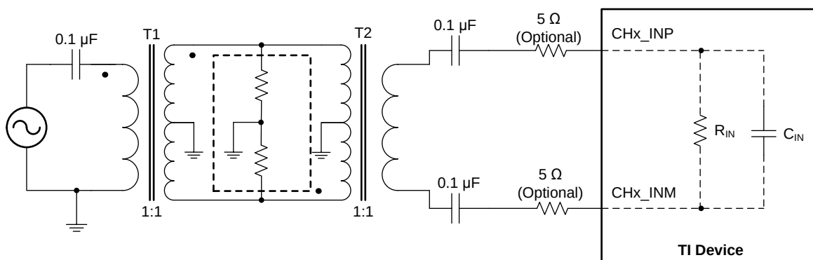
Figure 208. Input Drive Circuit
