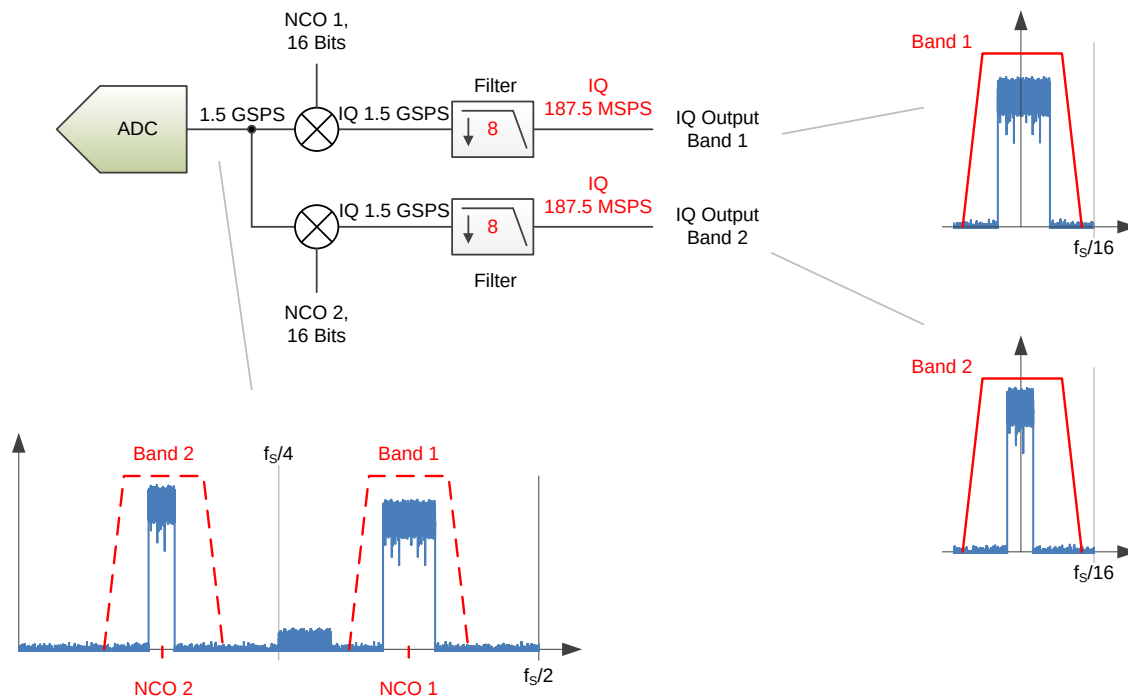
Figure 49. Dual-Band Example
