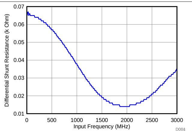
Figure 36. Differential Input Resistance vs Input Frequency
