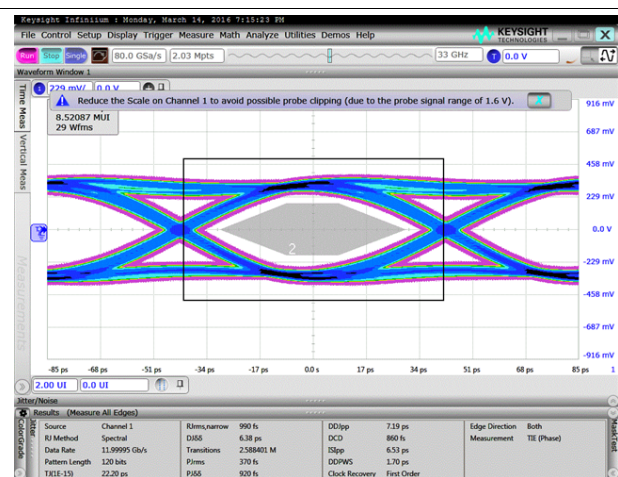
Figure 69. Data Eye at 12 Gbps
