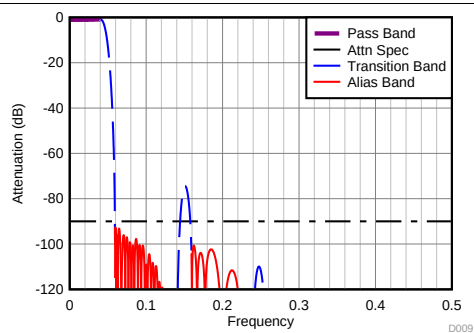
Figure 59. Filter Response Decimate-by-10
