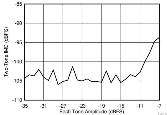
图 6-75. Intermodulation Distortion vs Input Amplitude (46 MHz and 50 MHz)
