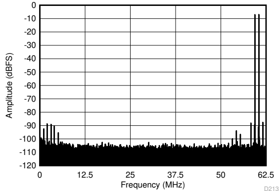
f_{IN1} = 185\text{ MHz} , f_{IN2} = 190\text{ MHz} , \text{IMD3} = 87.5\text{ dBFS} , each tone at -7 dBFS
