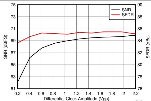
图 6-57. Performance vs Differential Clock Amplitude (40 MHz)
