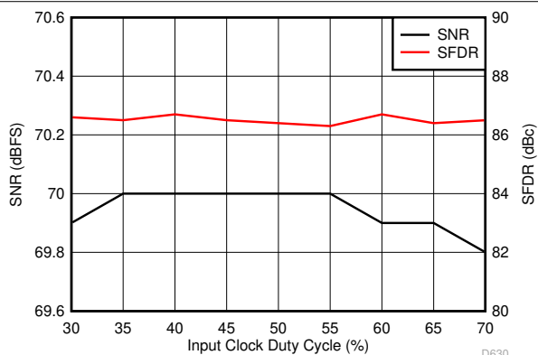
图 6-60. Performance vs Clock Duty Cycle (150 MHz)
