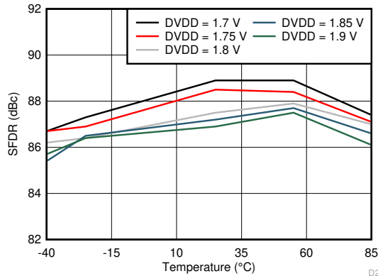
图 6-115. Spurious-Free Dynamic Range vs DVDD Supply and Temperature (170 MHz)
