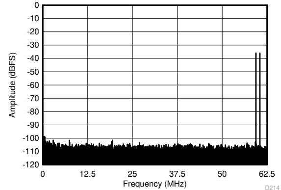
f_{IN1} = 185\text{ MHz} , f_{IN2} = 190\text{ MHz} , \text{IMD3} = 96.5\text{ dBFS} , each tone at -36 dBFS
