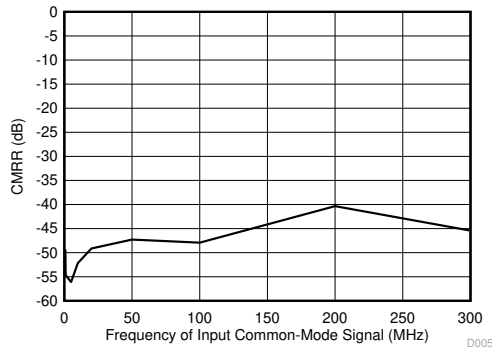
图 6-121. Common-Mode Rejection Ratio vs Common-Mode Signal Frequency
