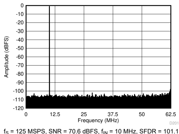
图 9-4. Performance FFT at 10 MHz (Low Input Frequency)
