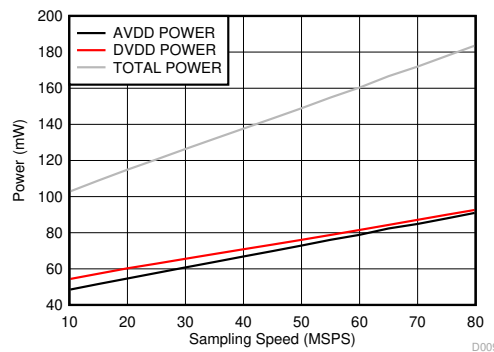
图 6-125. Power vs Sampling Speed (One-Wire Mode)
