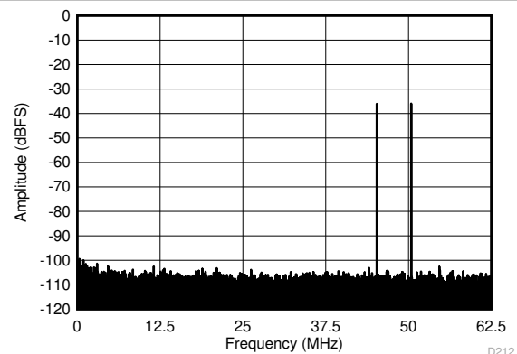
图 6-100. FFT for 450-MHz Input Signal (Dither Off)
