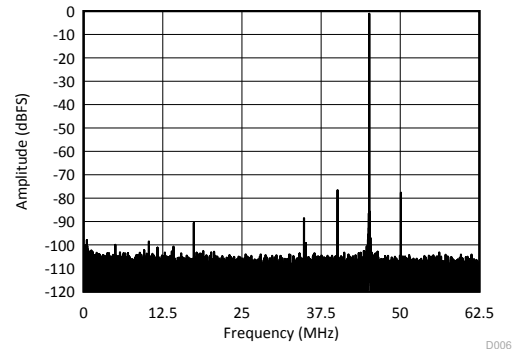
图 6-122. Common-Mode Rejection Ratio Spectrum
