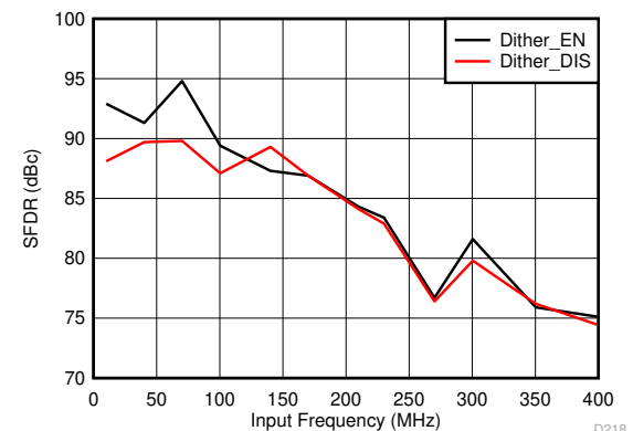
图 6-108. Spurious-Free Dynamic Range vs Input Frequency
