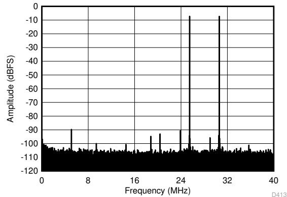
f_{IN1} = 185\text{ MHz} , f_{IN2} = 190\text{ MHz} , \text{IMD3} = 89\text{ dBFS} , each tone at -7 dBFS
