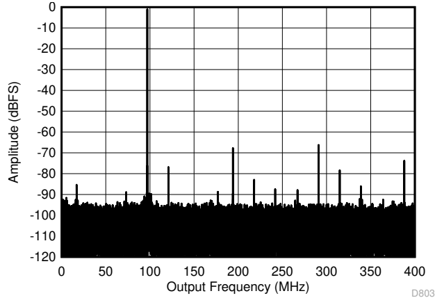
图 5-7. Single Tone FFT at 897 MHz and -1dBFS
