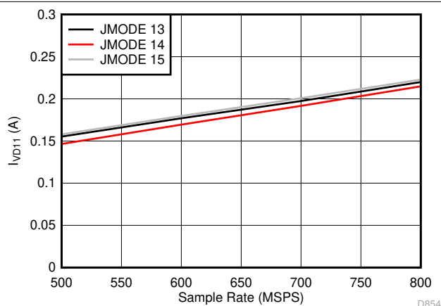
图 5-97. Dual Channel, I_{VD11} vs F_S for JMODES 13 - 15
