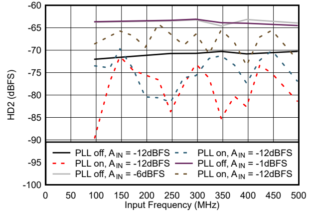
图 5-50. HD2 vs Input Frequency in Low Power Mode
