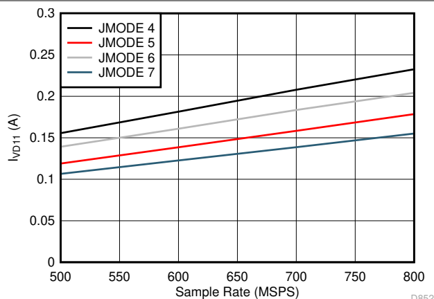
图 5-95. Dual Channel, I_{VD11} vs F_S for JMODES 4 - 7
