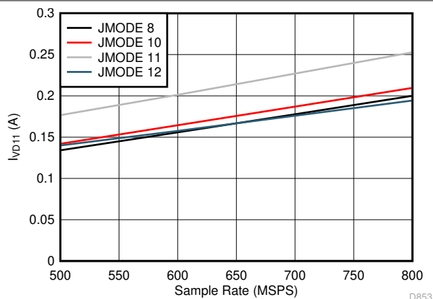
图 5-96. Dual Channel, I_{VD11} vs F_S for JMODES 8 - 12
