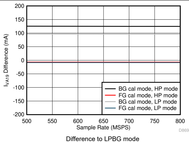
图 5-99. Dual Channel, I_{VA19} vs F_S over Modes
