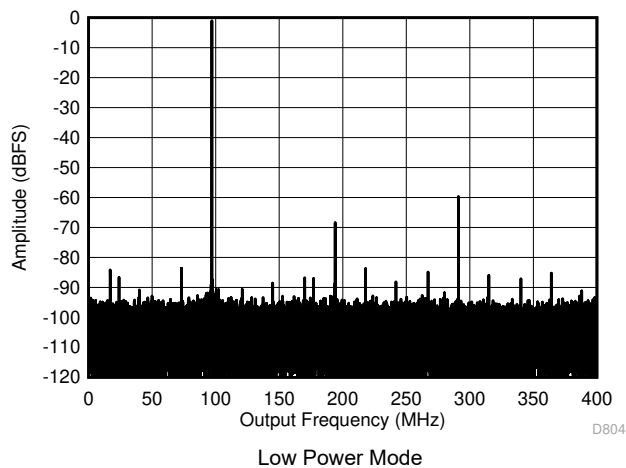
图 5-11. Single Tone FFT at 897 MHz and -1dBFS
