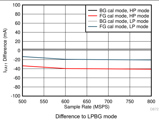
图 5-100. Dual Channel, I_{VA11} vs F_S over Modes
