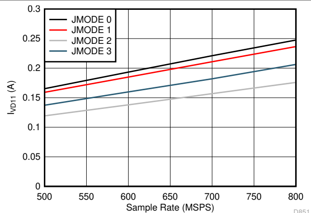
图 5-94. Dual Channel, I_{VD11} vs F_S for JMODES 0 - 3
