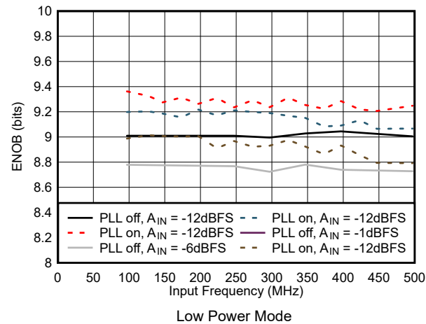
图 5-53. ENOB vs Input Frequency in Low Power Mode
