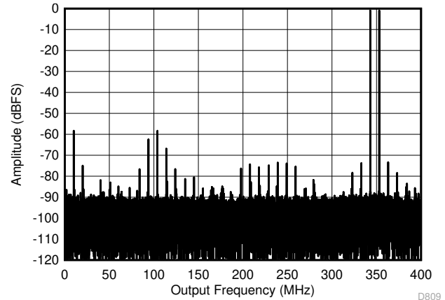
图 5-66. Two Tone FFT at 347 MHz
