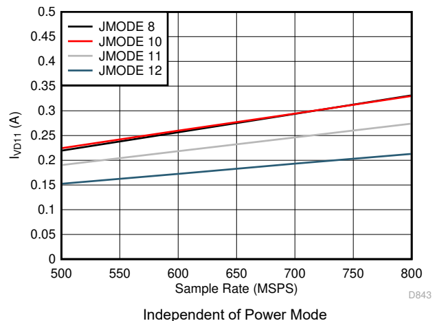
图 5-82. Quad Channel, I_{VD11} vs F_S for JMODES 8-12
