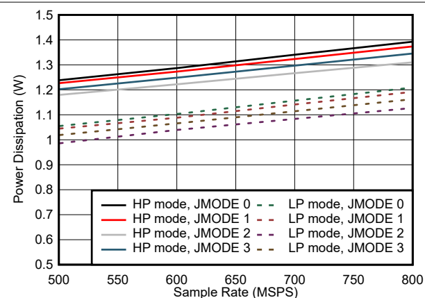
图 5-88. Dual Channel, Power Dissipation vs F_S for JMODES 0 - 3
