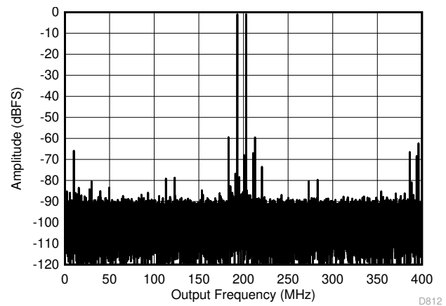
图 5-68. Two Tone FFT at 3498 MHz
