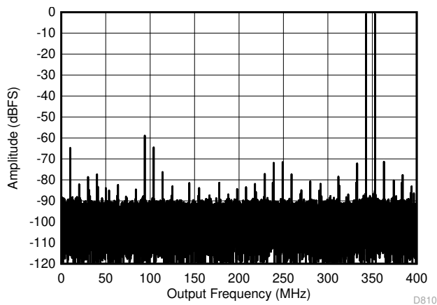
图 5-67. Two Tone FFT at 1798 MHz
