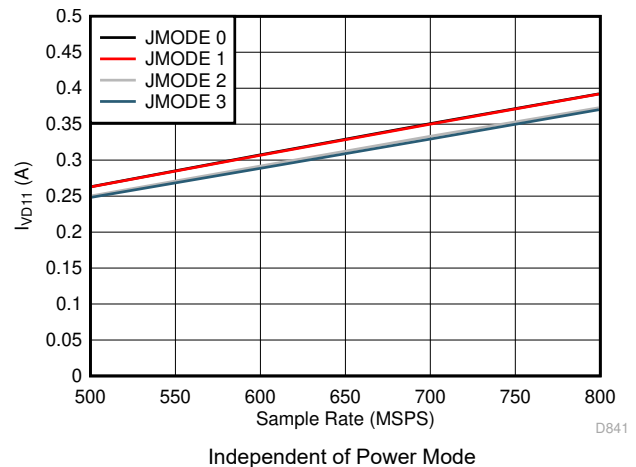
图 5-80. Quad Channel, I_{VD11} vs F_S for JMODES 0 - 3
