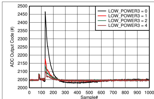
图 6-12. Background Calibration Core Transition In Low Power Mode
