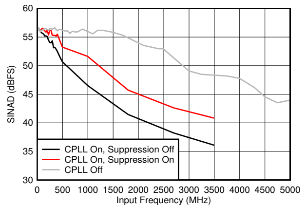
图 5-42. SINAD vs F IN and C-PLL modes
