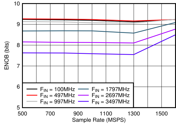
图 5-26. ENOB vs Sample Rate
