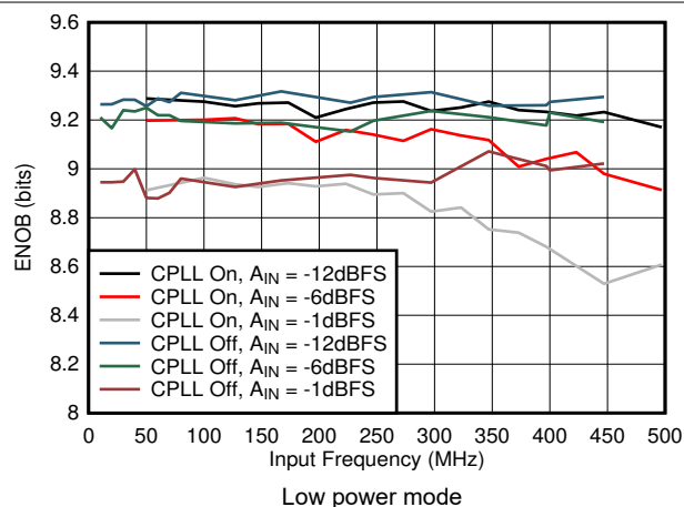
图 5-57. ENOB vs A_{IN} and C-PLL
