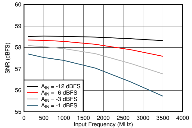
图 5-18. SNR vs Input Frequency
