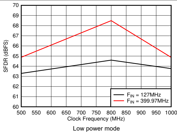
图 5-29. SFDR vs Sample Rate
