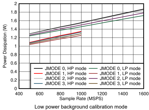
图 5-89. Dual Channel, Power Dissipation vs F_S and JMODE 0 - 3
