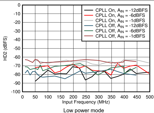
图 5-58. HD2 vs A_{IN} and C-PLL
