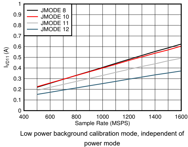
图 5-87. Quad Channel, I_{VD11} vs F_S and JMODE 8 - 12
