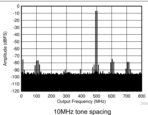
图 5-69. Two Tone FFT at 498MHz
