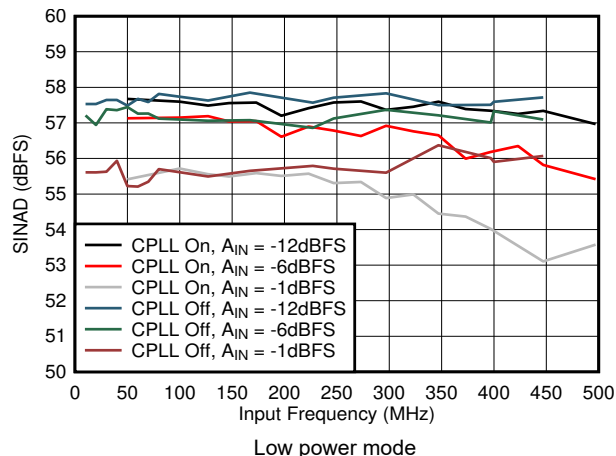
图 5-56. SINAD vs A_{IN} and C-PLL
