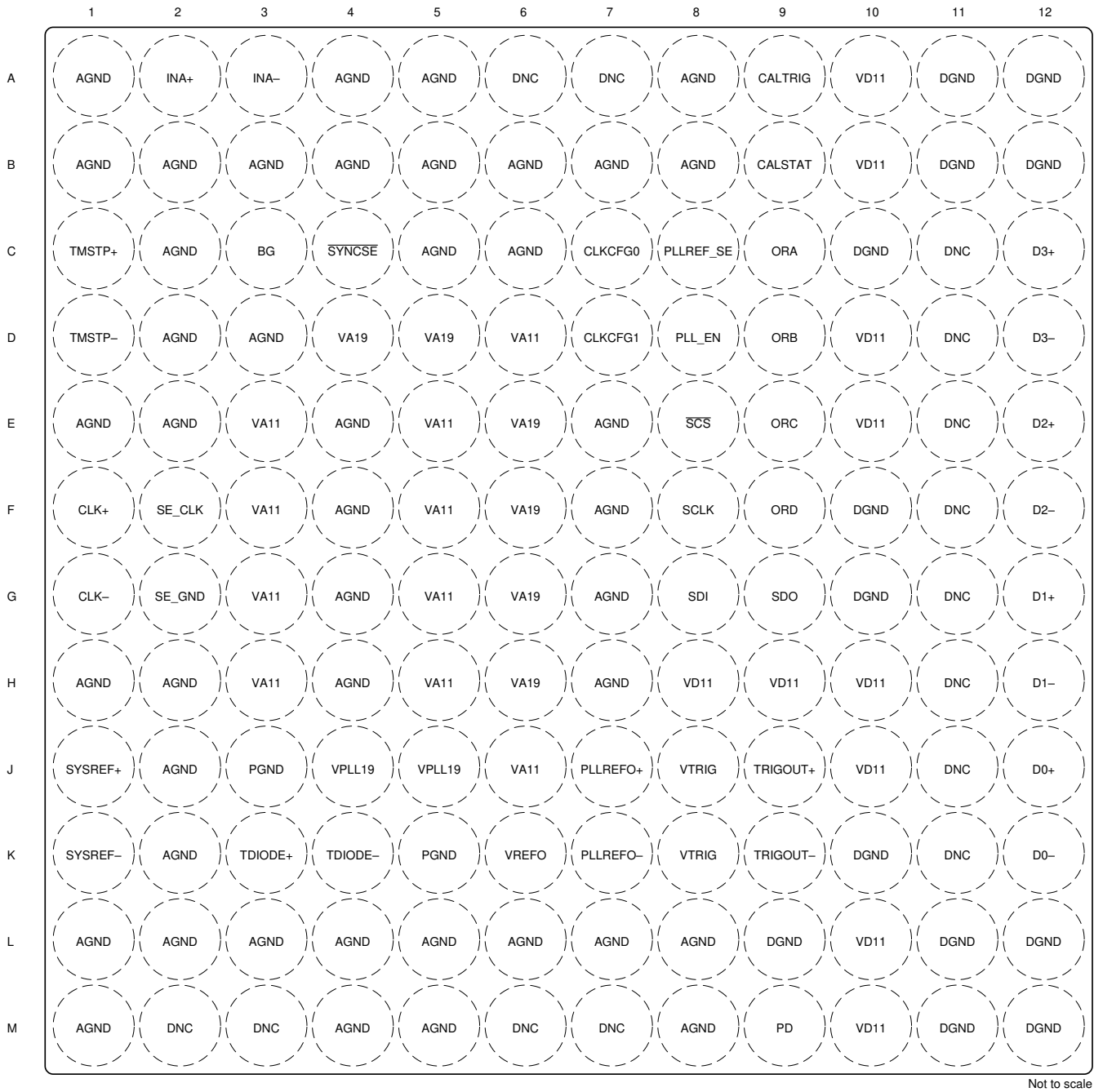
图 4-3. Single Channel AAV Package, 144-Ball Flip Chip BGA (Top View)
