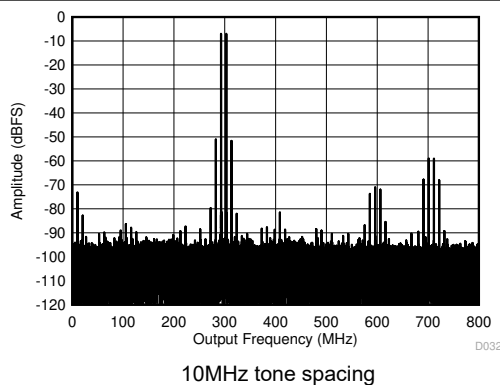
图 5-71. Two Tone FFT at 3498MHz
