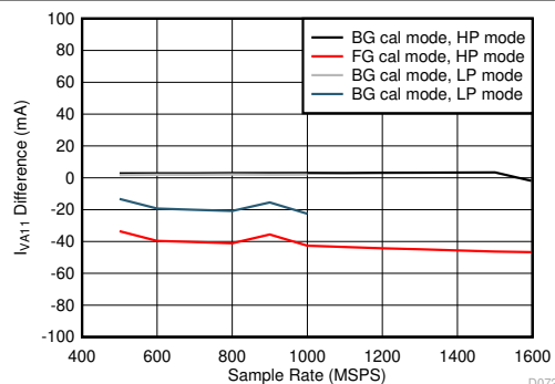
图 5-116. Dual Channel, I_{VA11} Change with Calibration Mode
