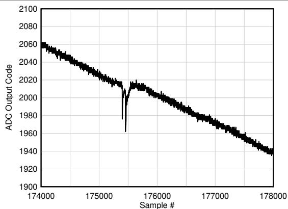
图 5-127. Background Calibration Core Transition (AC Signal Zoomed)
