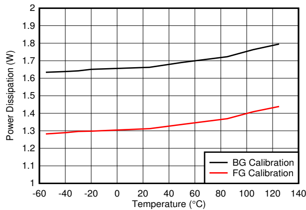
图 5-123. Single Channel, Power Dissipation vs Temperature
