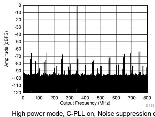
图 5-6. Single Tone FFT at 347MHz and -1dBFS
