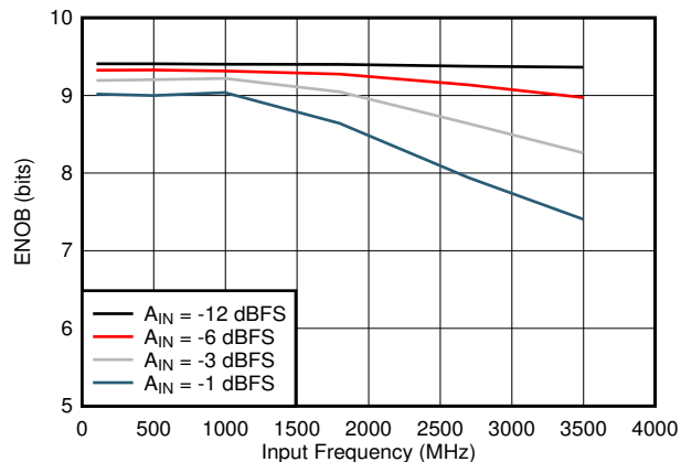
图 5-20. ENOB vs Input Frequency
