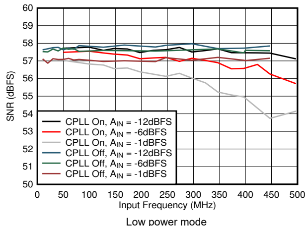
图 5-55. SNR vs A_{IN} and C-PLL
