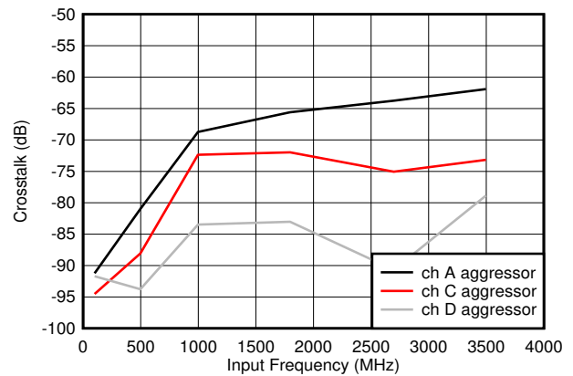
图 5-78. Crosstalk to Channel B vs F_{IN}
