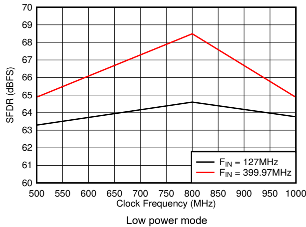
图 5-27. SFDR vs Sample Rate
