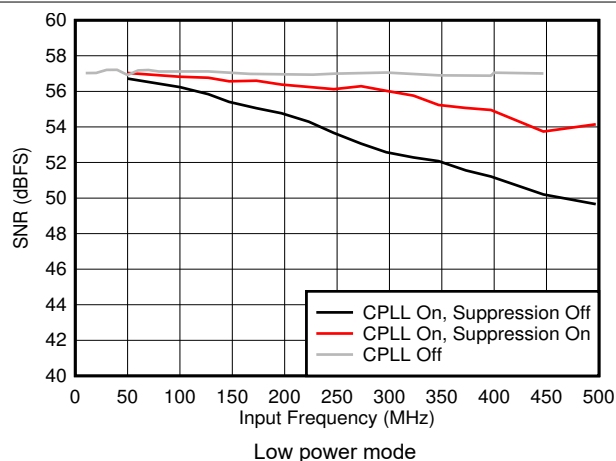
图 5-45. SNR vs F_{IN} and C-PLL modes
