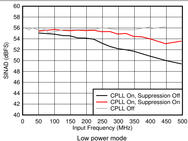
图 5-46. SINAD vs F_{IN} and C-PLL modes
