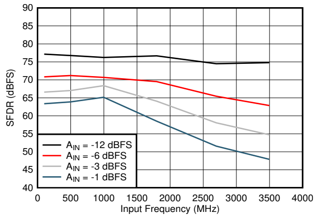
图 5-17. SFDR vs Input Frequency
