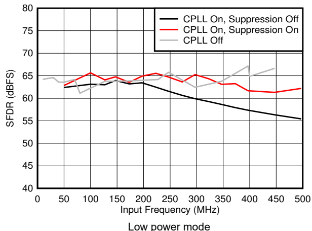
图 5-44. SFDR vs F_{IN} and C-PLL modes
