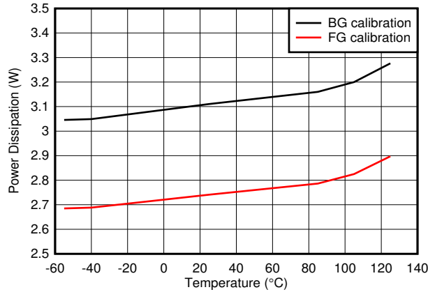
图 5-121. Quad Channel, Power Dissipation vs Temperature
