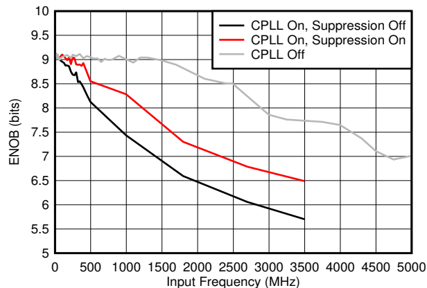
图 5-43. ENOB vs F_{IN} and C-PLL modes
