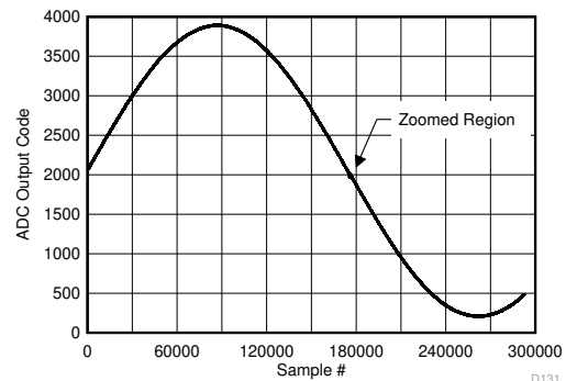
图 5-124. Background Calibration Core Transition (midscale voltage)
