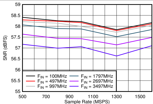
图 5-24. SNR vs Sample Rate
