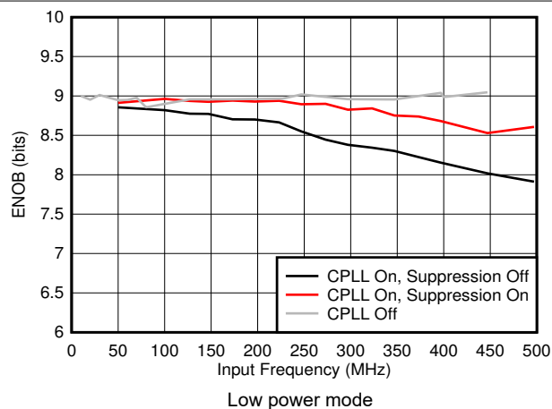
图 5-47. ENOB vs F_{IN} and C-PLL modes
