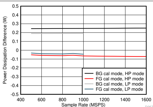
图 5-109. Quad Channel, Power Dissipation Change with Calibration Mode
