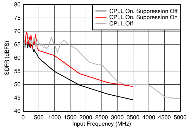
图 5-40. SFDR vs F IN and C-PLL modes
