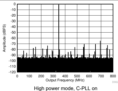
图 5-5. Single Tone FFT at 347MHz and -1dBFS
