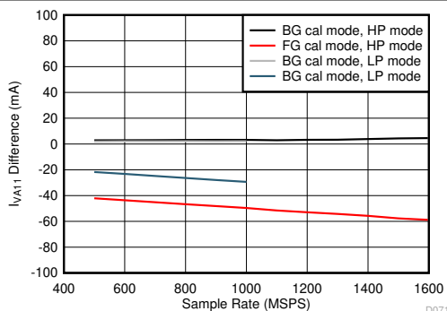
图 5-115. Quad Channel, I_{VA11} Change with Calibration Mode
