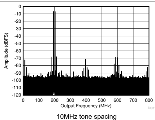
图 5-70. Two Tone FFT at 1798MHz
