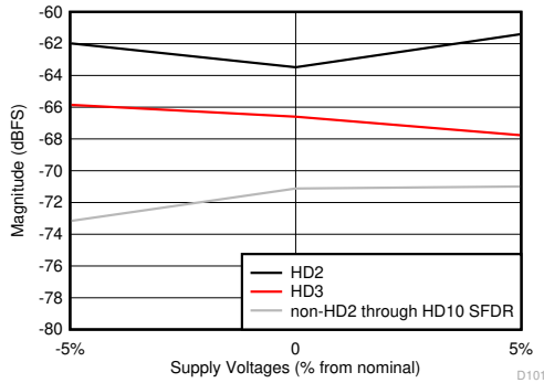
图 5-61. HD2, HD3 and Worst non-HD Spur vs Supply Voltage
