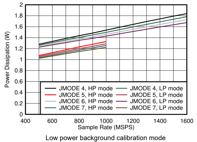
图 5-90. Dual Channel, Power Dissipation vs F_S and JMODE 4 - 7
