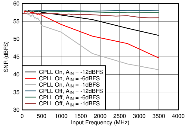
图 5-49. SNR vs A_{IN} and C-PLL
