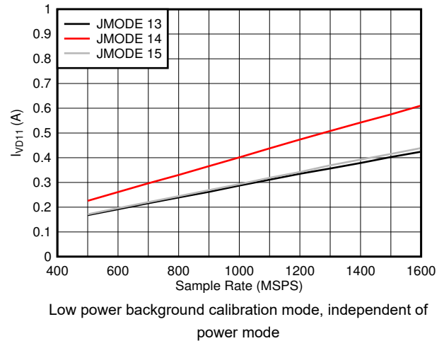
图 5-88. Quad Channel, I_{VD11} vs F_S and JMODE 13 - 15
