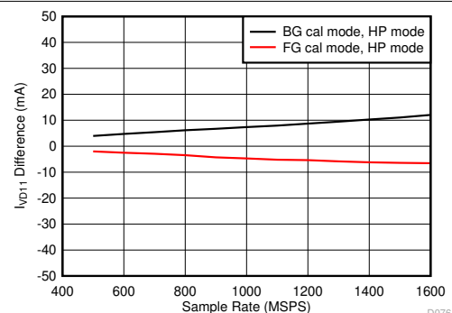
图 5-118. Quad Channel, I_{VD11} Change with Calibration Mode
