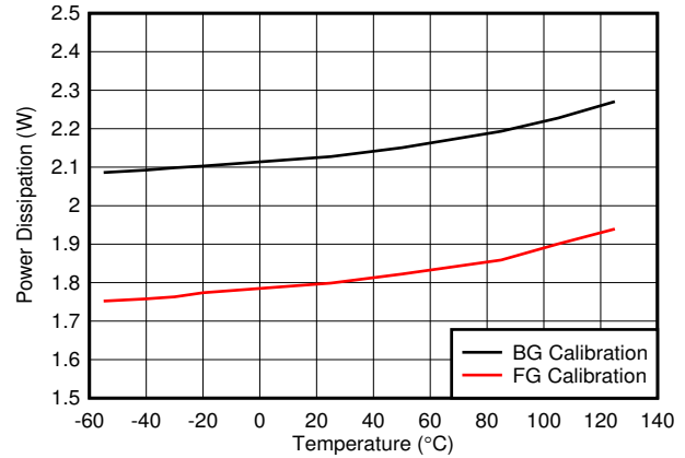
图 5-122. Dual Channel, Power Dissipation vs Temperature
