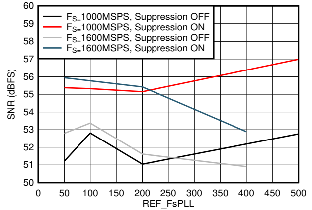
图 5-38. SNR vs F REF and Suppression
