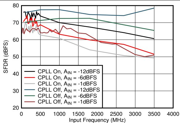
图 5-48. SFDR vs A_{IN} and C-PLL
