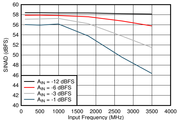
图 5-19. SINAD vs Input Frequency
