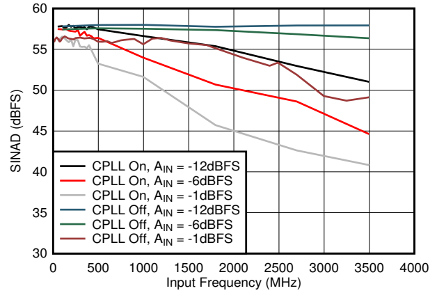
图 5-50. SINAD vs A_{IN} and C-PLL
