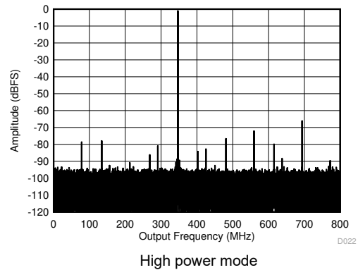
图 5-4. Single Tone FFT at 347MHz and -1dBFS
