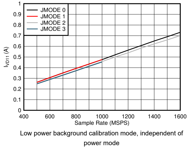
图 5-85. Quad Channel, I_{VD11} vs F_S and JMODE 0 - 3
