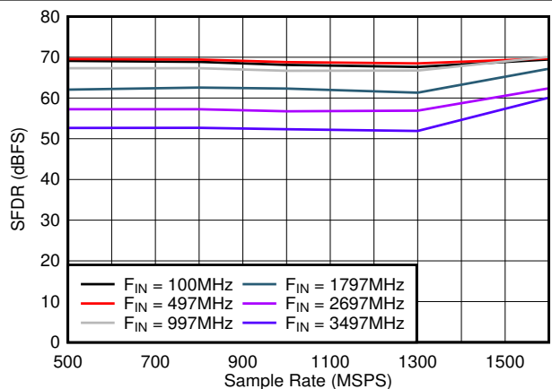
图 5-23. SFDR vs Sample Rate
