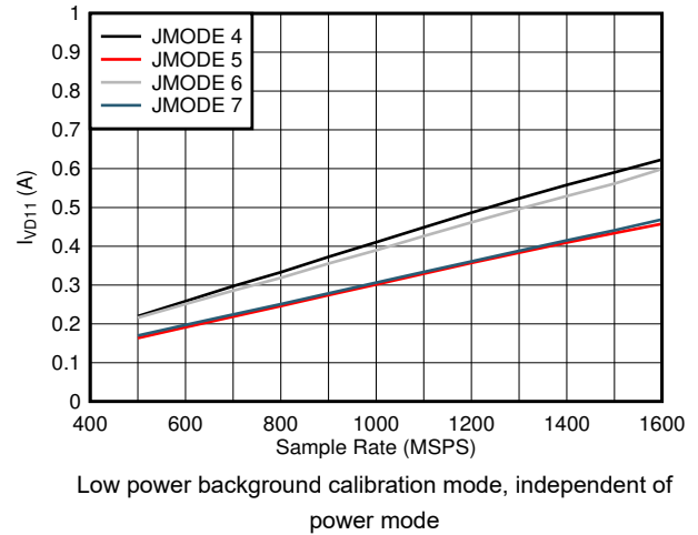
图 5-86. Quad Channel, I_{VD11} vs F_S and JMODE 4 - 7
