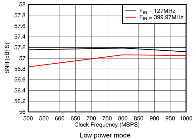
图 5-28. SNR vs Sample Rate
