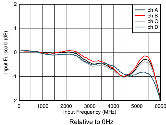
图 5-3. Input Fullscale vs Frequency
