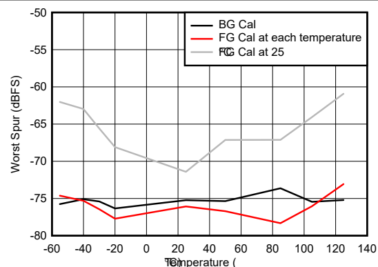
图 5-68. Worst Spur vs Temperature
