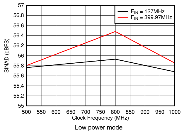
图 5-30. SINAD vs Sample Rate
