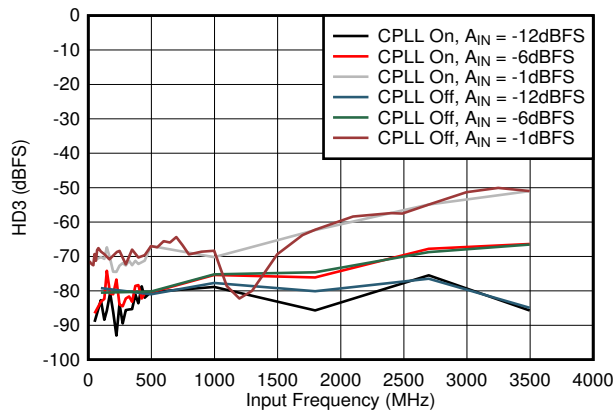
图 5-53. HD3 vs A_{IN} and C-PLL
