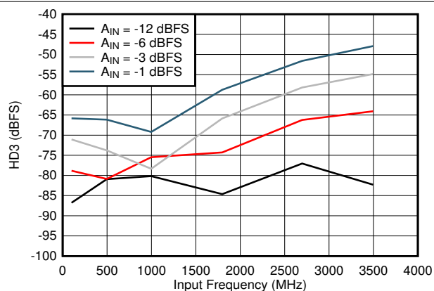
图 5-22. HD3 vs Input Frequency
