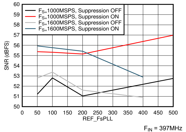
图 5-38. SNR vs F_{REF} and Suppression
