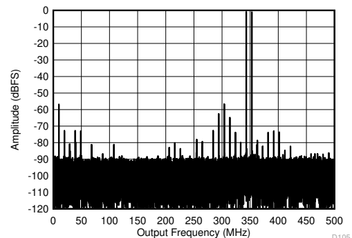
图 5-70. Two Tone FFT at 1798MHz
