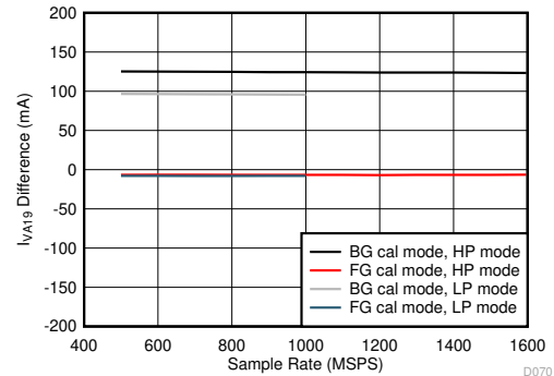
图 5-114. Single Channel, I_{VA19} Change with Calibration Mode
