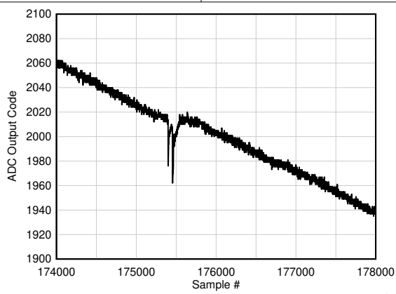
图 5-125. Background Calibration Core Transition (offset voltage)
