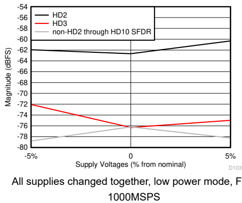
图 5-63. HD2, HD3 and Worst non-HD Spur vs Supply Voltage
