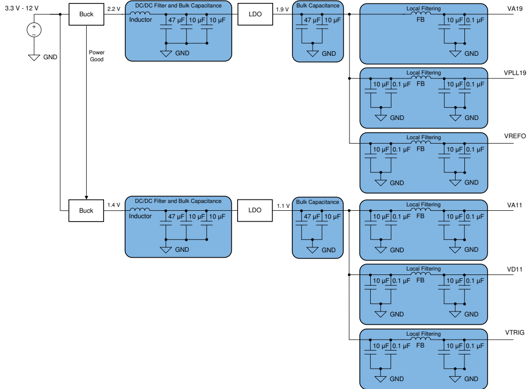
图 7-3. LDO Linear Regulator Approach Example
