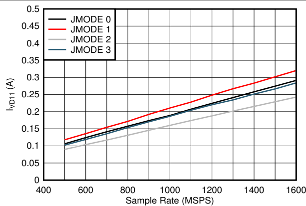
图 5-105. Single Channel, I_{VD11} vs F_S and JMODE 0 - 3
