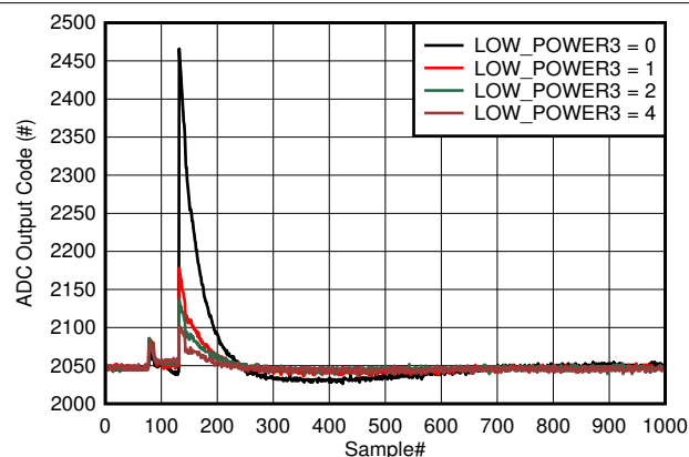
图 6-10. Background Calibration Core Transition In Low Power Mode
