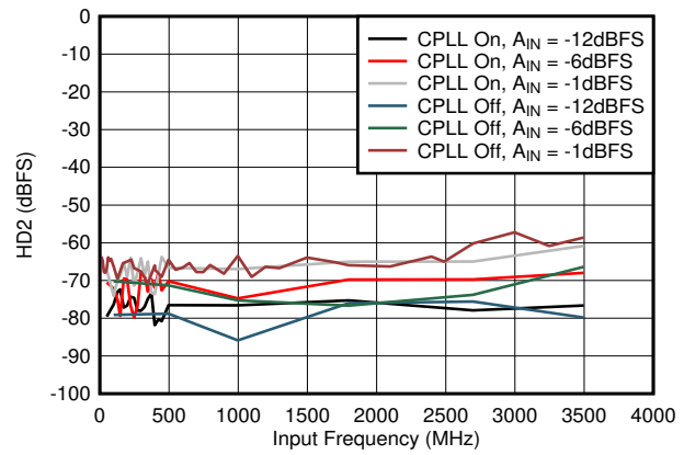
图 5-52. HD2 vs A_{IN} and C-PLL
