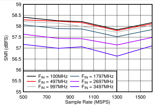
图 5-24. SNR vs Sample Rate
