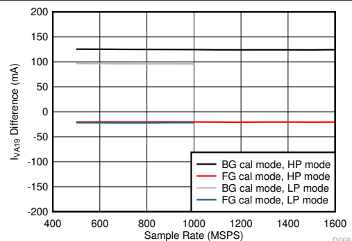
图 5-110. Dual Channel, Power Dissipation Change with Calibration Mode
