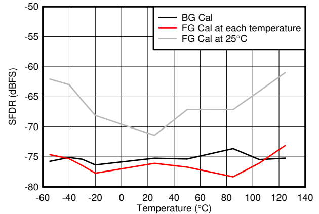
图 5-68. Worst Spur vs Temperature
