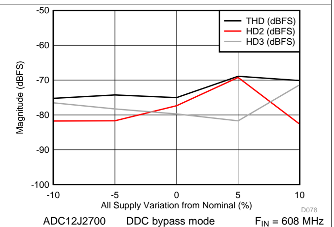
Figure 18. THD, H2, H3 vs Supply Voltage
