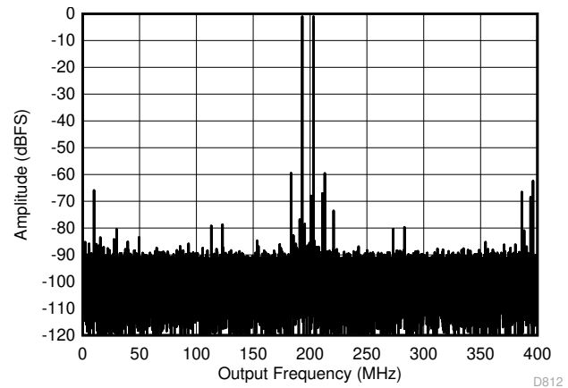
图 5-68. Two Tone FFT at 3498 MHz
