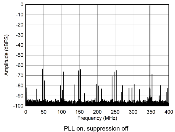
图 5-14. Single Tone FFT at 347 MHz and -1dBFS
