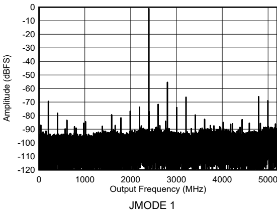
图 5-27. DES Mode: Single Tone Output Spectrum at 2397 MHz
