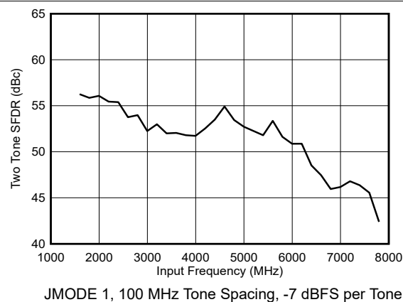
图 5-23. DES Mode: Two Tone SFDR vs Input Frequency
