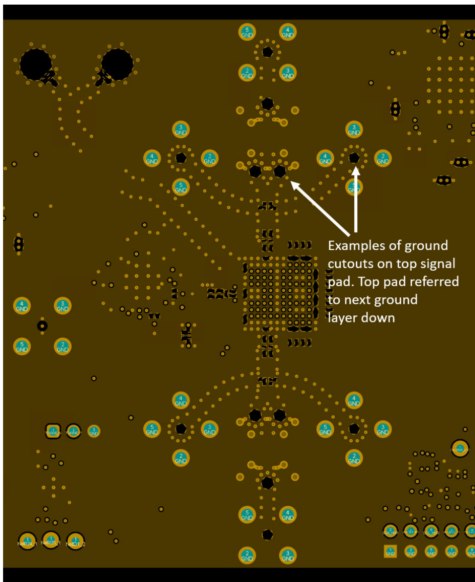
图 7-8. Example of Ground Cut-outs on Top Signal Pad
