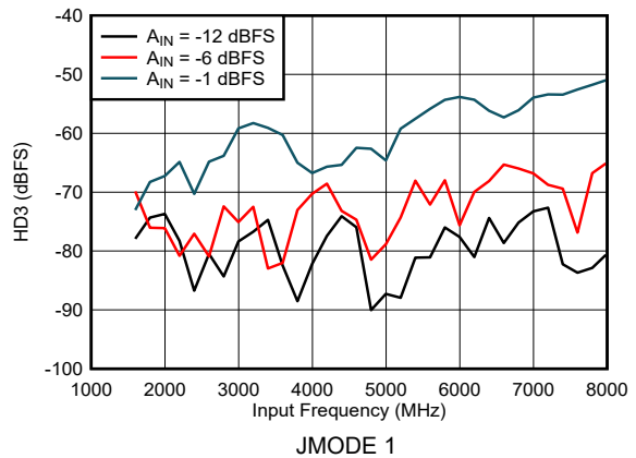
图 5-12. DES Mode: HD3 vs Input Frequency
