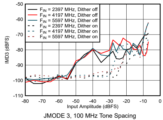
图 5-46. Dual Channel Mode: IMD3 vs Input Amplitude
