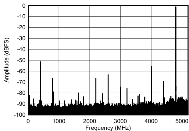
图 7-4. FFT for 5597 MHz Input Signal, 10.4 GSPS, JMODE1
