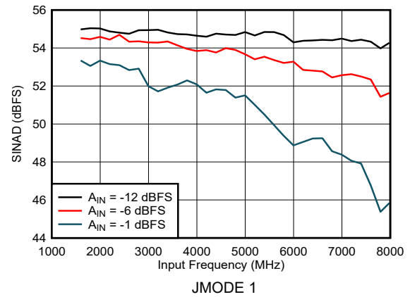
图 5-10. DES Mode: SINAD vs Input Frequency
