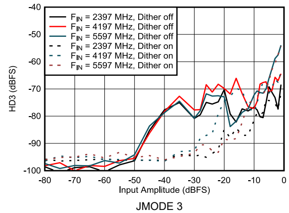
图 5-42. Dual Channel Mode: HD3 vs Input Amplitude
