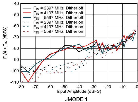
图 5-21. DES Mode: F_S/4 + F_{\text{IN}} vs Input Amplitude
