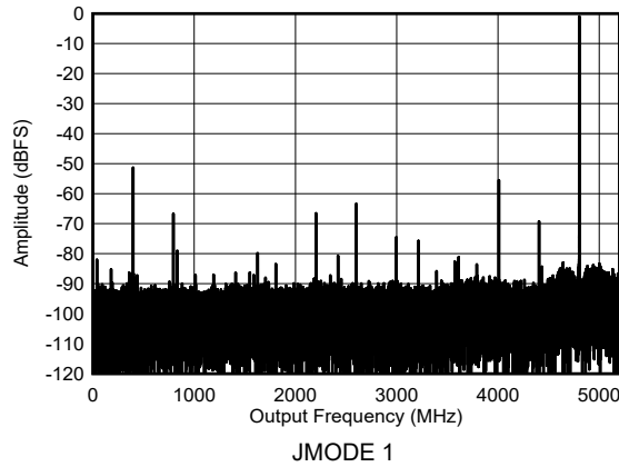
图 5-29. DES Mode: Single Tone Output Spectrum at 5597 MHz
