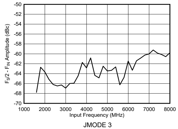
图 5-38. Dual Channel Mode: F_S/2 - F_{\text{IN}} vs Input Frequency
