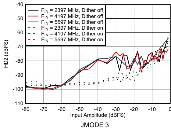
图 5-41. Dual Channel Mode: HD2 vs Input Amplitude
