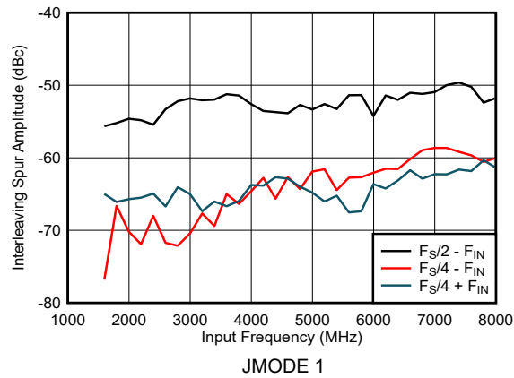
图 5-13. DES Mode: Interleaving Spurs vs Input Frequency
