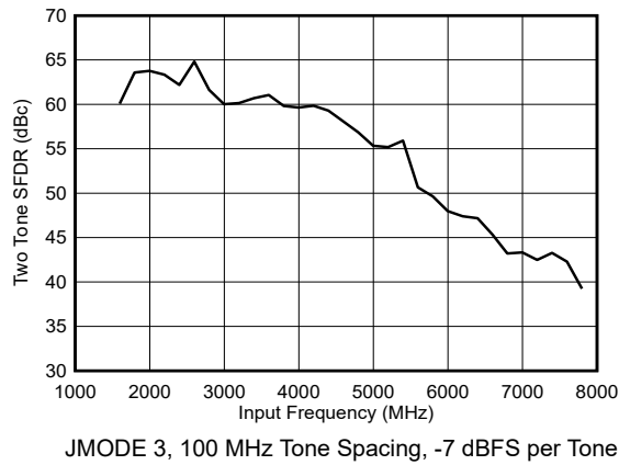
图 5-45. Dual Channel Mode: Two Tone SFDR vs Input Frequency
