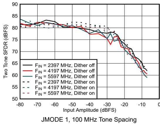
图 5-25. DES Mode: Two Tone SFDR vs Input Amplitude
