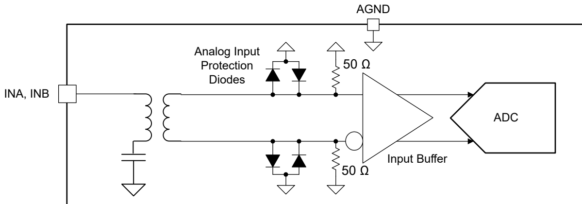
图 6-1. ADC12DJ5200SE Analog Input Internal Termination and Protection Diagram
