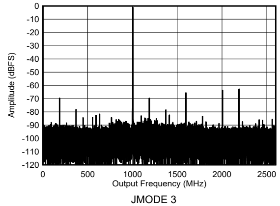
图 5-50. Dual Channel Mode: Single Tone Spectrum at 4197 MHz
