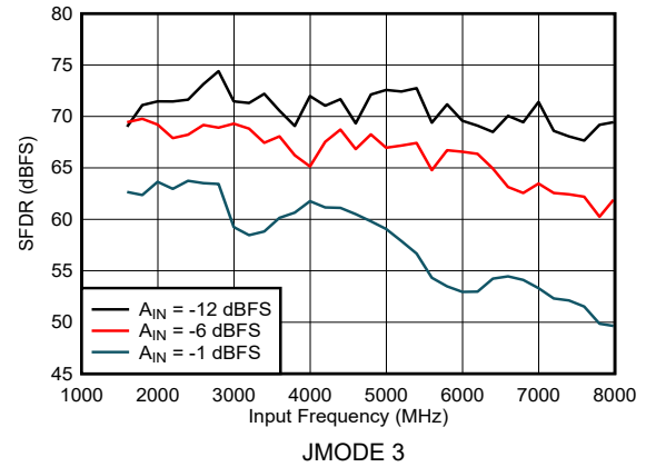
图 5-34. Dual Channel Mode: SFDR vs Input Frequency
