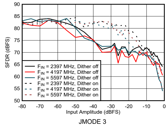
图 5-40. Dual Channel Mode: SFDR vs Input Amplitude
