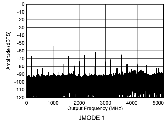
图 5-28. DES Mode: Single Tone Output Spectrum at 4197 MHz
