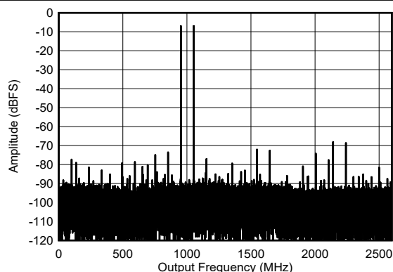
图 5-53. Dual Channel Mode: Dual Tone Spectrum at 4197 MHz
