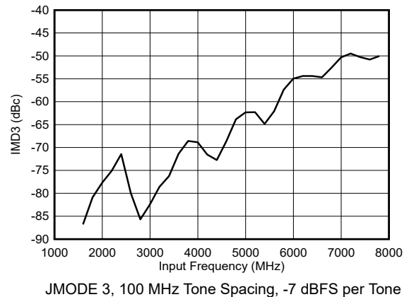
图 5-44. Dual Channel Mode: IMD3 vs Input Frequency
