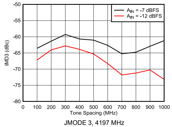
图 5-48. Dual Channel Mode: IMD3 vs Tone Spacing
