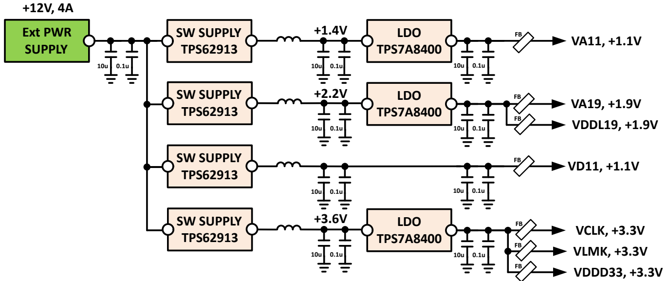
图 7-5. LDO Linear Regulator Approach Example
