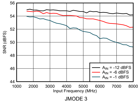
图 5-33. Dual Channel Mode: SNR vs Input Frequency
