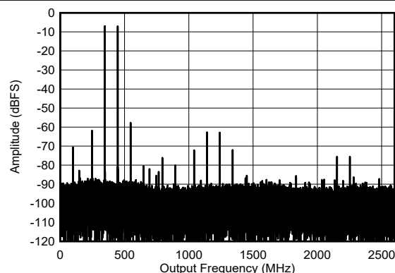
图 5-54. Dual Channel Mode: Dual Tone Spectrum at 5597 MHz
