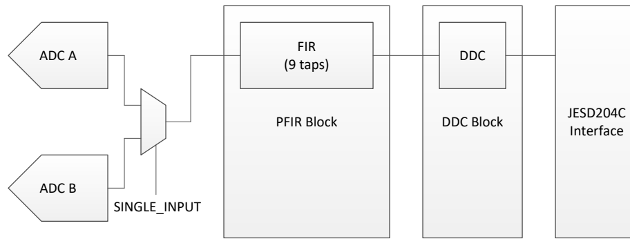
图 6-5. Single Channel Equalization PFIR Block Diagram
