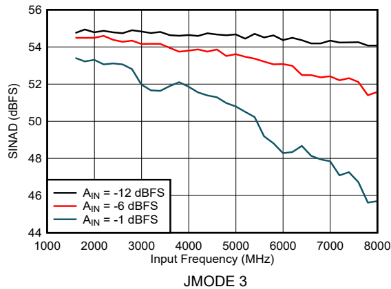
图 5-35. Dual Channel Mode: SINAD vs Input Frequency
