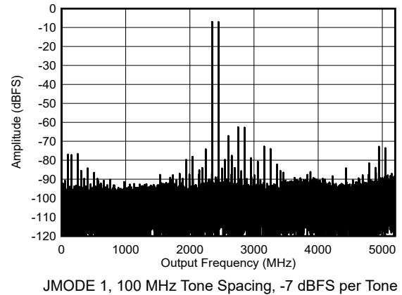
图 5-30. DES Mode: Two Tone Output Spectrum at 2397 MHz
