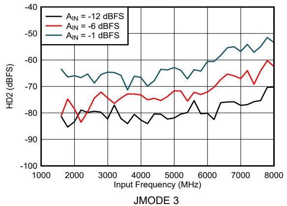
图 5-36. Dual Channel Mode: HD2 vs Input Frequency
