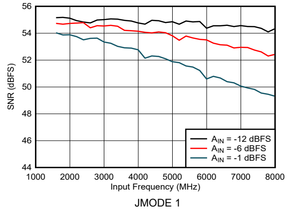
图 5-8. DES Mode: SNR vs Input Frequency
