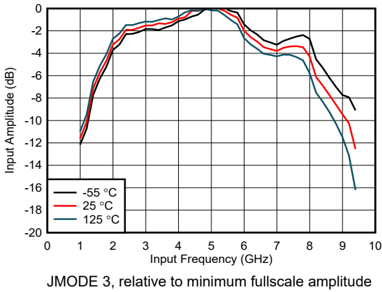
图 5-5. Dual Channel Mode: Input Amplitude vs Input Frequency
