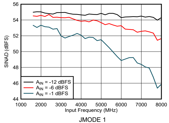
图 5-16. DES Mode: SINAD vs Input Amplitude
