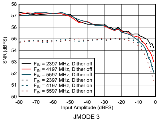
图 5-39. Dual Channel Mode: SNR vs Input Amplitude
