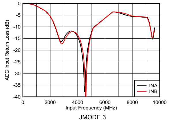
图 5-6. Dual Channel Mode: Input Return Loss vs Input Frequency
