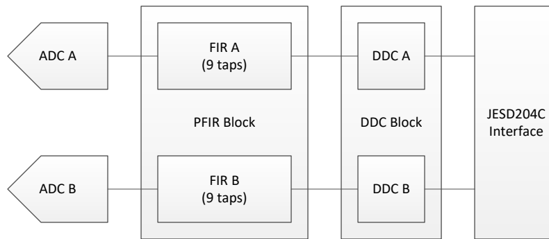
图 6-4. Dual Channel Equalization PFIR Block Diagram
