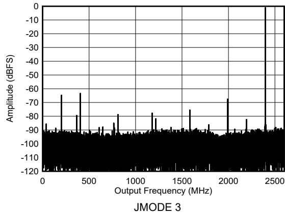
图 5-49. Dual Channel Mode: Single Tone Spectrum at 2397 MHz
