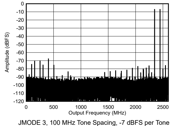
图 5-52. Dual Channel Mode: Dual Tone Spectrum at 2397 MHz
