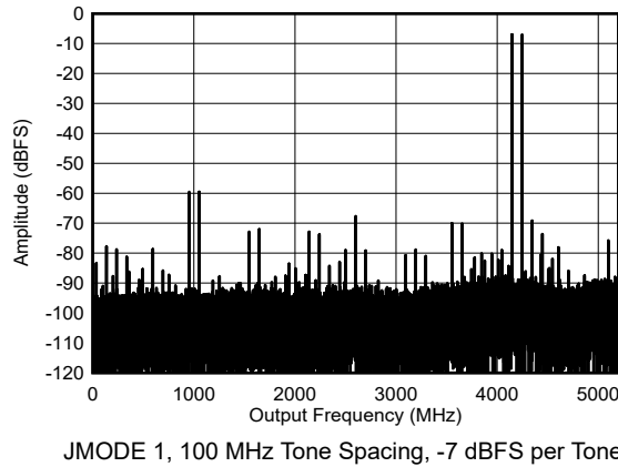
图 5-31. DES Mode: Two Tone Output Spectrum at 4197 MHz
