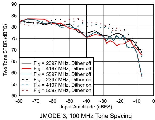
图 5-47. Dual Channel Mode: Two Tone SFDR vs Input Amplitude
