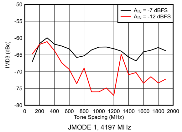
图 5-26. DES Mode: IMD3 vs Tone Spacing
