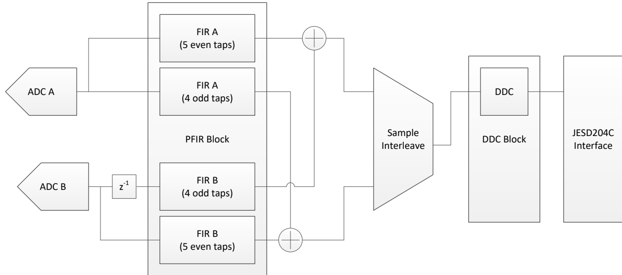
图 6-7. Alternate I/Q Correction-Type Filter Block Diagram
