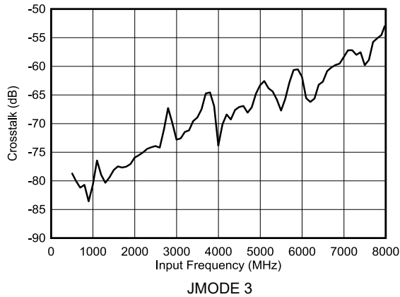
图 5-7. Dual Channel Mode: Crosstalk vs Input Frequency
