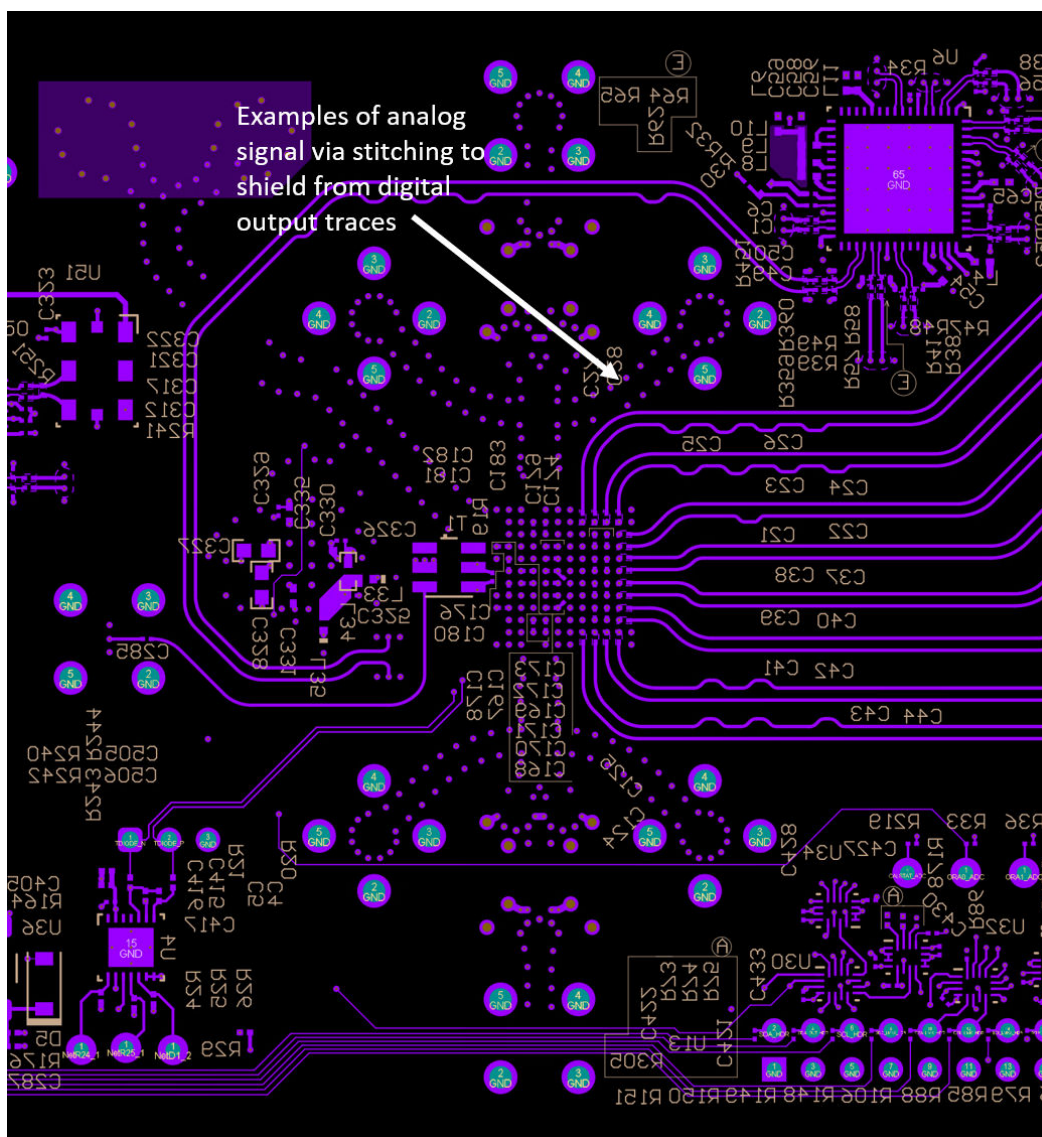
图 7-9. Example of Analog Signal Via Stitching
