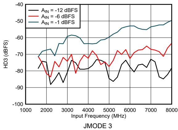
图 5-37. Dual Channel Mode: HD3 vs Input Frequency
