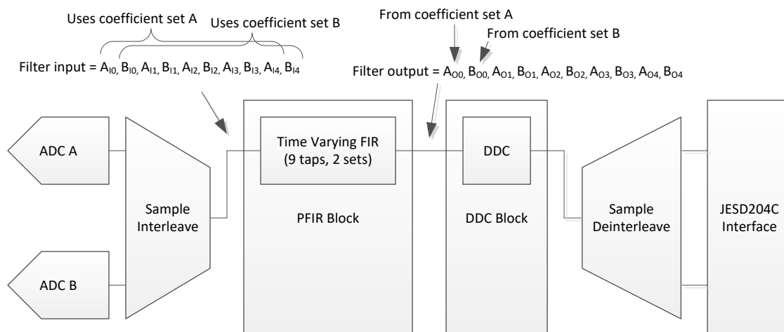
图 6-6. Time Varying Filter PFIR Block Diagram
