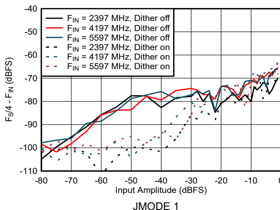
图 5-20. DES Mode: F_S/4 - F_{\text{IN}} vs Input Amplitude
