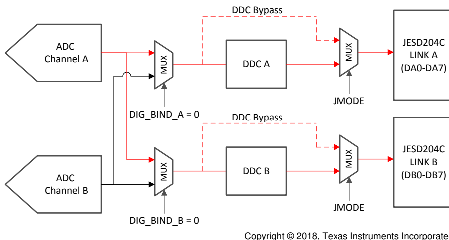
图 6-24. Dual DDC Mode or Redundant Data Mode for Channel A
