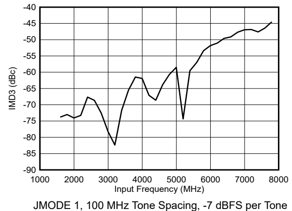
图 5-22. DES Mode: IMD3 vs Input Frequency
