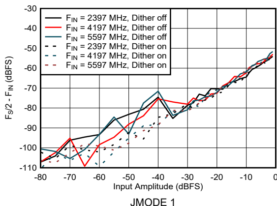
图 5-19. DES Mode: F_S/2 - F_{\text{IN}} vs Input Amplitude
