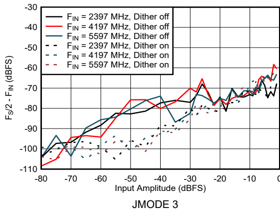
图 5-43. Dual Channel Mode: F_S/2 - F_{\text{IN}} vs Input Amplitude
