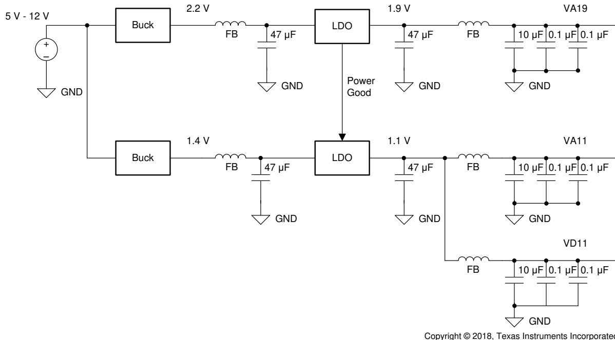
图 7-13. LDO Linear Regulator Approach Example
