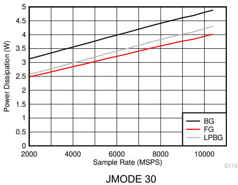
图 5-129. DES Mode: Power Dissipation vs Sample Rate
