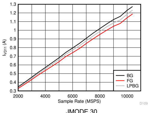
图 5-125. DES Mode: I_{VD11} vs Sample Rate
