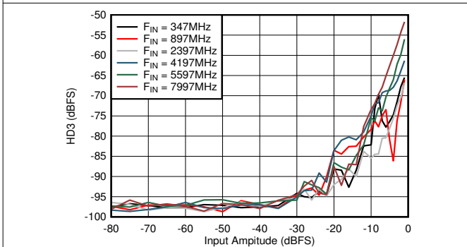
图 5-77. Dual Channel Mode: HD3 vs Input Amplitude and Frequency
