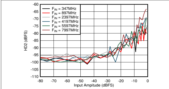
图 5-61. DES Mode: HD2 vs Input Amplitude and Frequency
