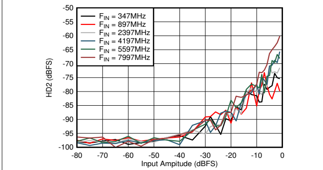
图 5-75. Dual Channel Mode: HD2 vs Input Amplitude and Frequency
