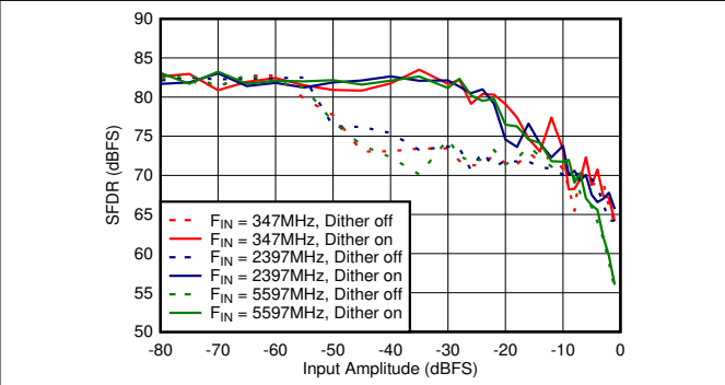
图 5-74. Dual Channel Mode: SFDR vs Input Amplitude and Dither
