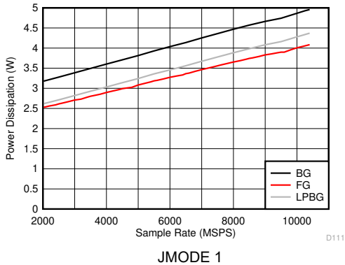
图 5-127. DES Mode: Power Dissipation vs Sample Rate
