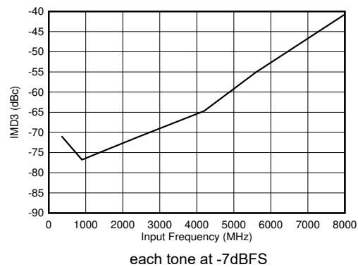
图 5-104. Dual Channel Mode: IMD3 vs Input Frequency
