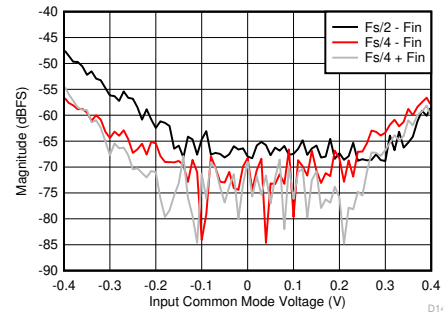
图 5-98. F_s/2 - F_{IN} and F_s/4 \pm F_{IN} vs Input Common Mode Voltage
