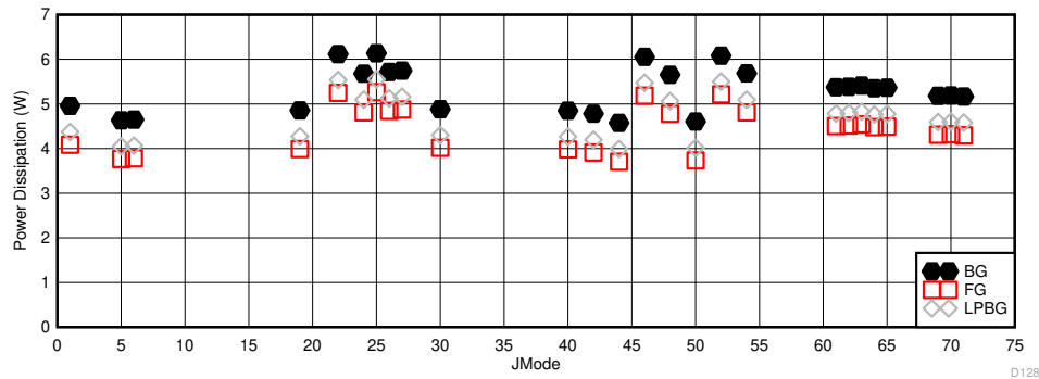
图 5-111. DES Mode: V_{D11} vs JMODE at 10.4GSPS
