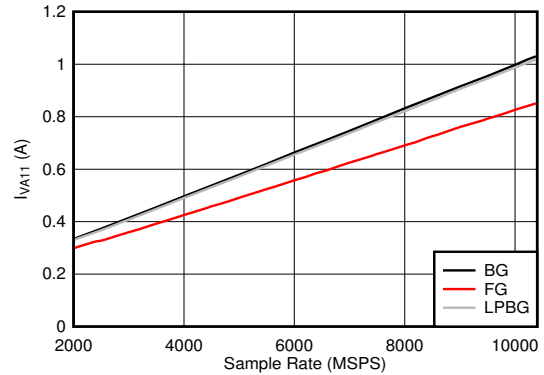
图 5-122. DES Mode: I_{VA11} vs Sample Rate
