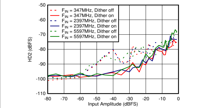
图 5-76. Dual Channel Mode: HD2 vs Input Amplitude and Dither
