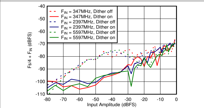
图 5-66. DES Mode: F_s/2 - F_{\text{IN}} vs Input Amplitude and Dither
