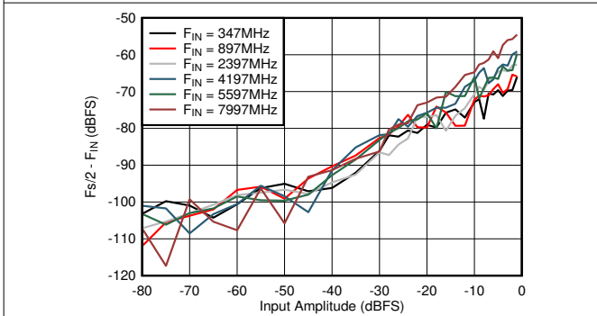
图 5-65. DES Mode: F_s/2 - F_{\text{IN}} vs Input Amplitude and Frequency
