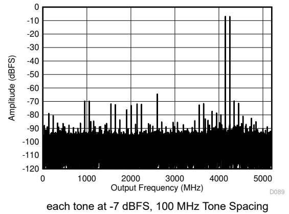
图 5-14. DES Mode: Two Tone FFT at 4197 MHz
