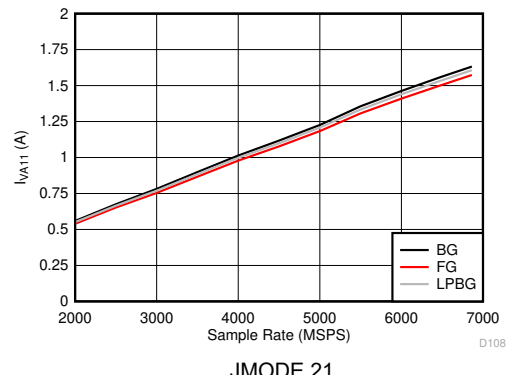
图 5-124. DES Mode: I_{VD11} vs Sample Rate
