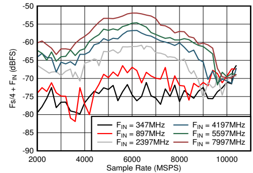
图 5-42. DES Mode: F_s/4 + F_{IN} vs Sample Rate and Input Frequency
