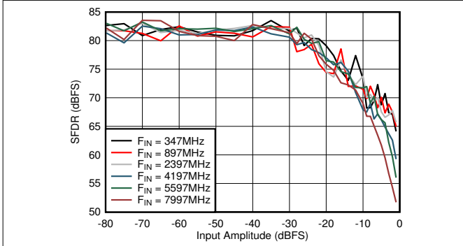
图 5-73. Dual Channel Mode: SFDR vs Input Amplitude and Frequency
