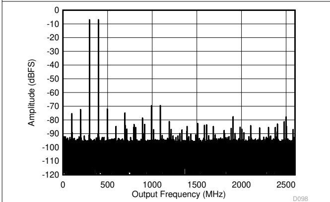
图 5-21. Dual Channel Mode: Single Tone FFT at 5597 MHz
