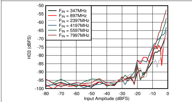
图 5-63. DES Mode: HD3 vs Input Amplitude and Frequency
