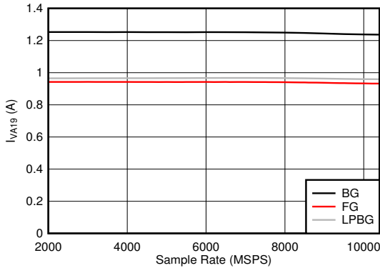
图 5-121. DES Mode: I_{VA19} vs Sample Rate
