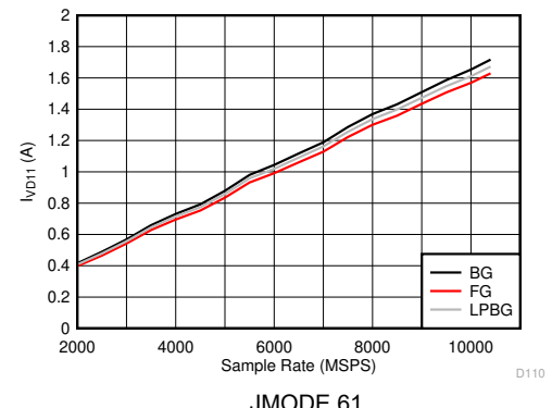
图 5-126. DES Mode: I_{VD11} vs Sample Rate
