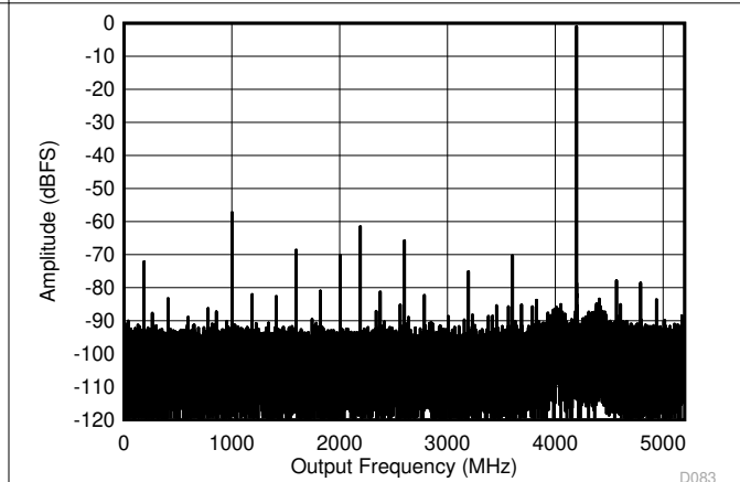
图 5-8. DES Mode: Single Tone FFT at 4197 MHz
