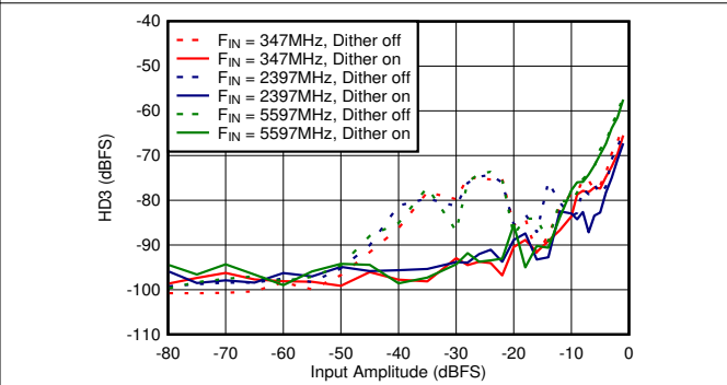
图 5-64. DES Mode: HD3 vs Input Amplitude and Dither
