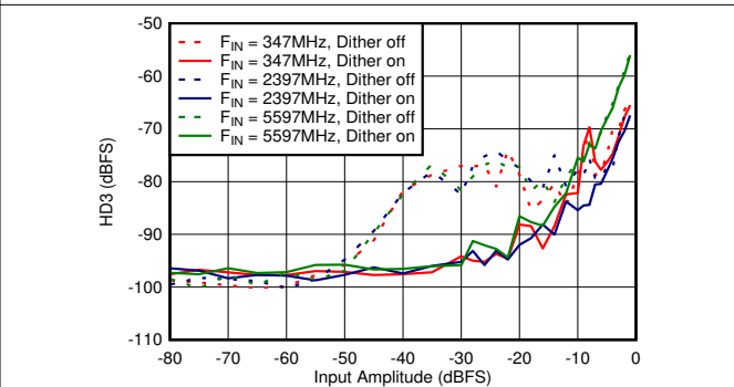
图 5-78. Dual Channel Mode: HD3 vs Input Amplitude and Dither
