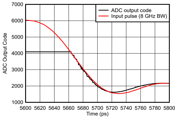
图 5-147. Pulse Overdrive Recovery Zoomed
