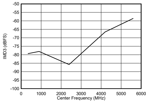
图 6-105. Dual Channel Mode: IMD3 vs Input Frequency
