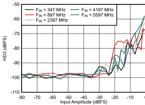
图 6-61. DES Mode: HD3 vs Input Amplitude and Frequency
