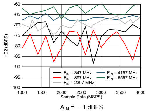
图 6-48. Dual Channel Mode: HD2 vs Sample Rate and Input Frequency
