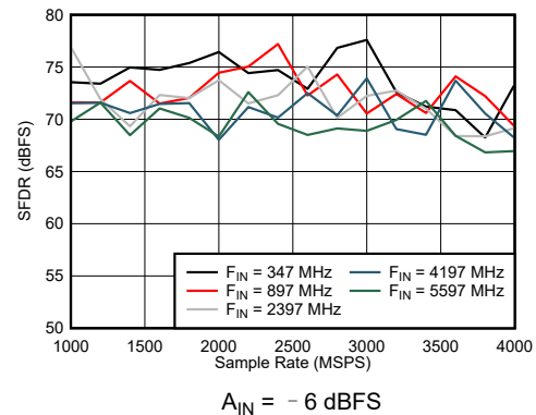
图 6-46. Dual Channel Mode: SFDR vs Sample Rate and Input Frequency
