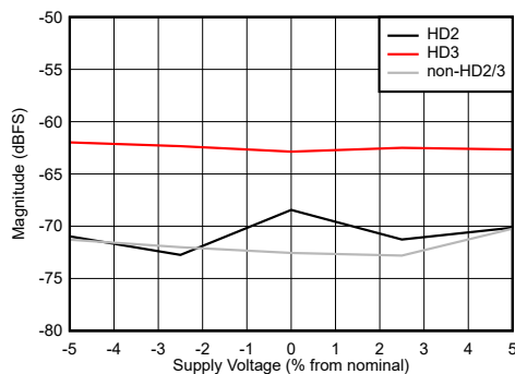
图 6-101. DES Mode: HD2, HD3 and Worst non-HD Spur vs Supply Voltage
