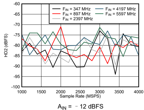
图 6-50. Dual Channel Mode: HD2 vs Sample Rate and Input Frequency
