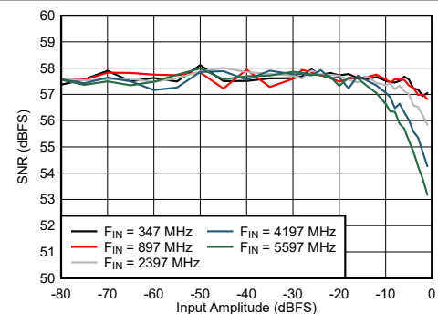
图 6-67. Dual Channel Mode: SNR vs Input Amplitude and Frequency
