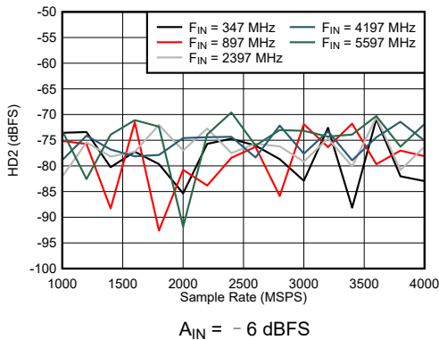
图 6-49. Dual Channel Mode: HD2 vs Sample Rate and Input Frequency
