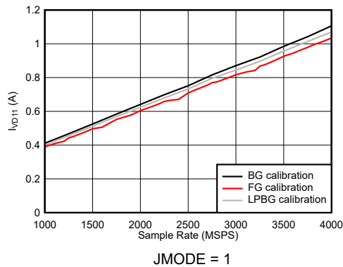
图 6-118. DES Mode: I_{VD11} vs Sample Rate
