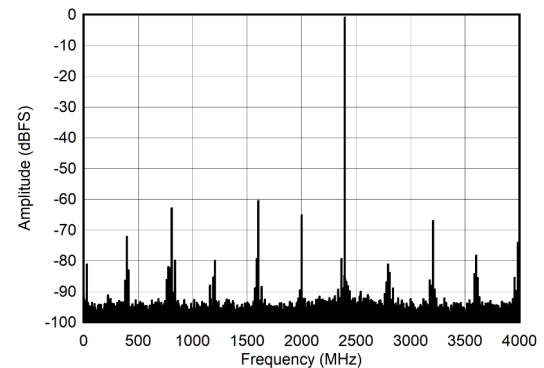
图 6-10. DES Mode: Single Tone FFT at 2397 MHz
