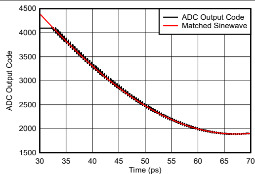
图 6-144. Sinewave Overdrive Recovery
