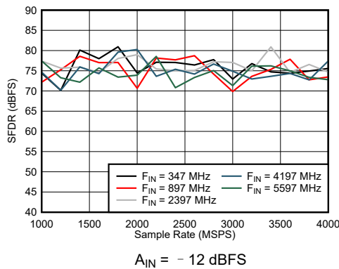
图 6-47. Dual Channel Mode: SFDR vs Sample Rate and Input Frequency
