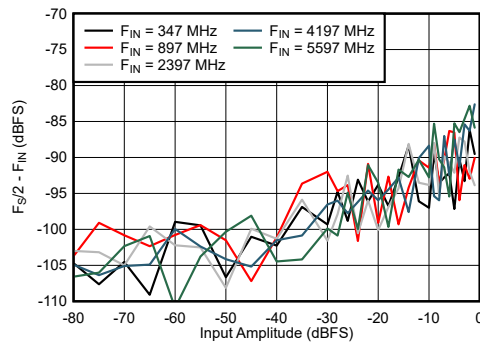
图 6-75. Dual Channel Mode: F_{S/2} - F_{IN} vs Input Amplitude and Frequency
