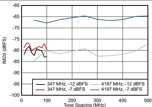
图 6-109. Dual Channel Mode: IMD3 vs Tone Spacing
