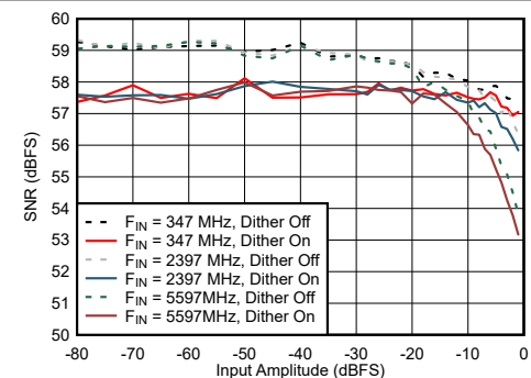
图 6-68. Dual Channel Mode: SNR vs Input Amplitude and Dither
