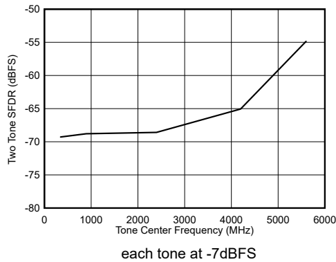
图 6-111. Dual Channel Mode: Two Tone SFDR vs Input Frequency
