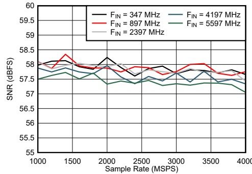
图 6-42. Dual Channel Mode: SNR vs Sample Rate and Input Frequency
