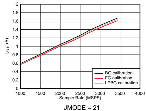
图 6-119. DES Mode: I_{VD11} vs Sample Rate
