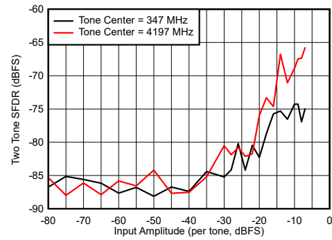
图 6-112. DES Mode: Two Tone SFDR vs Input Amplitude
