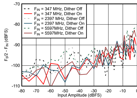
图 6-76. Dual Channel Mode: F_{S/2} - F_{IN} vs Input Amplitude and Dither
