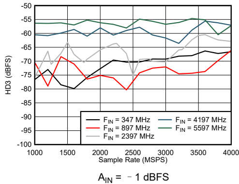
图 6-51. Dual Channel Mode: HD3 vs Sample Rate and Input Frequency
