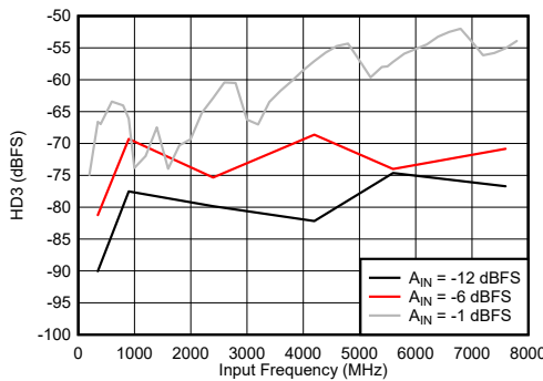
图 6-86. Dual Channel Mode: HD3 vs Input Frequency
