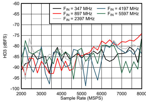
图 6-39. DES Mode: HD3 vs Sample Rate and Input Frequency
