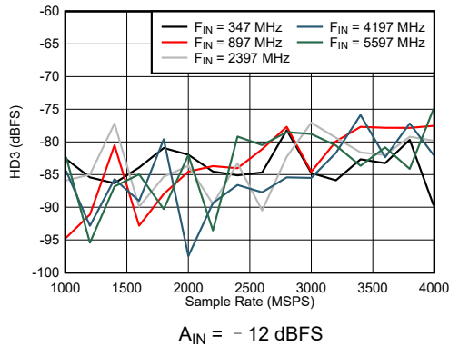
图 6-53. Dual Channel Mode: HD3 vs Sample Rate and Input Frequency
