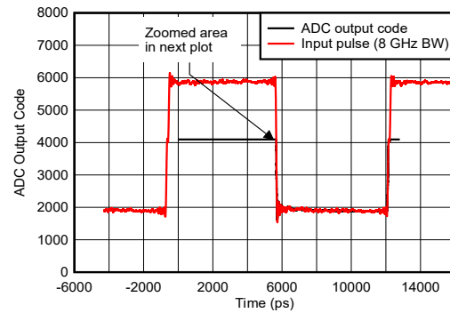
图 6-141. Pulse Overdrive Recovery
