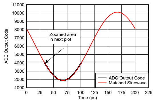
图 6-143. Sinewave Overdrive Recovery
