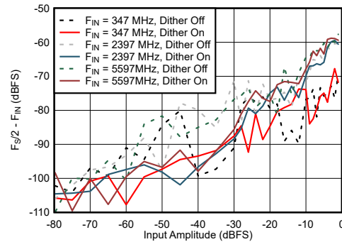
图 6-64. DES Mode: F_{S/2} - F_{\text{IN}} vs Input Amplitude and Dither
