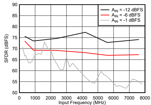
图 6-84. Dual Channel Mode: SFDR vs Input Frequency
