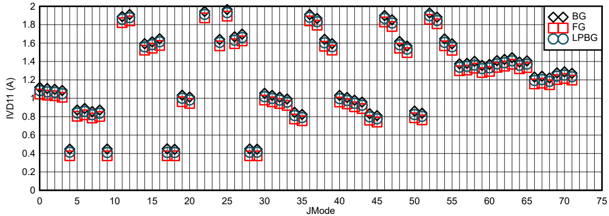
图 6-115. I_{VD11} vs \text{JMODE} at F_{\text{CLK}} = 4\text{ GHz}
