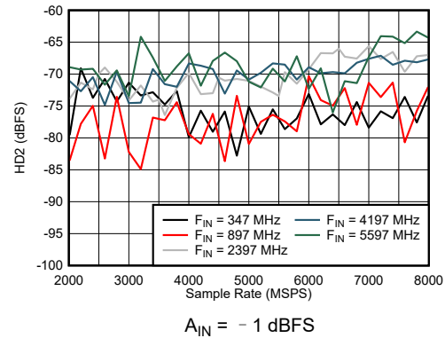
图 6-34. DES Mode: HD2 vs Sample Rate and Input Frequency
