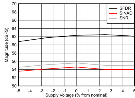
图 6-100. DES Mode: SNR, SINAD and SFDR vs Supply Voltage
