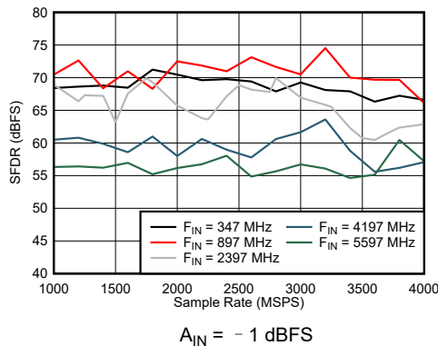
图 6-45. Dual Channel Mode: SFDR vs Sample Rate and Input Frequency
