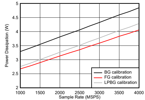
图 6-133. Dual Channel Mode: Power Dissipation vs Sample Rate
