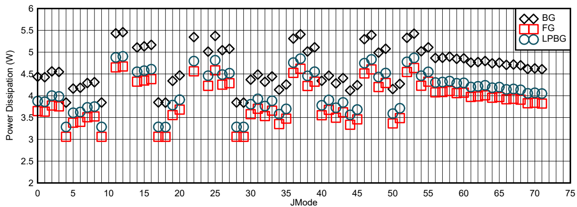
图 6-114. Power Dissipation vs JMODE at F_{\text{CLK}} = 4\text{ GHz}
