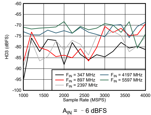
图 6-52. Dual Channel Mode: HD3 vs Sample Rate and Input Frequency
