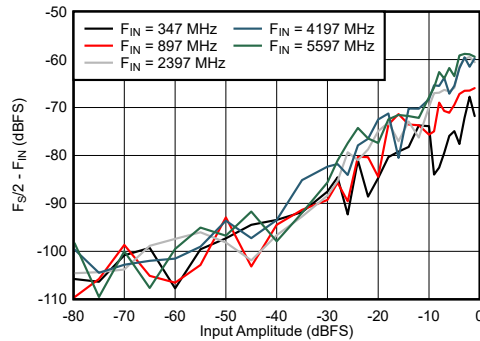
图 6-63. DES Mode: F_{S/2} - F_{\text{IN}} vs Input Amplitude and Frequency
