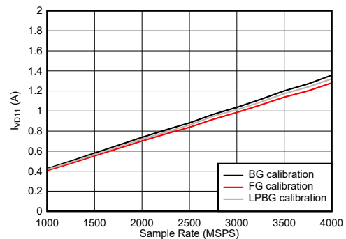
图 6-129. Dual Channel Mode: I_{VD11} vs Sample Rate
