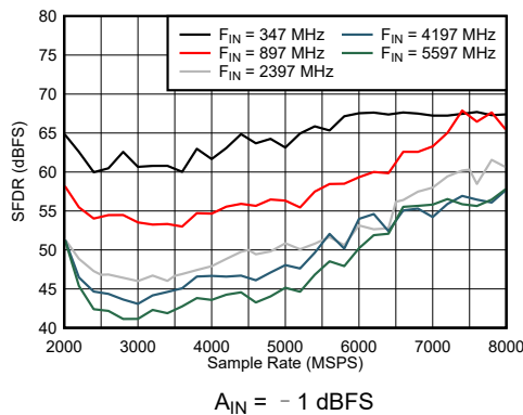
图 6-31. DES Mode: SFDR vs Sample Rate and Input Frequency
