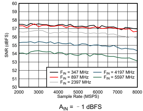
图 6-28. DES Mode: SNR vs Sample Rate and Input Frequency
