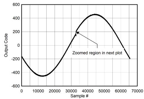
图 6-139. Background Calibration Core Transition (AC Signal)
