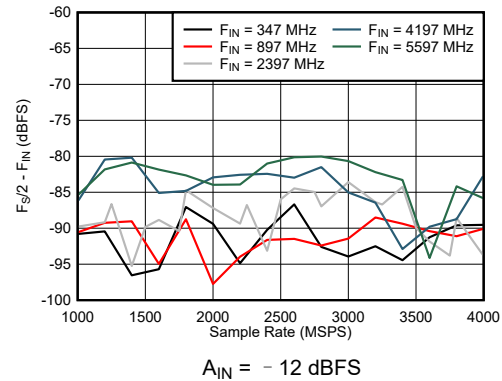
图 6-54. Dual Channel Mode: F_{S/2} - F_{\text{IN}} vs Sample Rate and Input Frequency
