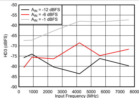
图 6-80. DES Mode: HD3 vs Input Frequency
