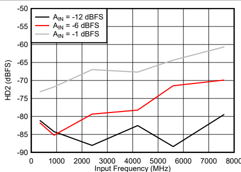
图 6-79. DES Mode: HD2 vs Input Frequency
