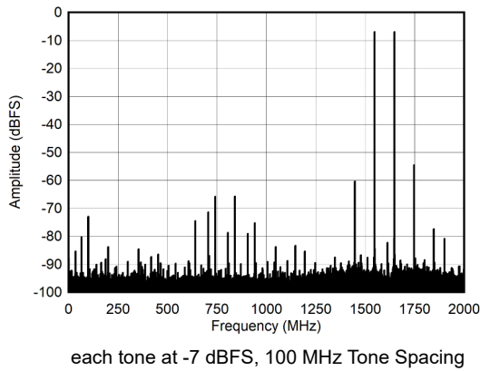
图 6-27. Dual Channel Mode: Two Tone FFT at 4197 MHz
