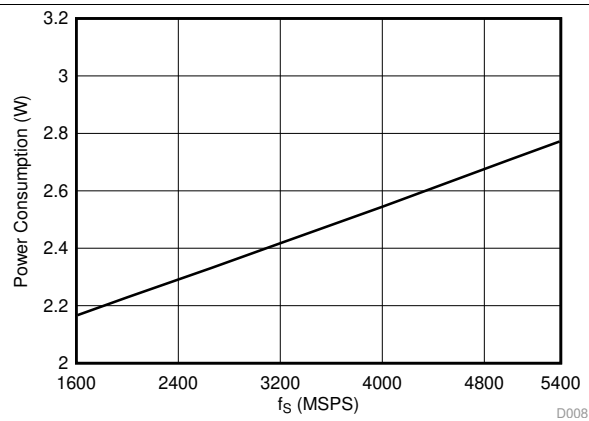
Figure 46. Power Consumption vs Sampling Rate
