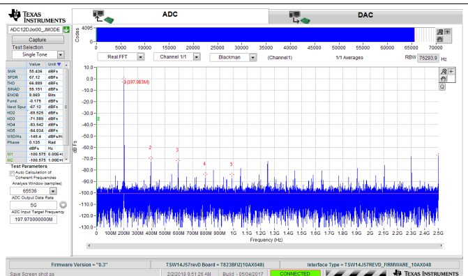
图 188. 200-MHz, Sine-Wave Frequency Domain (FFT) for 5-GSPS, Single-Channel Oscilloscope
