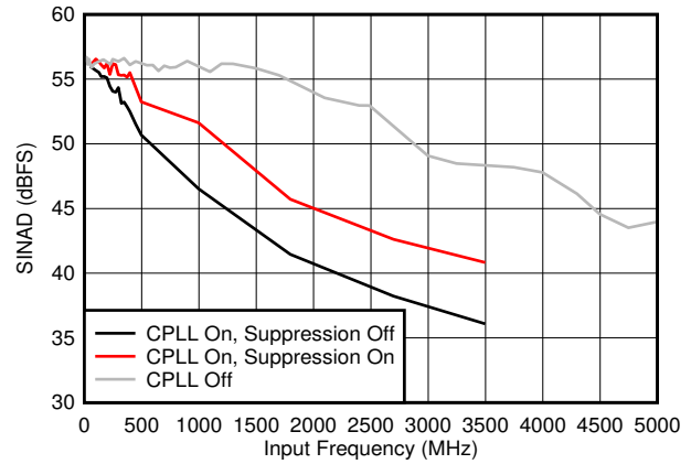
图 6-42. SINAD vs F_{IN} and C-PLL modes
