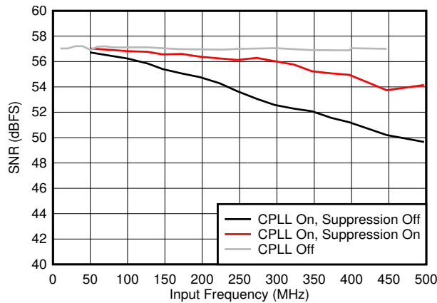
图 6-45. SNR vs F_{IN} and C-PLL modes
