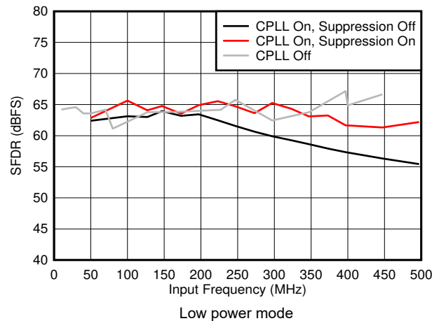
图 6-44. SFDR vs F_{IN} and C-PLL modes
