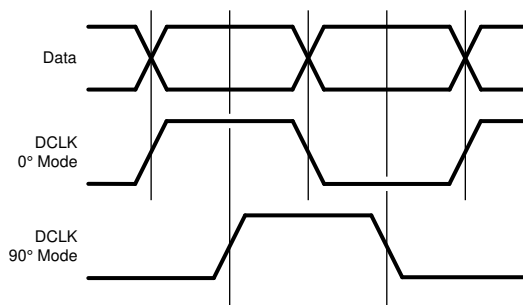
图 7-1. DDR DCLK-to-Data Phase Relationship
