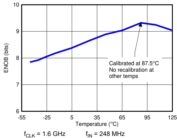
图 6-31. ENOB vs Temperature Calibration at 87.5°C Only
