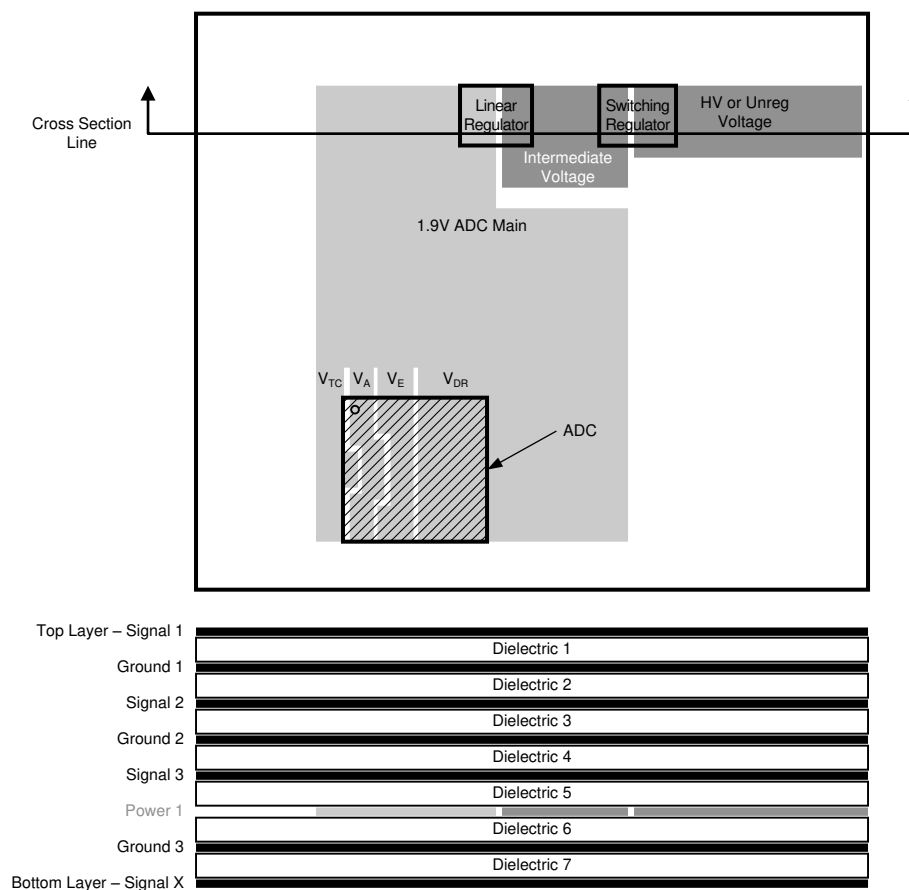
图 10-1. Power and Grounding Example
