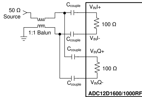
图 8-1. Driving DESIQ Mode
