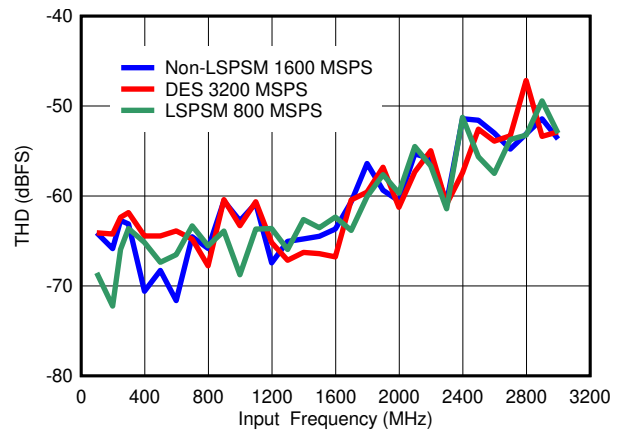
图 6-26. THD vs Input Frequency
