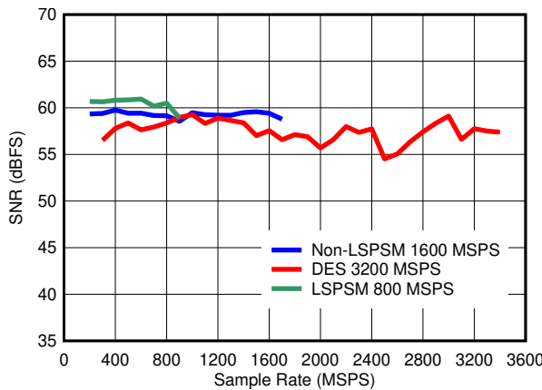
图 6-19. SNR vs Sample Rate
