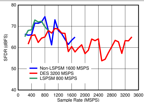
图 6-27. SFDR vs Sample Rate
