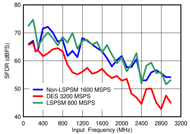
图 6-30. SFDR vs Input Frequency
