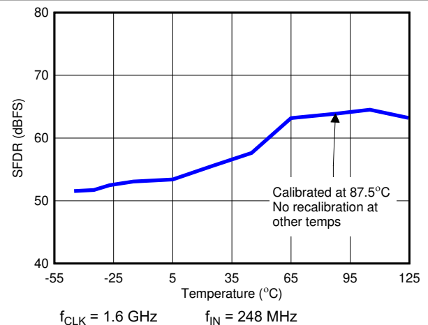
图 6-34. SFDR vs Temperature Calibration at 87.5°C Only
