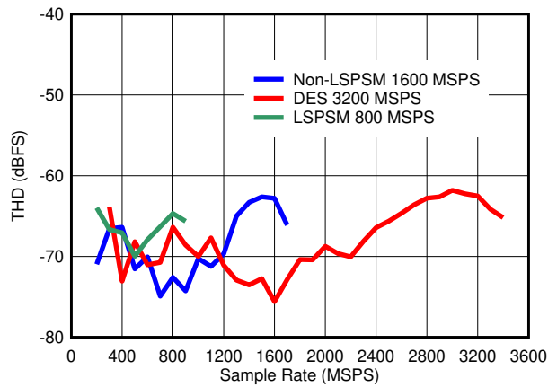
图 6-23. THD vs Sample Rate
