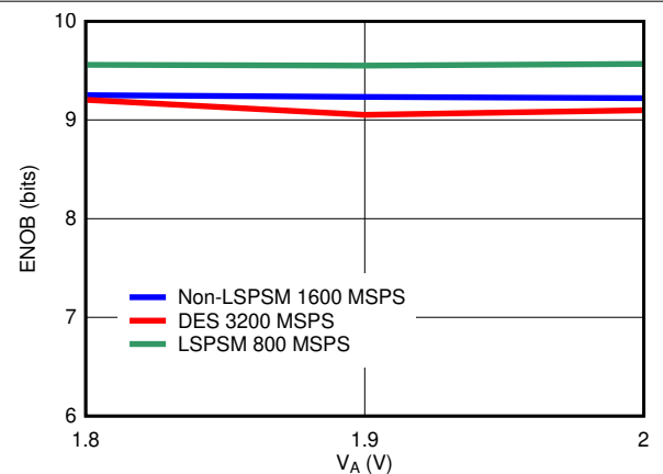
图 6-16. ENOB vs Supply Voltage
