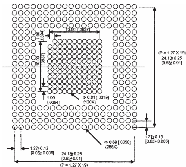
图 10-5. Landing Pattern Recommendation
