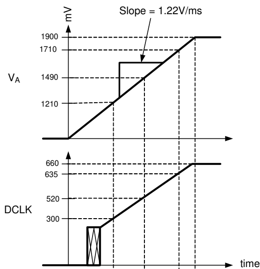
图 9-1. Supply and DCLK Ramping
