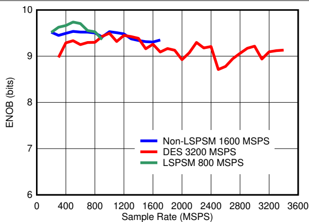
图 6-15. ENOB vs Sample Rate
