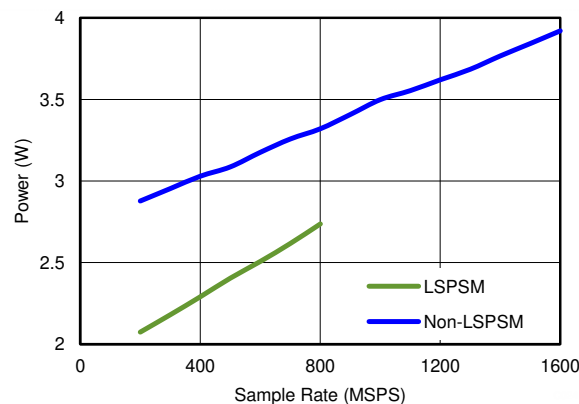
图 6-39. Power Consumption vs Sample Rate
