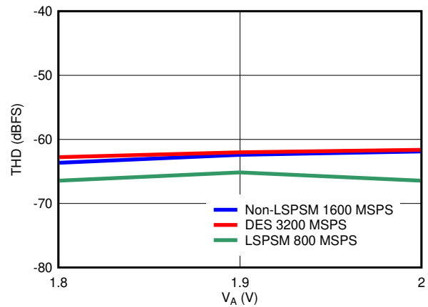
图 6-24. THD vs Supply Voltage
