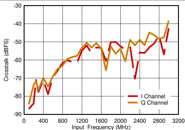
图 6-37. Cross Talk vs Input Frequency
