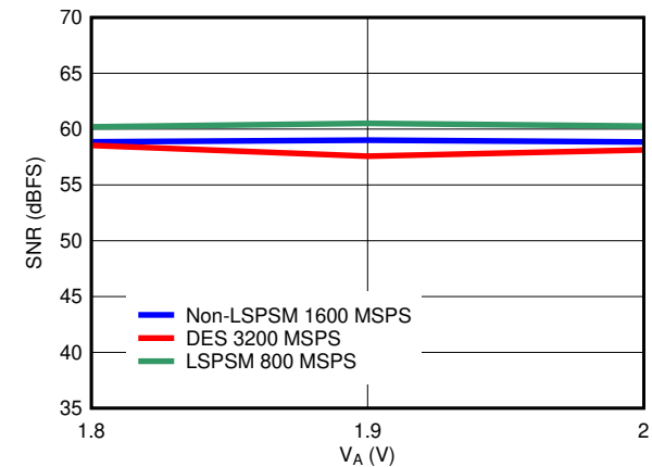
图 6-20. SNR vs Supply Voltage
