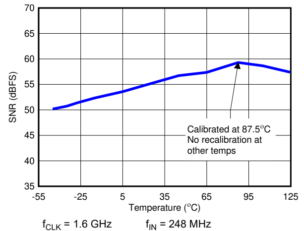
图 6-32. SNR vs Temperature Calibration at 87.5°C Only
