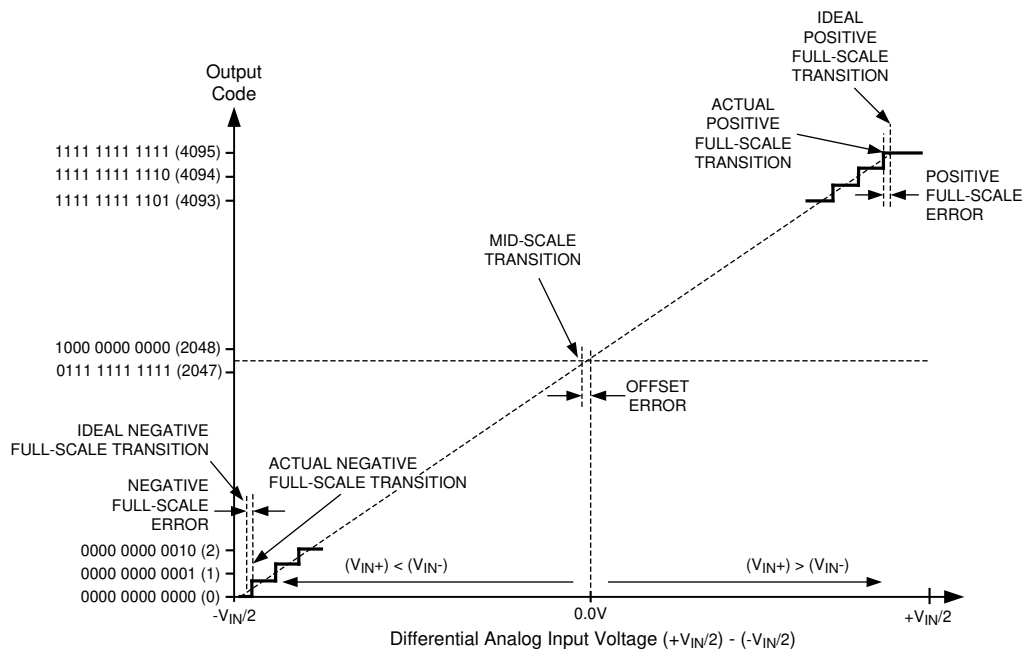
图 6-10. Input / Output Transfer Characteristic
