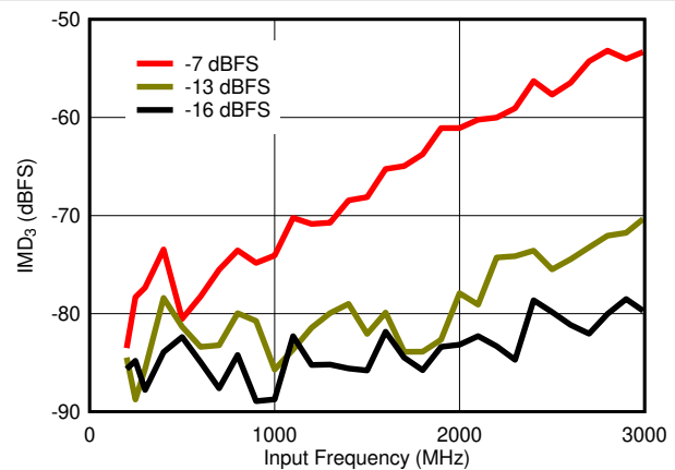
图 6-36. 3rd Order Intermodulation Distortion vs Input Frequency (DES Mode 3200 MSPS)
