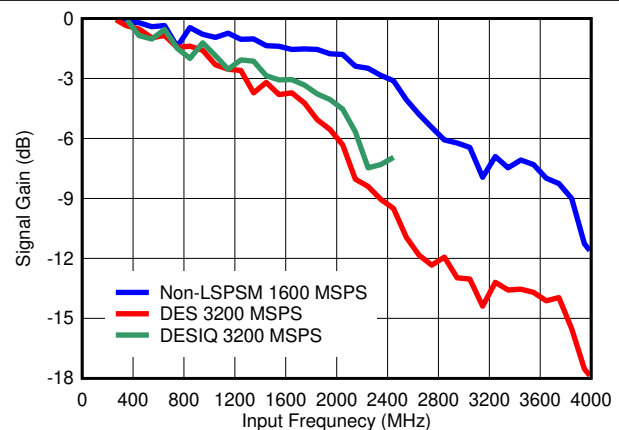
图 6-38. Insertion Loss vs Input Frequency
