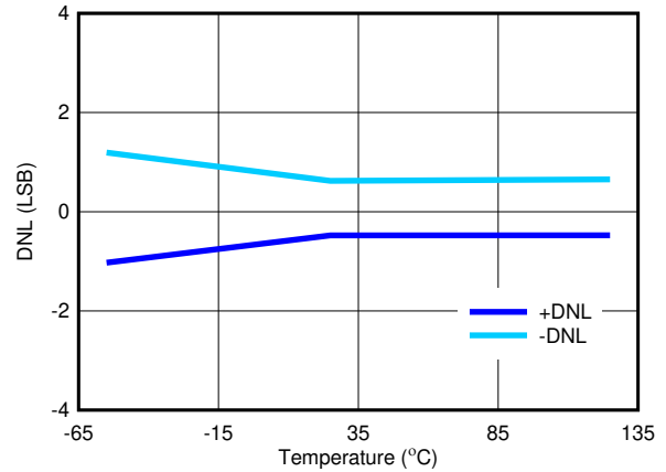
图 6-14. Minimum and Maximum DNL vs Temperature
