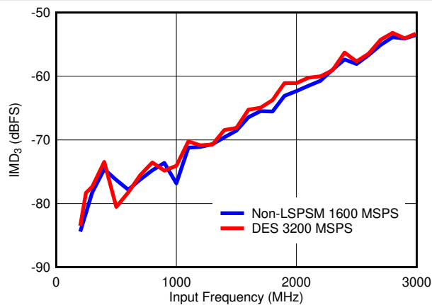
图 6-35. 3rd Order Intermodulation Distortion vs Input Frequency
