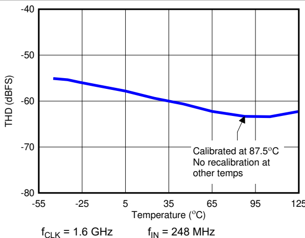
图 6-33. THD vs Temperature Calibration at 87.5°C Only
