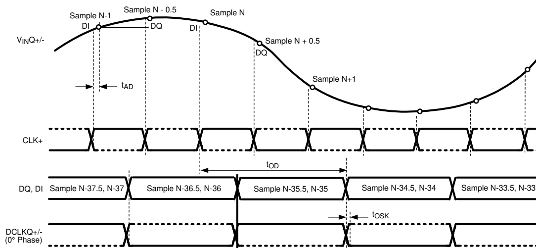
图 6-4. Clocking in Non-LSPSM, Non-Demux Mode DES Mode*
