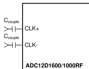
Figure 8-4. Differential Input Clock Connection
