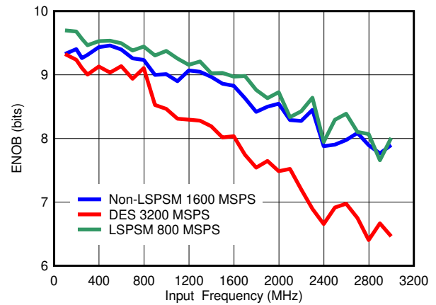
图 6-18. ENOB vs Input Frequency
