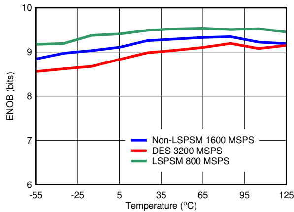
图 6-17. ENOB vs Temperature
