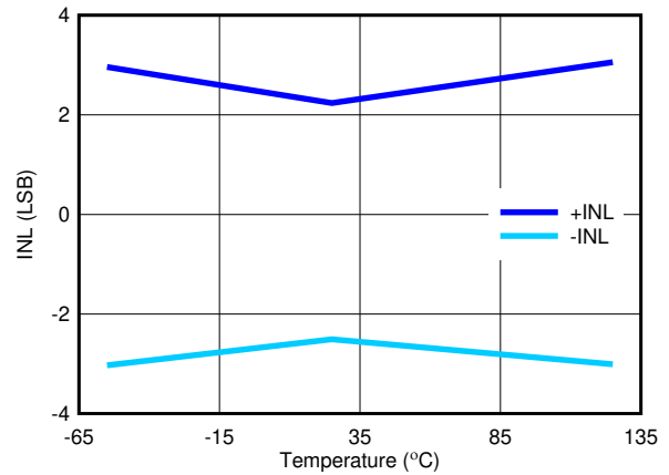
图 6-12. Minimum and Maximum INL vs Temperature
