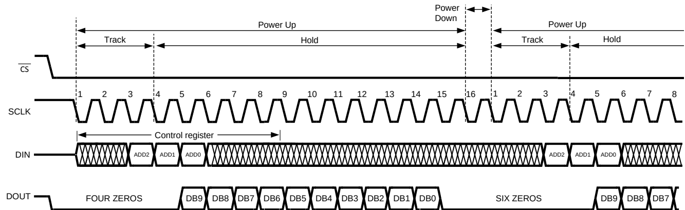
Figure 1. ADC108S102 Operational Timing Diagram
