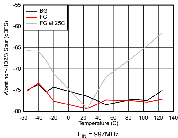
图 5-39. Worst non-HD2/3 Spur vs Temperature
