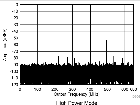
Figure 5-10. Single Tone FFT at 3497 MHz and -1 dBFS
