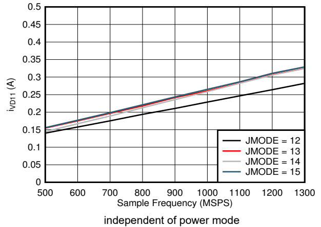
Figure 5-100. Dual Channel, I_{VD11} vs FS and JMODE 12 - 15
