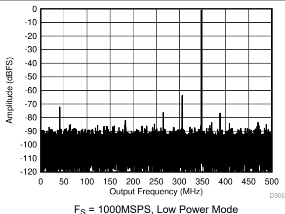
Figure 5-12. Single Tone FFT at 347 MHz and -1 dBFS
