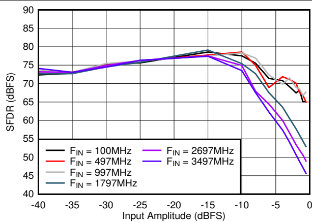
Figure 5-29. SFDR vs Input Amplitude
