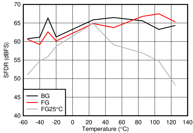
图 5-43. SFDR vs Temperature and Calibration Mode
