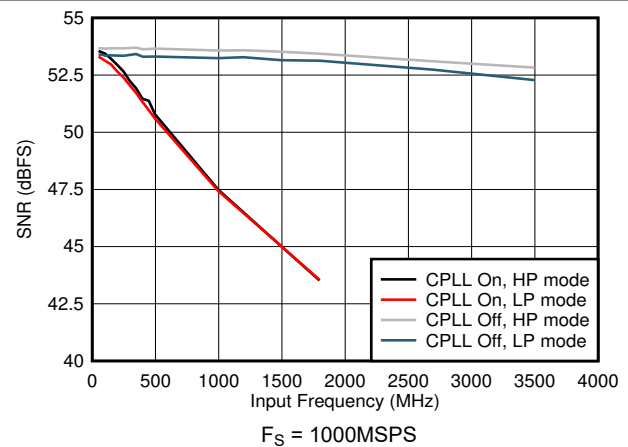
图 5-66. SNR vs Input Frequency and CPLL
