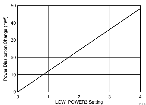
图 6-13. Power Dissipation Change vs LOW_POWER3 register setting
