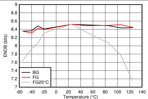
图 5-42. ENOB vs Temperature and Calibration Mode
