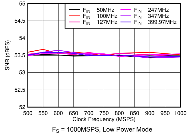
图 5-26. SNR vs Sample Rate
