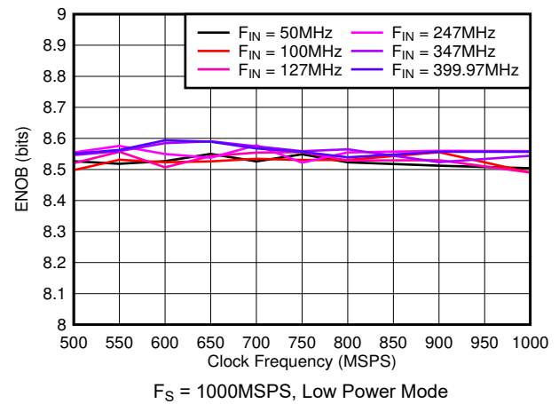
图 5-28. ENOB vs Sample Rate
