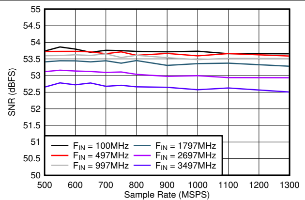
图 5-22. SNR vs Sample Rate
