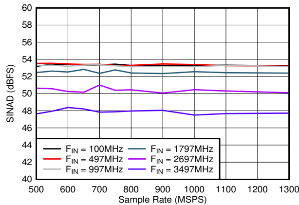
图 5-23. SINAD vs Sample Rate
