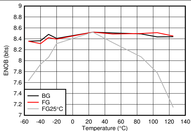
图 5-42. ENOB vs Temperature and Calibration Mode
