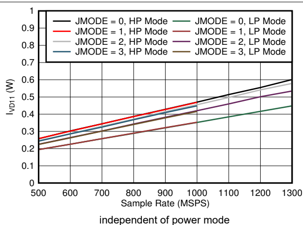
图 5-87. Quad Channel, I_{VD11} vs FS and JMODE 0 - 3
