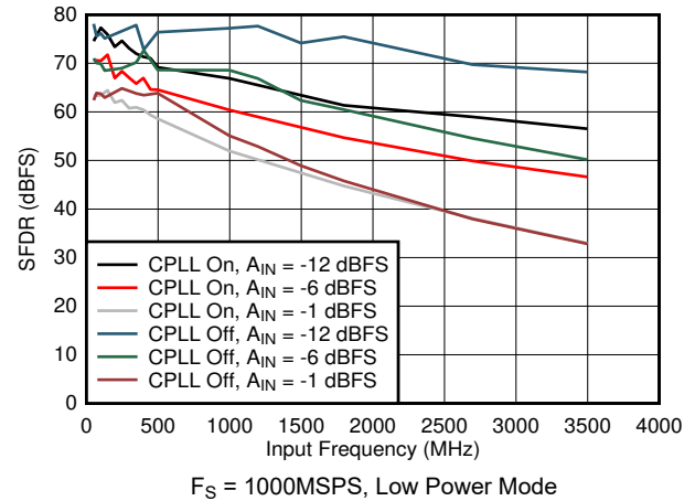
图 5-76. SFDR vs Input Frequency, CPLL and Input Amplitude
