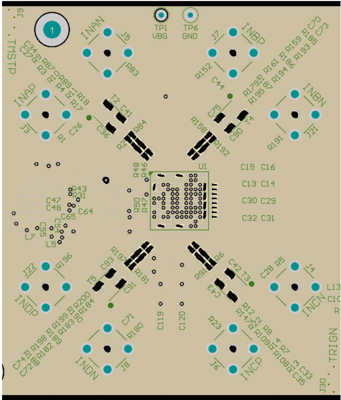
图 7-7. GND1 Cutouts to Optimize Impedance of Component Pads
