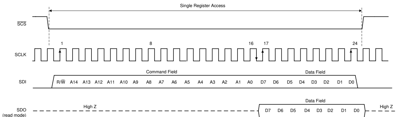
图 6-18. Serial Interface Protocol: Single Read/Write
