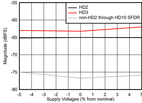
图 5-49. HD2, HD3 and Worst non-HD2/3 Spur vs Supply Voltage
