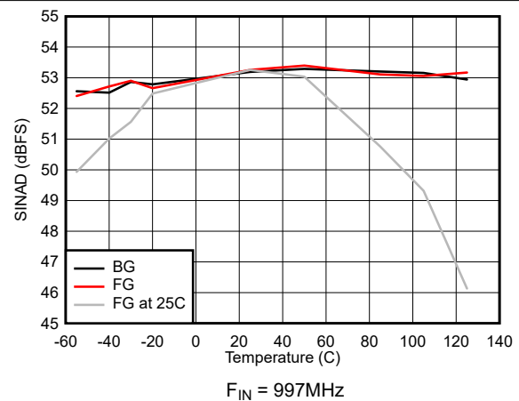
图 5-36. SINAD vs Temperature
