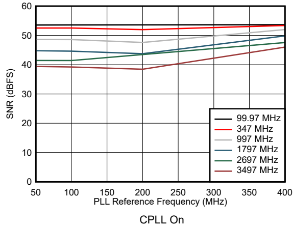
图 5-63. SNR vs Reference Clock Frequency
