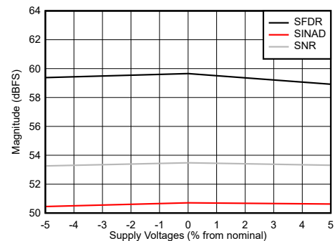
图 5-48. SNR, SFDR and SINAD vs Supply Voltage
