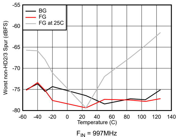
图 5-39. Worst non-HD2/3 Spur vs Temperature
