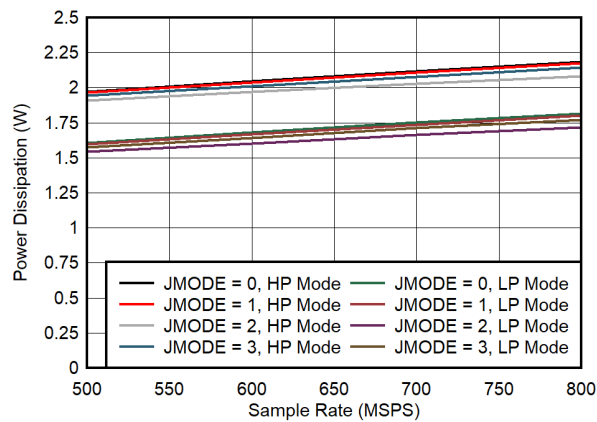
图 5-71. Quad Channel, Power Dissipation vs F_S for JMODES 0 - 3
