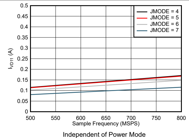
图 5-98. Single Channel, I_{VD11} vs F_S for JMODES 4 - 7
