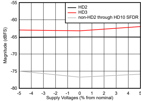
图 5-49. HD2, HD3 and Worst non-HD2/3 Spur vs Supply Voltage
