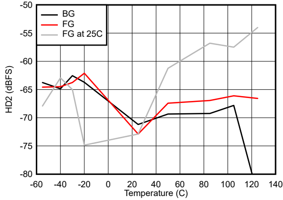
图 5-43. HD2 vs Temperature
