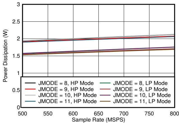
图 5-73. Quad Channel, Power Dissipation vs F_S for JMODES 8 - 11
