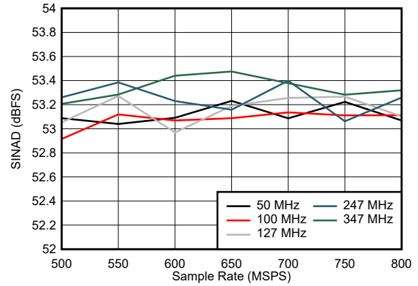
图 5-26. SINAD vs Sample Rate
