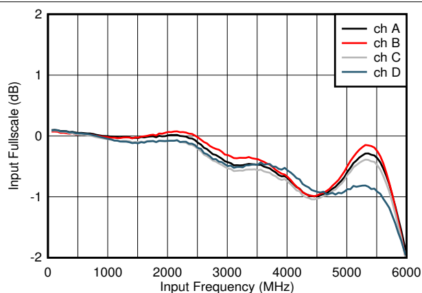
图 5-3. Input Fullscale vs Input Frequency
