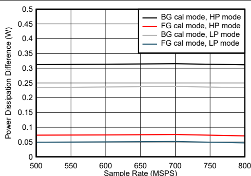
图 5-101. Quad Channel, Power Dissipation Change with Calibration Mode
