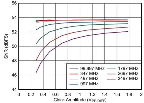
图 5-32. SNR vs Clock Amplitude
