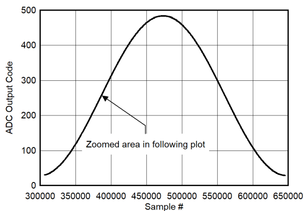
图 5-117. Background Core Transition (AC Signal)
