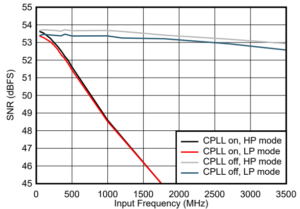
图 5-66. SNR vs Input Frequency and CPLL and Power Mode
