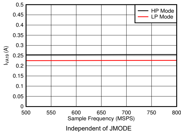
图 5-95. Single Channel, I_{VA19} vs F_S
