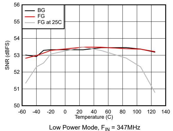
图 5-40. SNR vs Temperature
