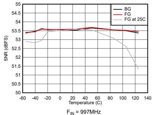
图 5-34. SNR vs Temperature
