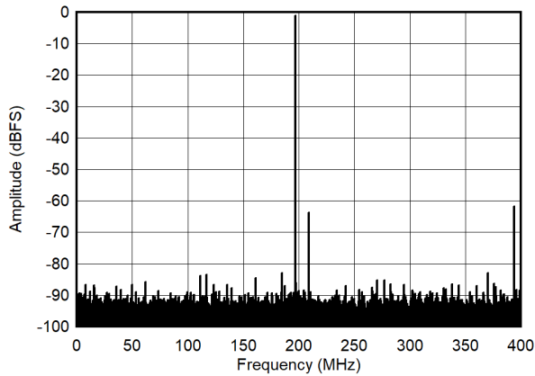
图 5-7. Single Tone FFT at 1797 MHz and -1dBFS
