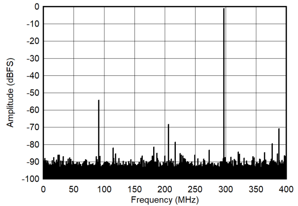
图 5-8. Single Tone FFT at 2697 MHz and -1dBFS
