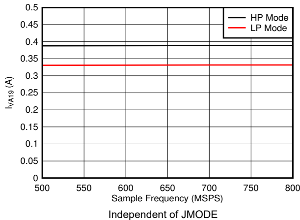
图 5-85. Dual Channel, I_{VA19} vs F_S
