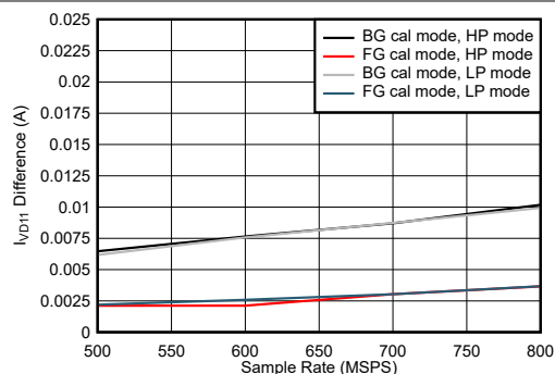
图 5-112. Single Channel, I_{VD11} Change with Calibration Mode
