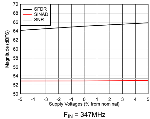
图 5-46. SNR, SFDR and SINAD vs Supply Voltage
