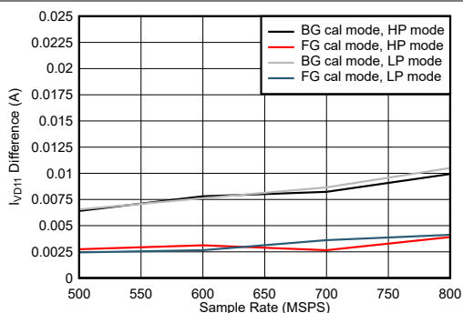
图 5-111. Dual Channel, I_{VD11} Change with Calibration Mode
