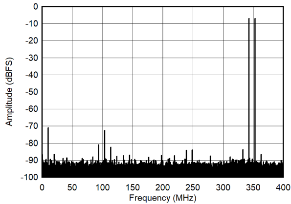
图 5-57. Dual Tone FFT at 348 MHz (LP Mode)
