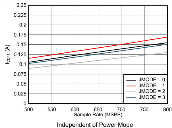
图 5-97. Single Channel, I_{VD11} vs F_S for JMODES 0 - 3
