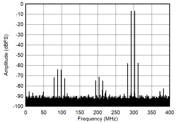
图 5-54. Dual Tone FFT at 2698 MHz
