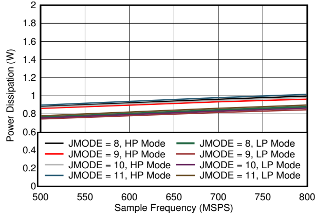
图 5-93. Single Channel, Power Dissipation vs F_S for JMODES 8 - 11
