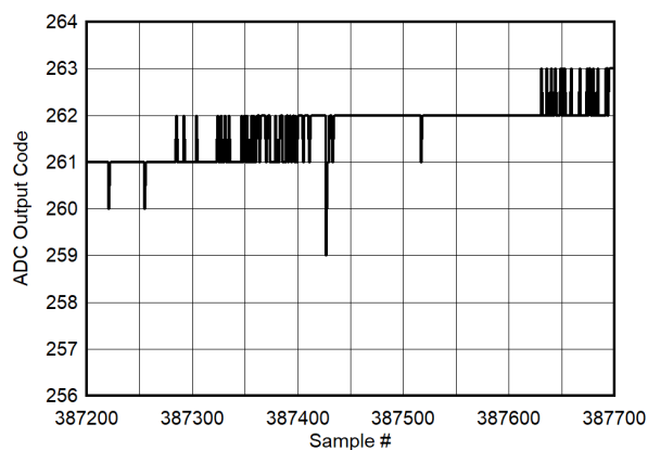
图 5-118. Background Core Transition (AC Signal Zoomed)
