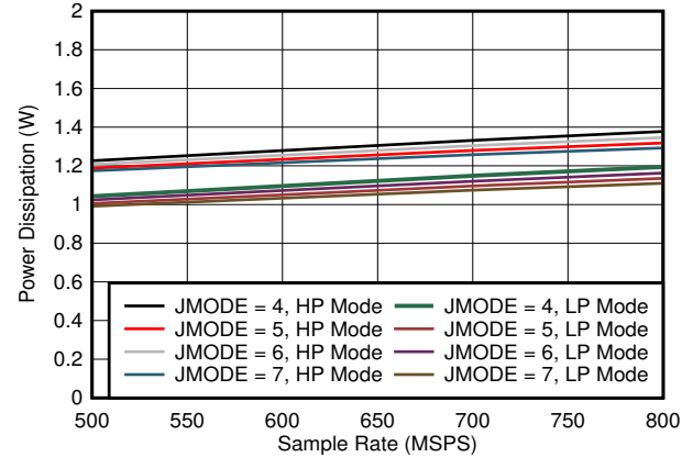
图 5-82. Dual Channel, Power Dissipation vs F_S for JMODES 4 - 7
