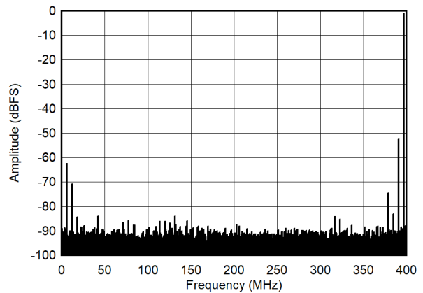
图 5-12. Single Tone FFT at 1197MHz and -1dBFS
