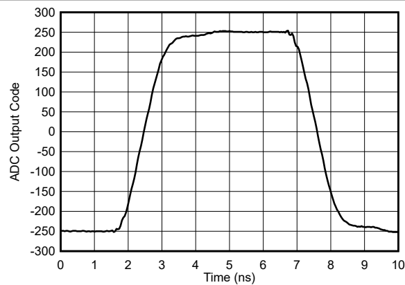
图 7-2. Measured Pulse using Sub-Sampling Technique for Equivalent 25.6 GSPS Measurement
