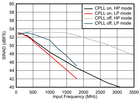
图 5-67. SINAD vs Input Frequency and CPLL and Power Mode
