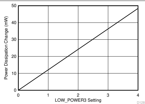
图 6-13. Power Dissipation Change vs LOW_POWER3 register setting
