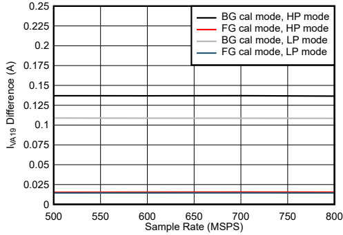
图 5-105. Dual Channel, I_{VA19} Change with Calibration Mode
