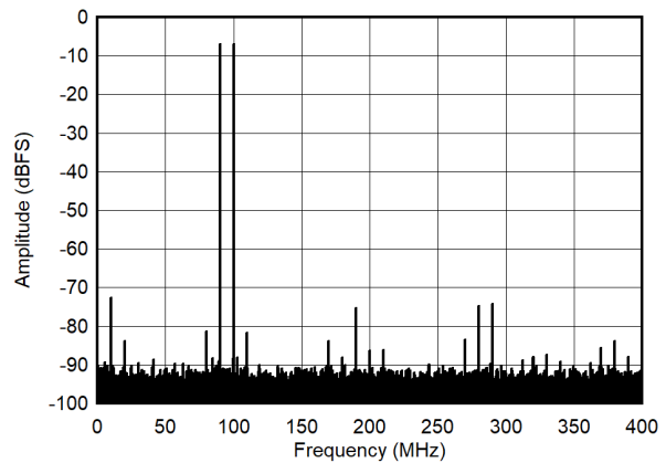
图 5-56. Dual Tone FFT at 95 MHz (LP Mode)
