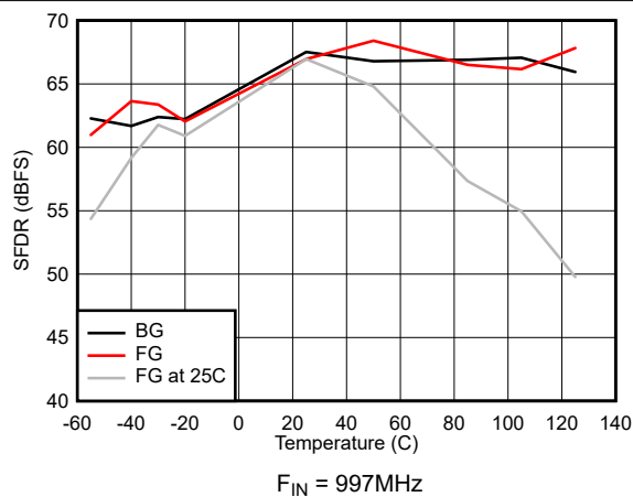
图 5-35. SFDR vs Temperature
