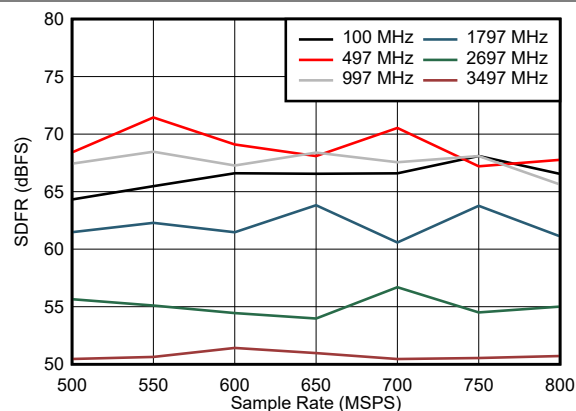
图 5-20. SFDR vs Sample Rate
