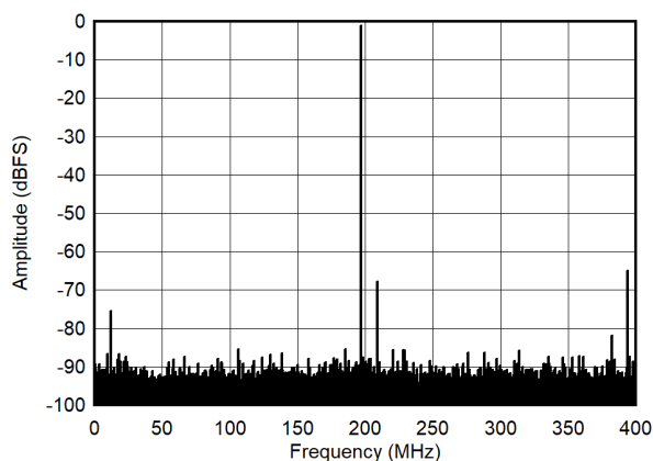
图 5-5. Single Tone FFT at 997 MHz and -1dBFS
