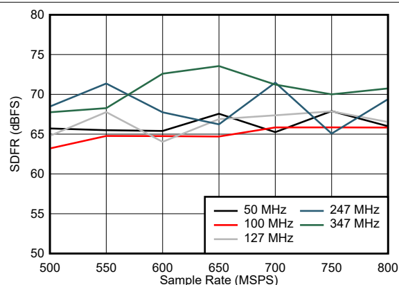
图 5-24. SFDR vs Sample Rate Low Power Mode
