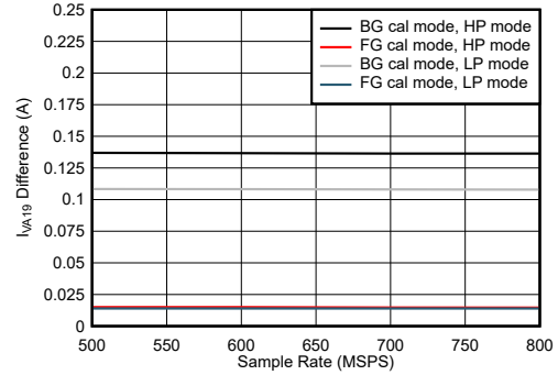
图 5-106. Single Channel, I_{VA19} Change with Calibration Mode
