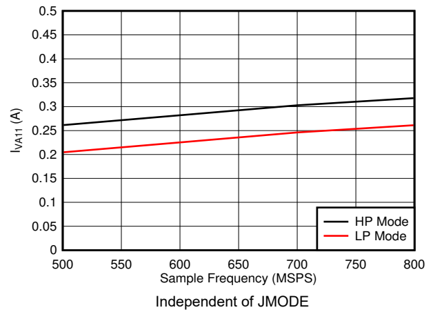
图 5-96. Single Channel, I_{VA11} vs F_S
