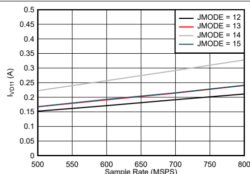
图 5-80. Quad Channel, I_{VD11} vs F_S for JMODES 12 - 15
