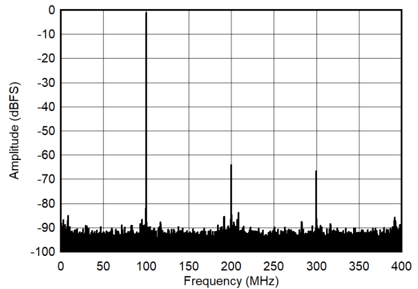
图 5-10. Single Tone FFT at 100MHz and -1dBFS
