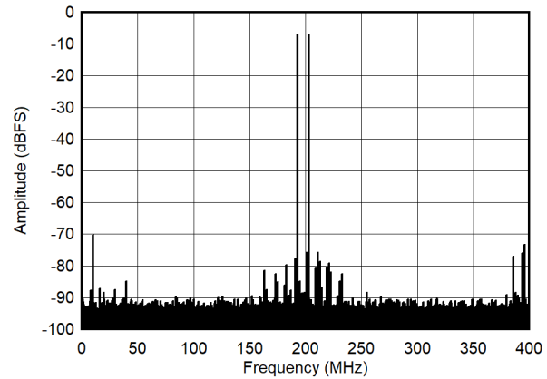
图 5-58. Dual Tone FFT at 998 MHz (LP Mode)
