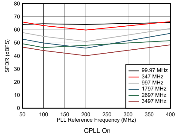
图 5-64. SFDR vs Reference Clock Frequency
