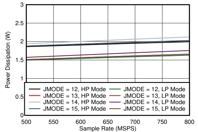
图 5-74. Quad Channel, Power Dissipation vs F_S for JMODES 12 - 15
