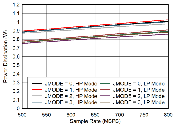
图 5-91. Single Channel, Power Dissipation vs F_S for JMODES 0 - 3
