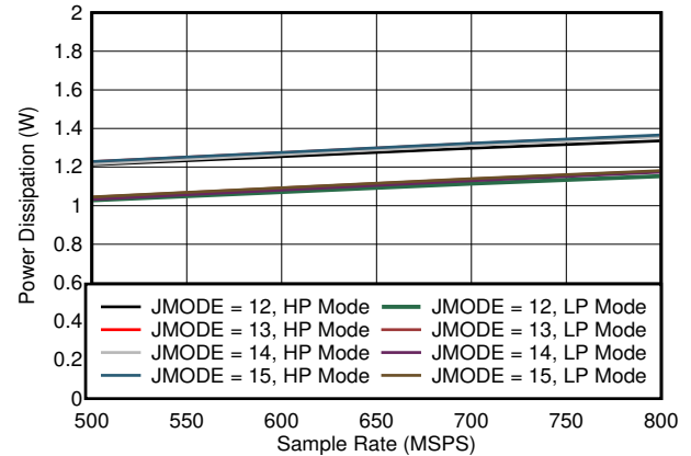
图 5-84. Dual Channel, Power Dissipation vs F_S for JMODES 12 - 15
