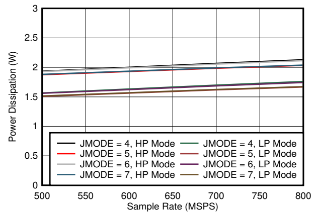
图 5-72. Quad Channel, Power Dissipation vs F_S for JMODES 4 - 7
