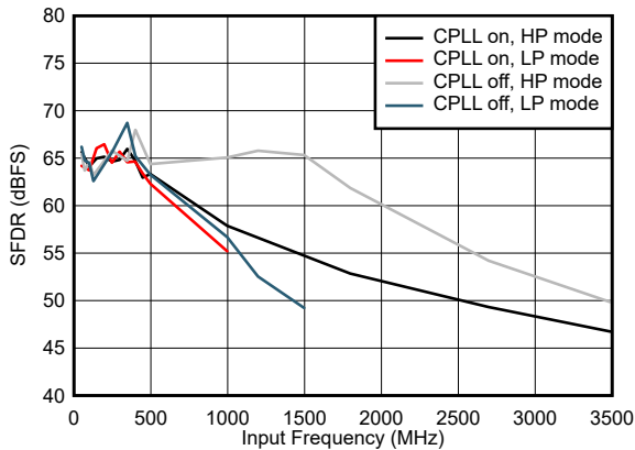
图 5-65. SFDR vs Input Frequency and CPLL and Power Mode
