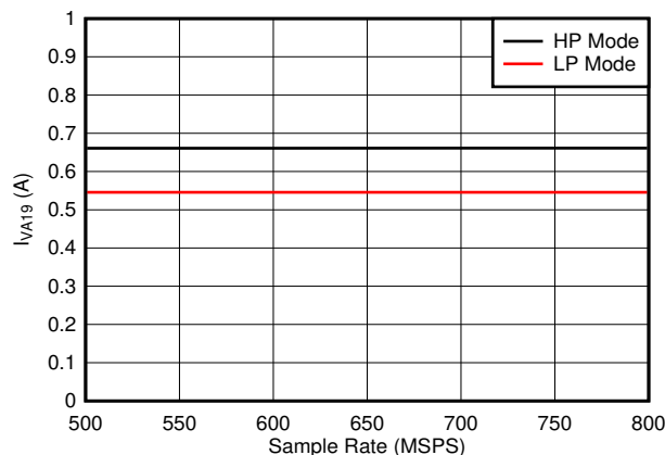
图 5-75. Quad Channel, I_{VA19} vs F_S
