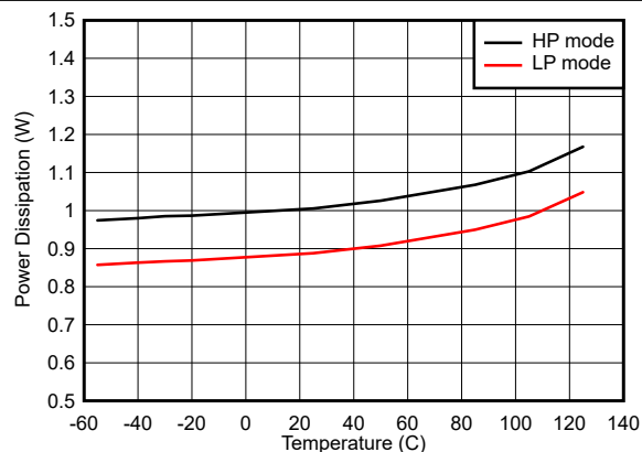
图 5-113. Quad Channel, Power Dissipation vs Temperature
