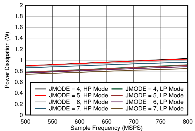
图 5-92. Single Channel, Power Dissipation vs F_S for JMODES 4 - 7
