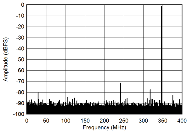
图 5-11. Single Tone FFT at 347MHz and -1dBFS
