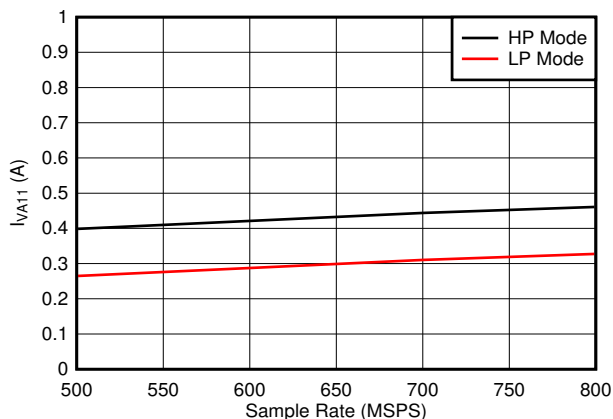
图 5-76. Quad Channel, I_{VA11} vs F_S
