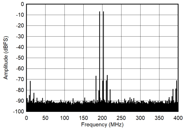
图 5-53. Dual Tone FFT at 1798 MHz
