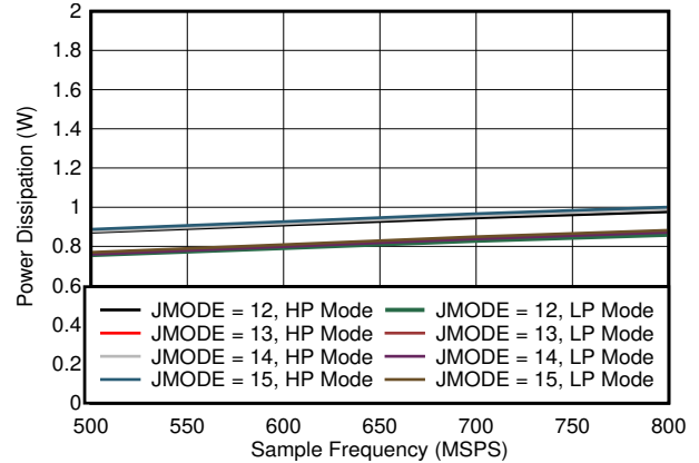
图 5-94. Single Channel, Power Dissipation vs F_S for JMODES 12 - 15
