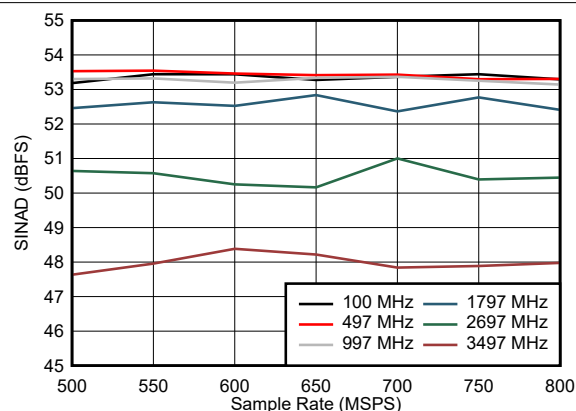
图 5-22. SINAD vs Sample Rate
