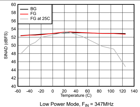
图 5-42. SINAD vs Temperature
