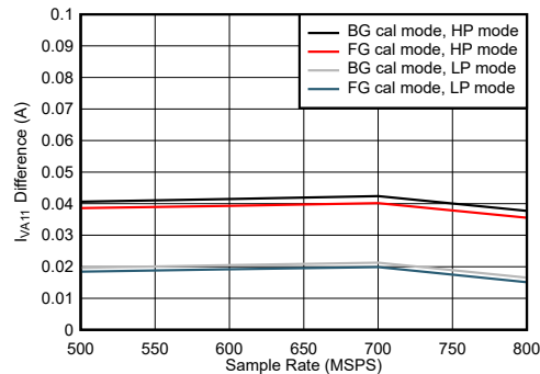
图 5-107. Quad Channel, I_{VA11} Change with Calibration Mode
