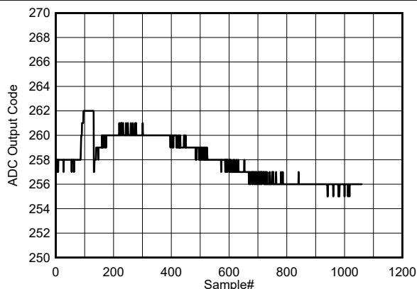
图 5-116. Background Core Transition (DC midscale input)
