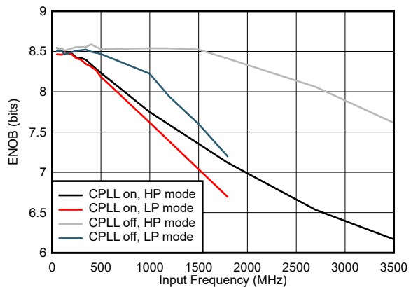
图 5-68. ENOB vs Input Frequency and CPLL and Power Mode
