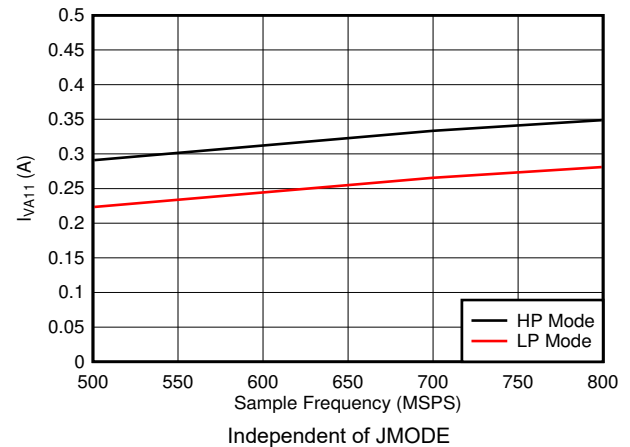
图 5-86. Dual Channel, I_{VA11} vs F_S
