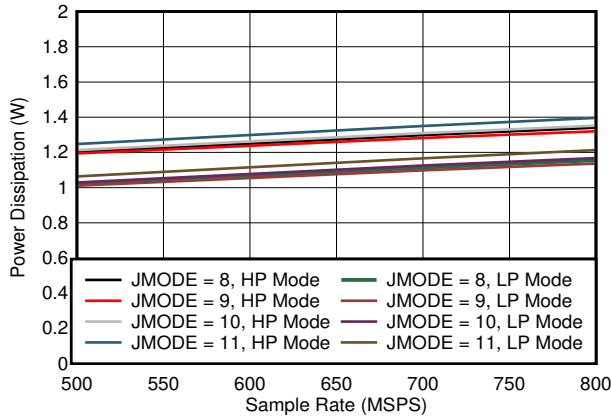
图 5-83. Dual Channel, Power Dissipation vs F_S for JMODES 8 - 11
