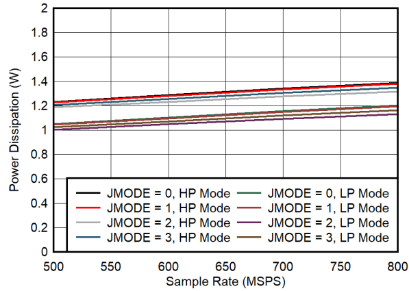
图 5-81. Dual Channel, Power Dissipation vs F_S for JMODES 0 - 3
