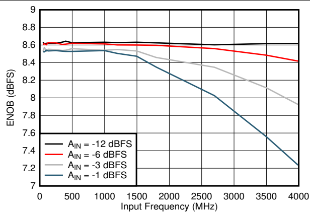
图 5-18. ENOB vs Input Frequency
