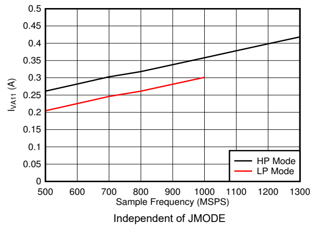
图 5-106. Single Channel, I_{VA11} vs FS
