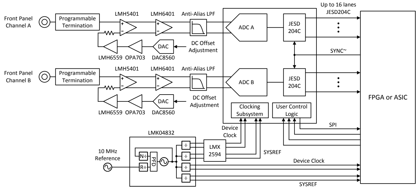
图 7-3. Typical Configuration for Reconfigurable Oscilloscope
