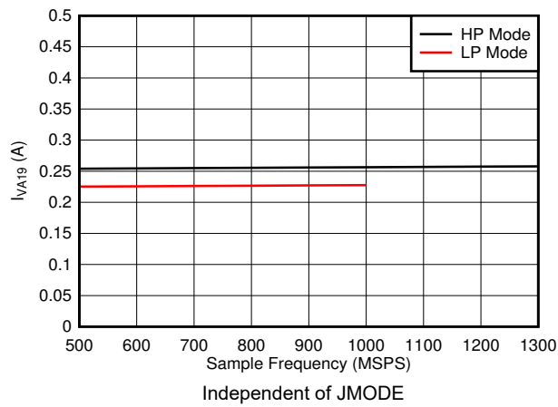
图 5-105. Single Channel, I_{VA19} vs FS
