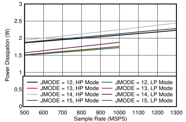
图 5-84. Quad Channel, Power Dissipation vs FS for JMODES 12 - 15
