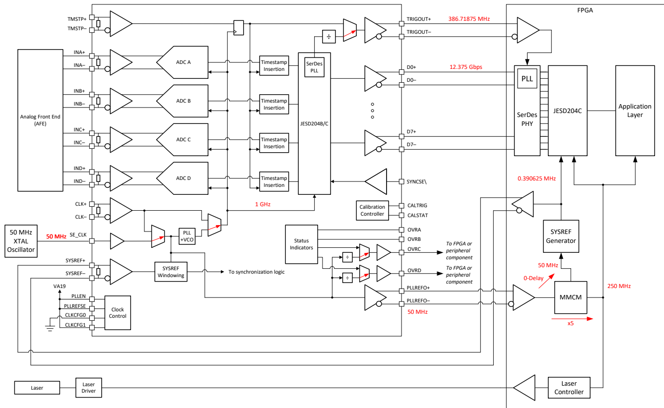
图 7-1. Typical Configuration for a LiDAR Digitizer
