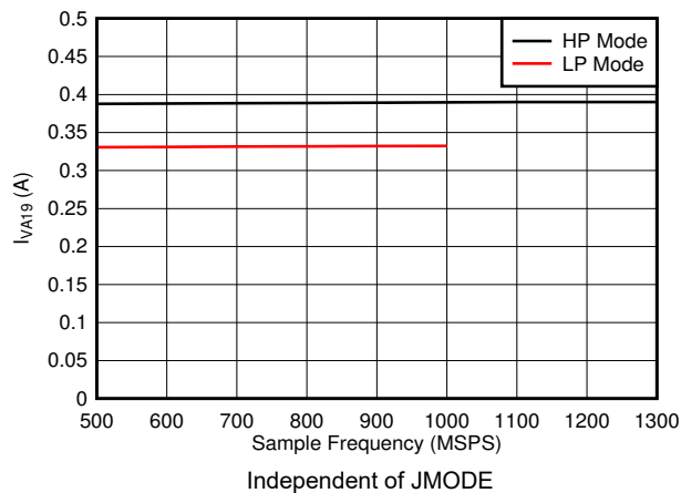
图 5-95. Dual Channel, I_{VA19} vs FS
