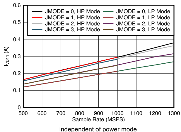
图 5-97. Dual Channel, I_{VD11} vs FS and JMODE 0 - 3
