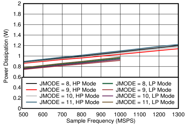
图 5-103. Single Channel, Power Dissipation vs FS for JMODES 8 - 11
