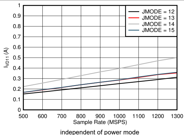
图 5-90. Quad Channel, I_{VD11} vs FS and JMODE 12 - 15
