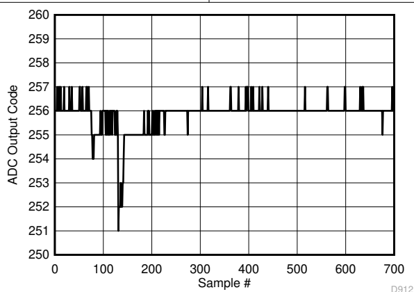
图 5-129. Background Calibration Core Transition (DC Signal)
