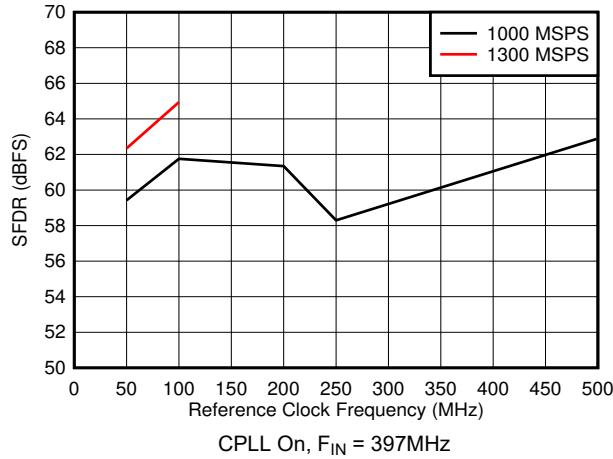
图 5-61. SFDR vs Reference Clock Frequency
