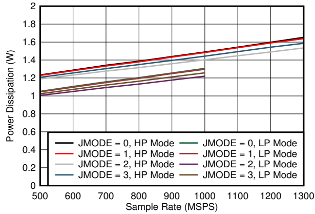
图 5-91. Dual Channel, Power Dissipation vs FS for JMODES 0 - 3
