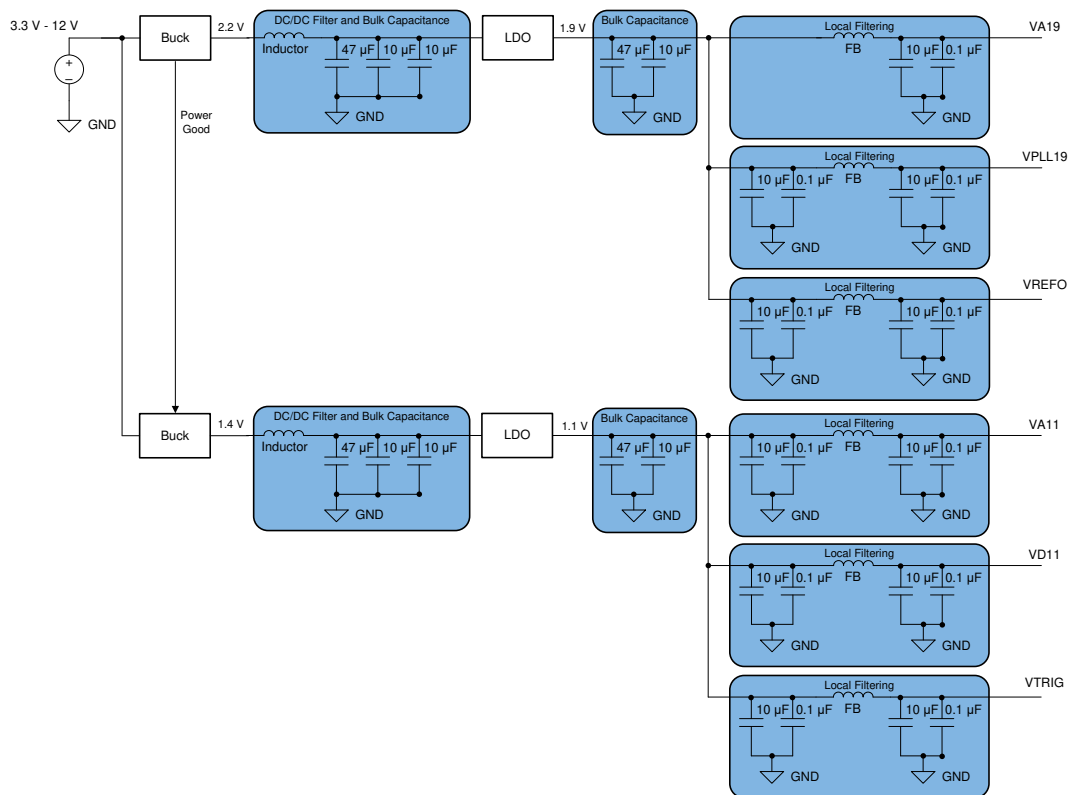
图 7-4. LDO Linear Regulator Approach Example
