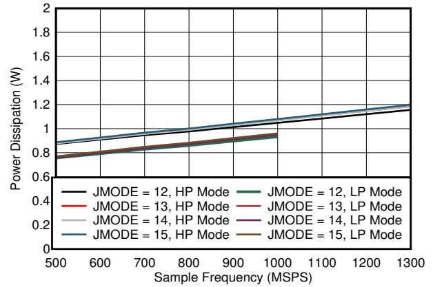
图 5-104. Single Channel, Power Dissipation vs FS for JMODES 12 - 15
