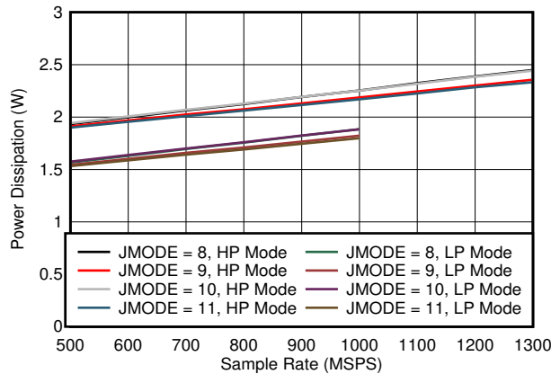
图 5-83. Quad Channel, Power Dissipation vs FS for JMODES 8 - 11
