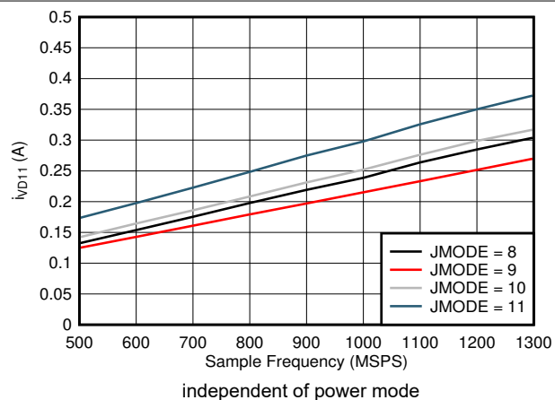
图 5-99. Dual Channel, I_{VD11} vs FS and JMODE 8 - 11
