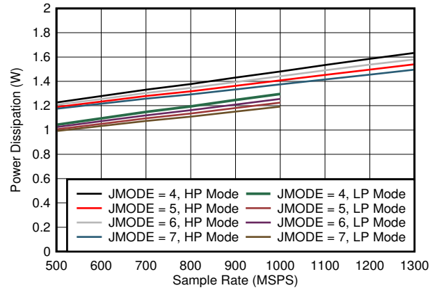
图 5-92. Dual Channel, Power Dissipation vs FS for JMODES 4 - 7
