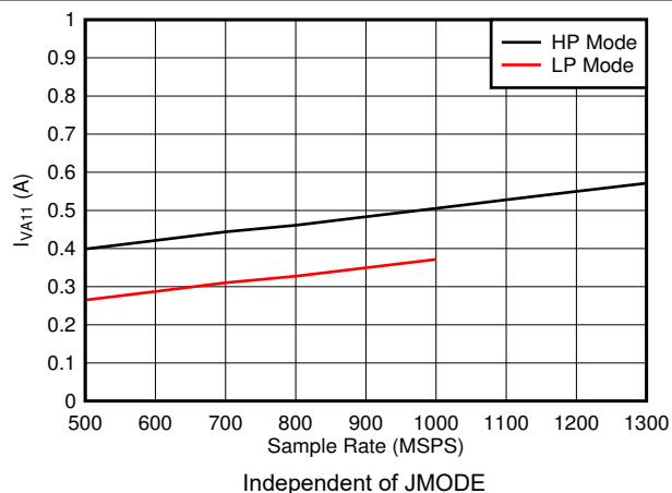
图 5-86. Quad Channel, I_{VA11} vs FS
