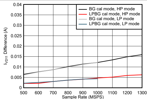
图 5-122. Dual Channel, I_{VD11} Change with Calibration Mode
