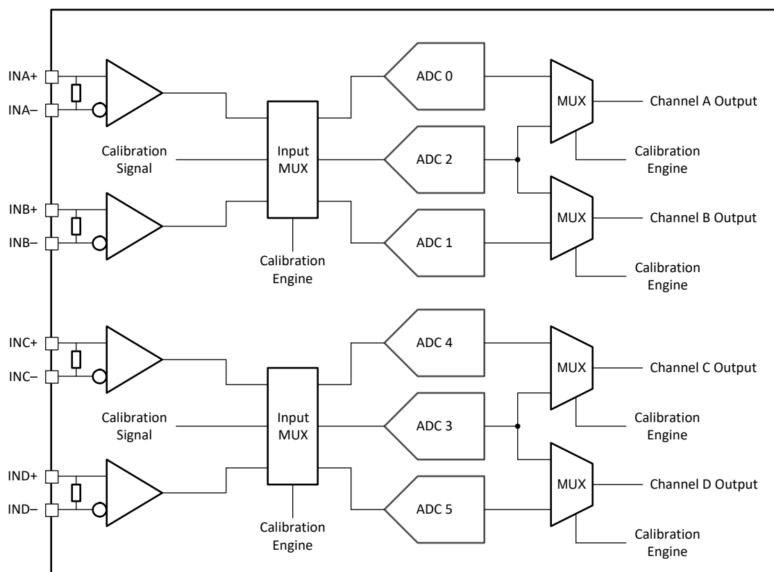
图 6-15. Quad Channel Calibration System Block Diagram
