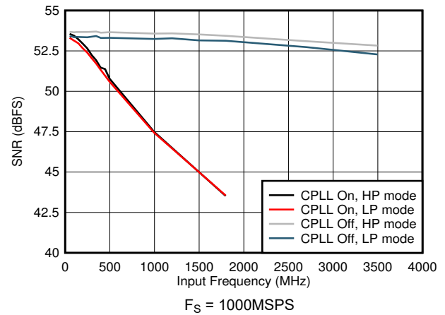
图 5-66. SNR vs Input Frequency and CPLL
