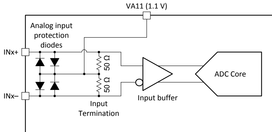
图 6-4. Analog Input Internal Termination and Protection Diagram
