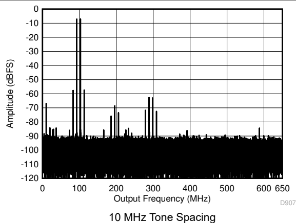
图 5-53. Two Tone FFT at 2698 MHz Center
