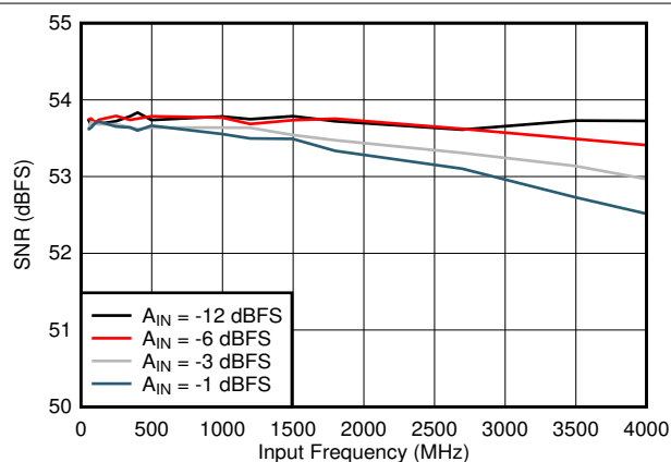
图 5-16. SNR vs Input Frequency
