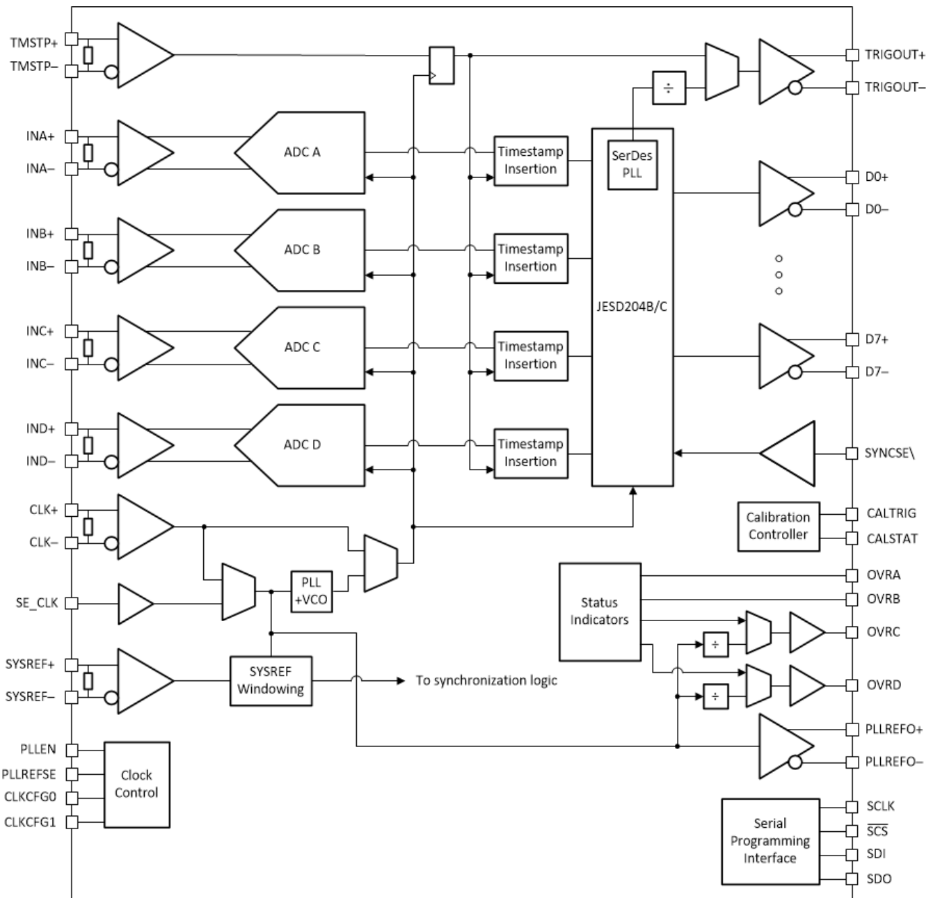
图 6-1. Quad Channel Functional Block Diagram
