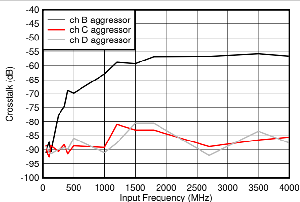
图 5-59. Crosstalk to Channel A vs F_{IN}
