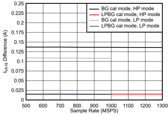
图 5-115. Dual Channel, I_{VA19} Change with Calibration Mode
