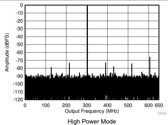
图 5-6. Single Tone FFT at 997 MHz and -1 dBFS
