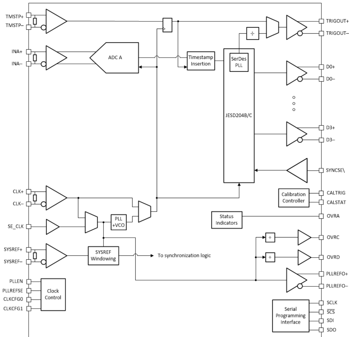
图 6-3. Single Channel Functional Block Diagram
