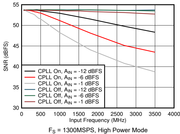
图 5-69. SNR vs Input Frequency, CPLL and Input Amplitude
