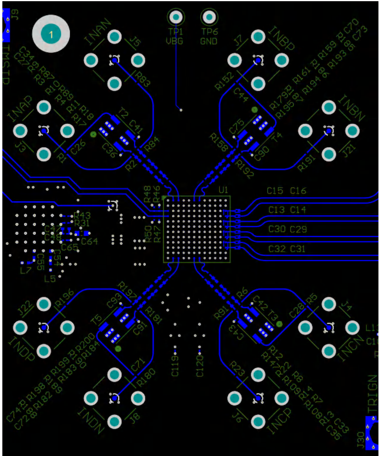
图 7-6. Top Layer Routing: Analog Inputs (INA±, INB±, INC±, IND±), TMSTP± and D[3:0]± Routing
