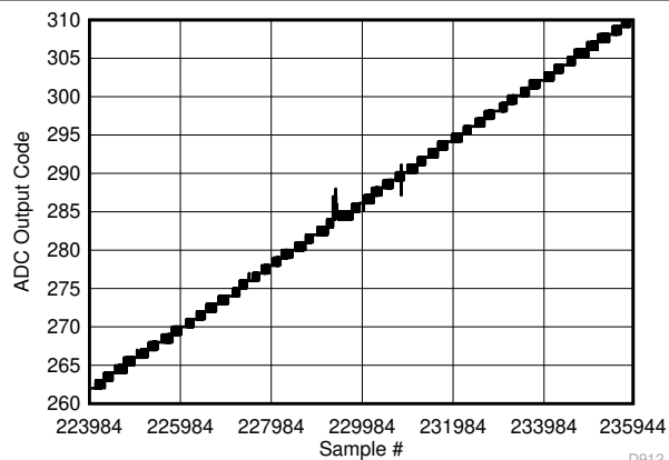
图 5-128. Background Calibration Core Transition (AC Signal Zoomed)
