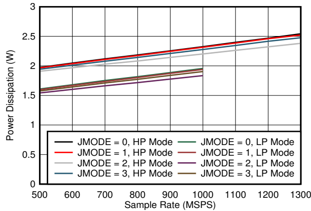
图 5-81. Quad Channel, Power Dissipation vs FS for JMODES 0 - 3
