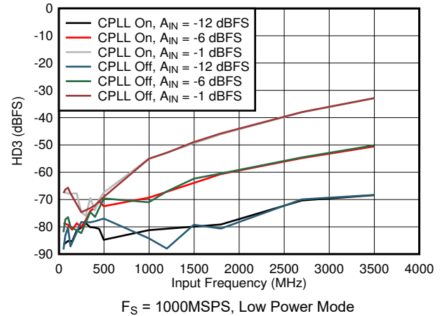
图 5-80. HD3 vs Input Frequency, CPLL and Input Amplitude
