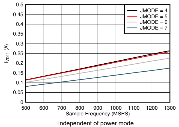
图 5-108. Single Channel, I_{VD11} vs FS and JMODE 4 - 7
