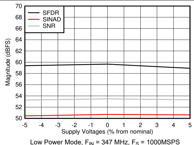
图 5-46. SNR, SFDR and SINAD vs Supply Voltage
