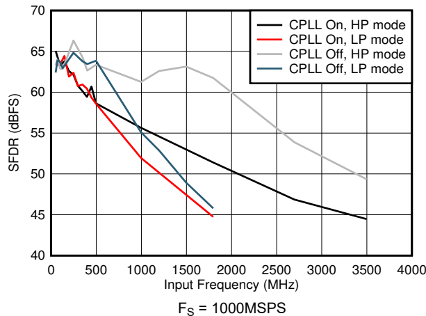
图 5-65. SFDR vs Input Frequency and CPLL
