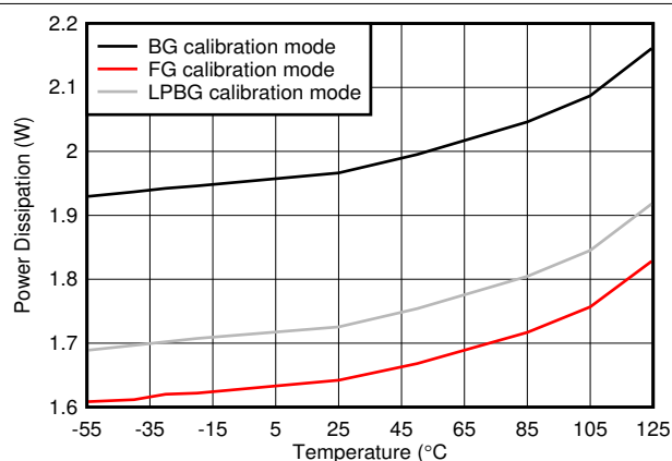
图 5-124. Dual Channel, Power Dissipation vs Temperature
