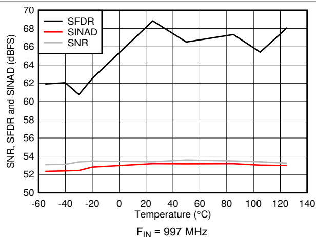
图 5-35. SNR, SFDR and SINAD vs Temperature
