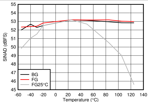
图 5-37. SINAD vs Temperature and Calibration Mode
