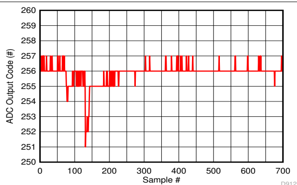
图 5-126. Background Calibration Core Transition (midscale voltage)
