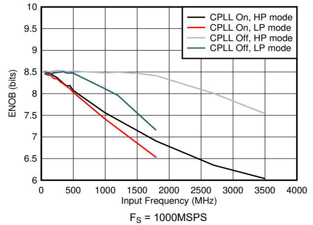
图 5-68. ENOB vs Input Frequency and CPLL
