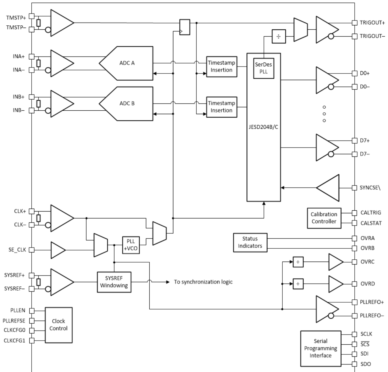
图 6-2. Dual Channel Functional Block Diagram
