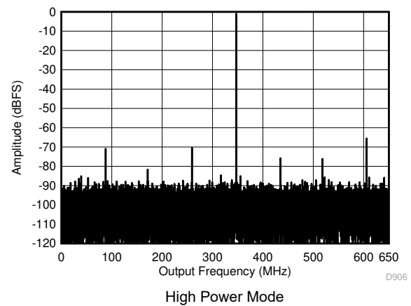
图 5-4. Single Tone FFT at 347 MHz and -1 dBFS
