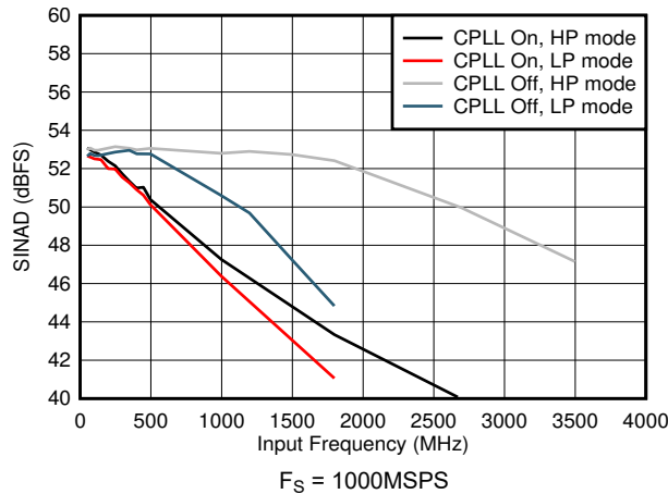
图 5-67. SINAD vs Input Frequency and CPLL
