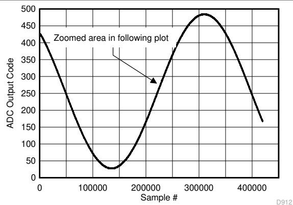
图 5-127. Background Calibration Core Transition (AC Signal)
