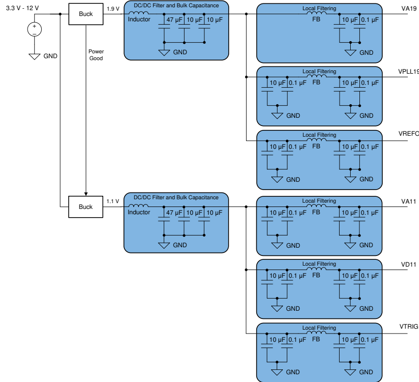
图 7-5. Switcher-Only Approach Example
