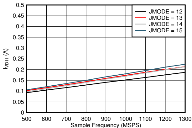
图 5-110. Single Channel, I_{VD11} vs FS and JMODE 12 - 15
