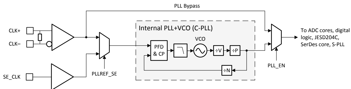
图 6-6. Converter PLL (C-PLL) Architecture
