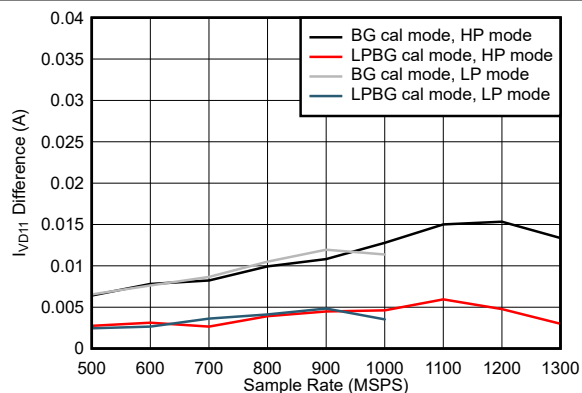
图 5-121. Dual Channel, I_{VD11} Change with Calibration Mode
