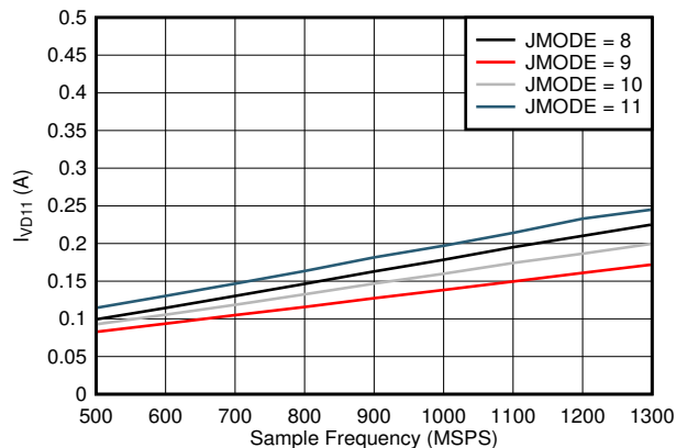
图 5-109. Single Channel, I_{VD11} vs FS and JMODE 8 - 11
