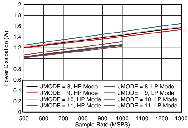
图 5-93. Dual Channel, Power Dissipation vs FS for JMODES 8 - 11
