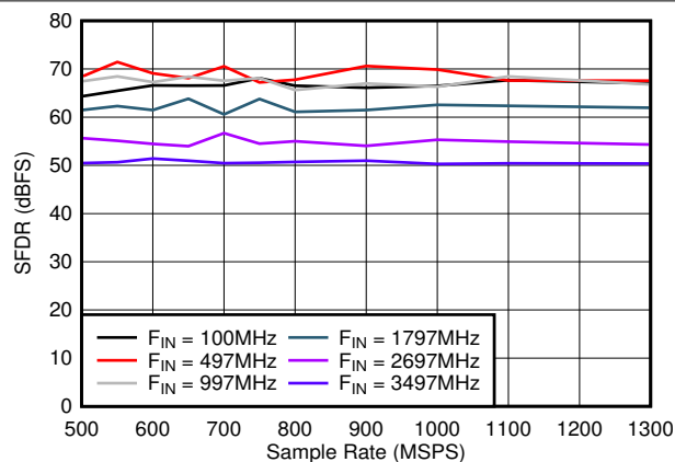
图 5-21. SFDR vs Sample Rate
