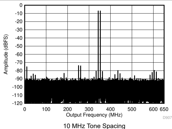
图 5-49. Two Tone FFT at 348 MHz Center
