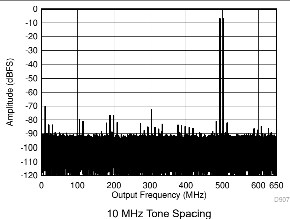
图 5-50. Two Tone FFT at 498 MHz Center
