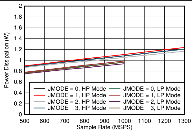
图 5-101. Single Channel, Power Dissipation vs FS for JMODES 0 - 3
