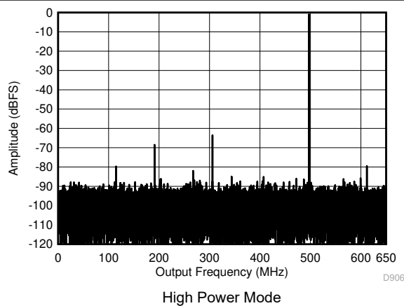
图 5-5. Single Tone FFT at 497 MHz and -1 dBFS
