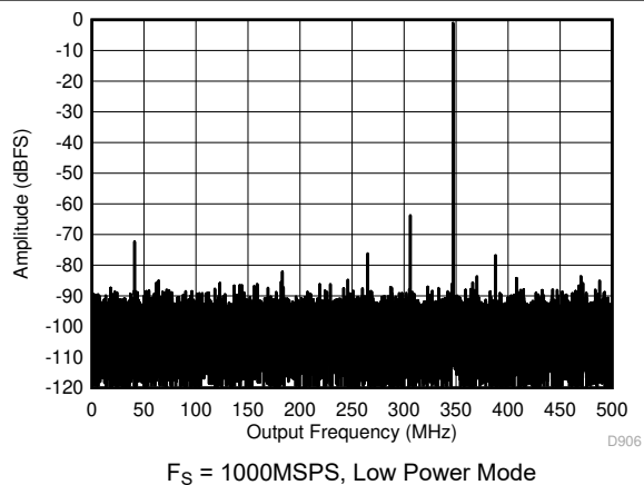
图 5-12. Single Tone FFT at 347 MHz and -1 dBFS
