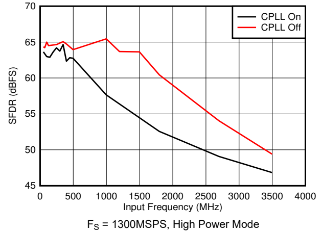
图 5-62. SFDR vs Input Frequency and CPLL
