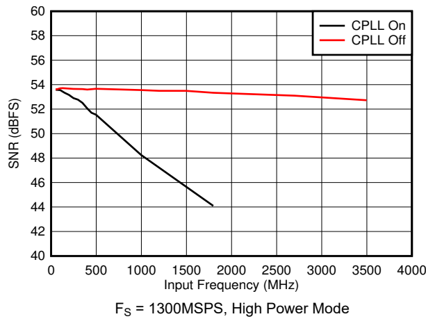
图 5-63. SNR vs Input Frequency and CPLL
