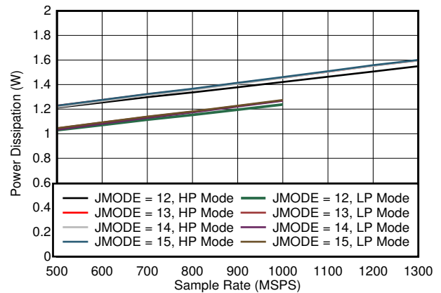
图 5-94. Dual Channel, Power Dissipation vs FS for JMODES 12 - 15
