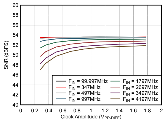
图 5-34. SNR vs Clock Amplitude
