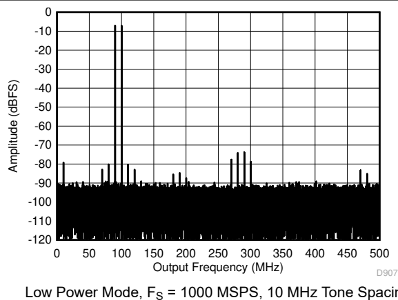
图 5-54. Two Tone FFT at 95.07 MHz Center
