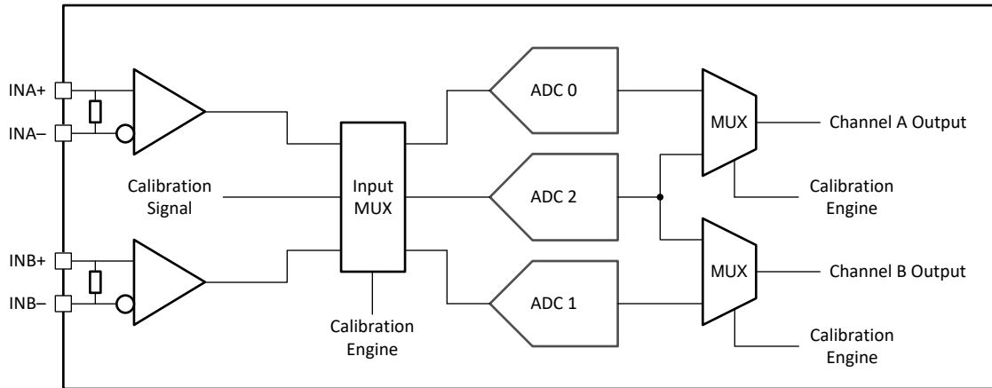
图 6-16. DualChannel Calibration System Block Diagram
