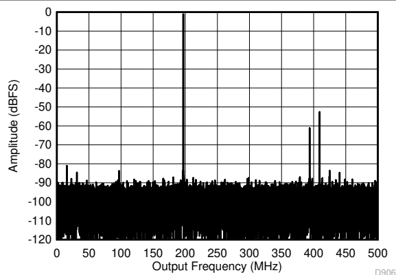
图 5-13. Single Tone FFT at 1197 MHz and -1 dBFS
