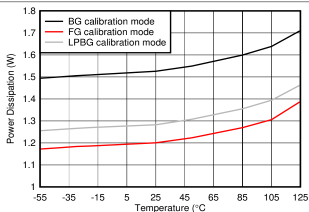
图 5-125. Single Channel, Power Dissipation vs Temperature
