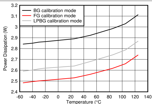
图 5-123. Quad Channel, Power Dissipation vs Temperature
