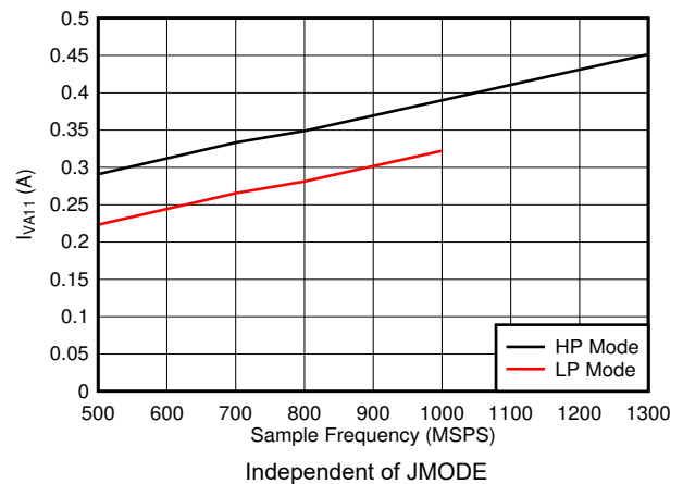
图 5-96. Dual Channel, I_{VA11} vs FS
