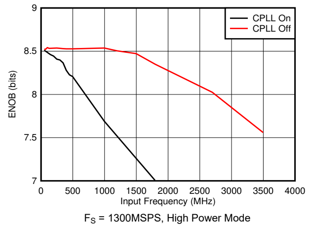
图 5-64. ENOB vs Input Frequency and CPLL
