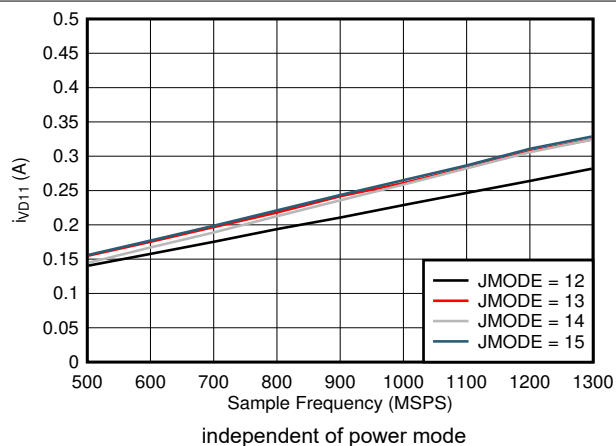
图 5-100. Dual Channel, I_{VD11} vs FS and JMODE 12 - 15
