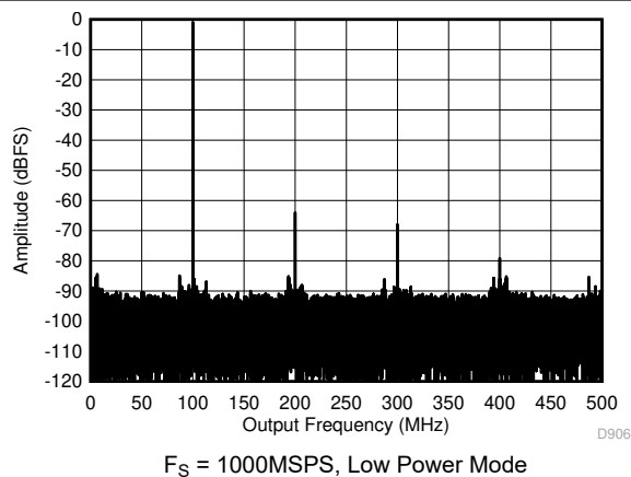
图 5-11. Single Tone FFT at 99.997 MHz and -1 dBFS
