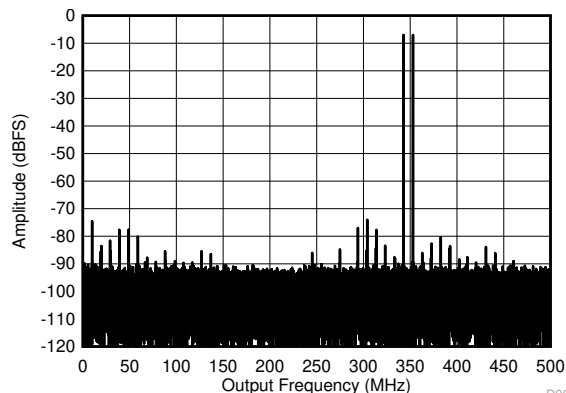
图 5-55. Two Tone FFT at 348 MHz Center
