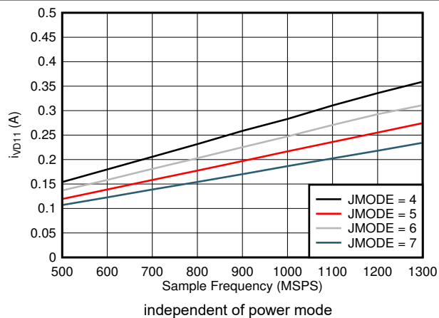
图 5-98. Dual Channel, I_{VD11} vs FS and JMODE 4 - 7
