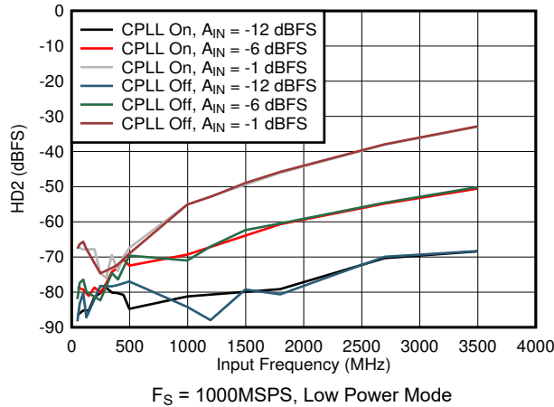
图 5-79. HD2 vs Input Frequency, CPLL and Input Amplitude
