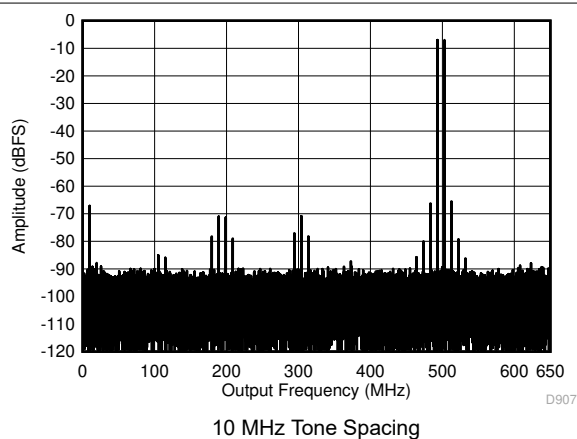
图 5-52. Two Tone FFT at 1798 MHz Center
