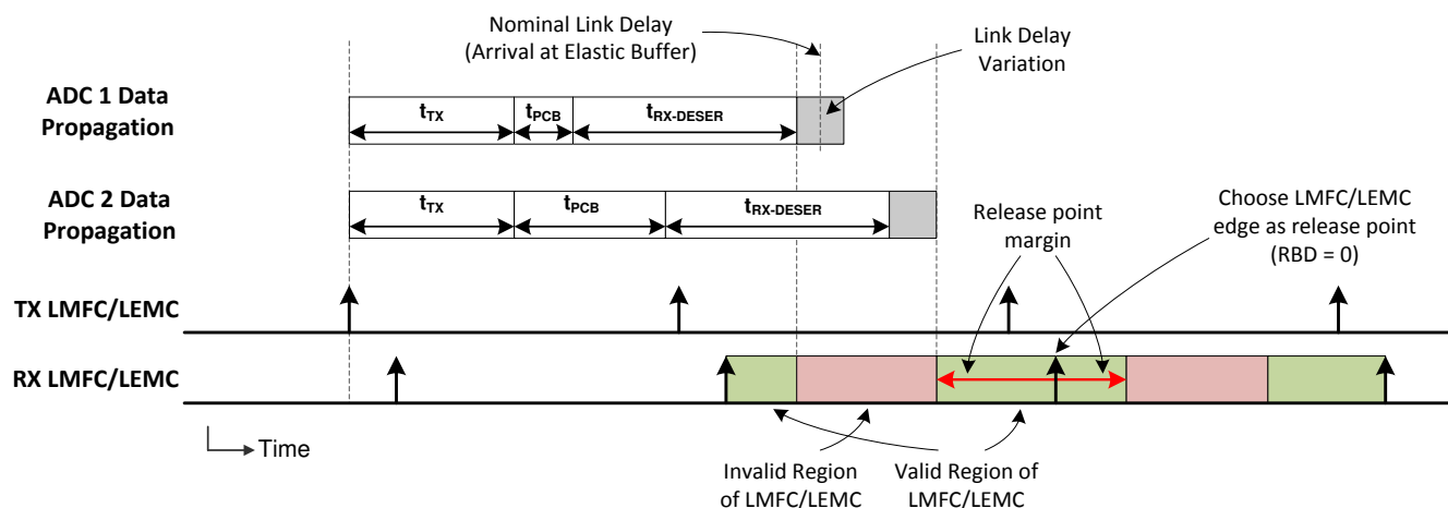
图 6-11. LMFC/LEMC Valid Region Definition for Elastic Buffer Release Point Selection
