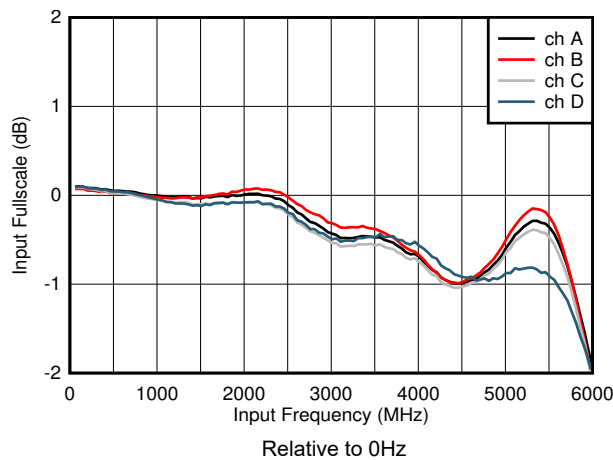
图 5-3. Input Fullscale vs Input Frequency
