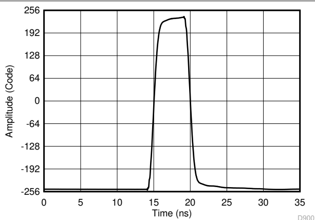
图 7-2. Measured Pulse using Sub-Sampling Technique for Equivalent 32 GSPS Measurement
