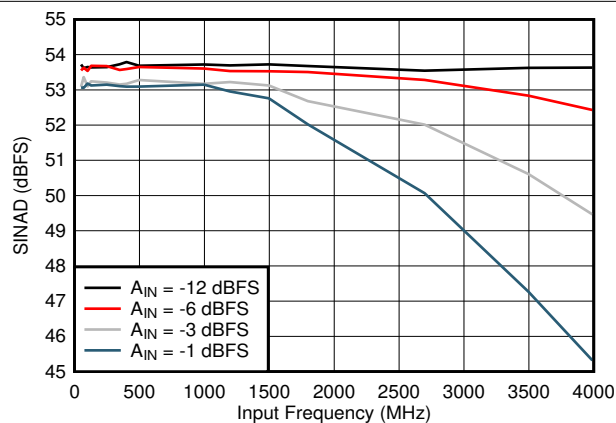
图 5-17. SINAD vs Input Frequency
