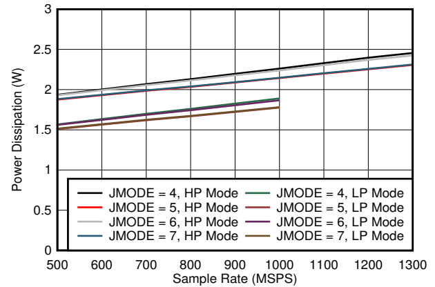
图 5-82. Quad Channel, Power Dissipation vs FS for JMODES 4 - 7
