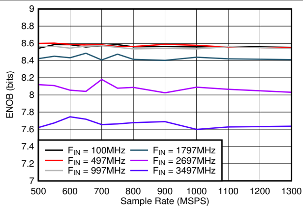
图 5-24. ENOB vs Sample Rate
