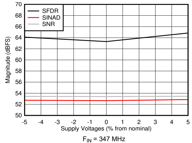
图 5-44. SNR, SFDR and SINAD vs Supply Voltage
