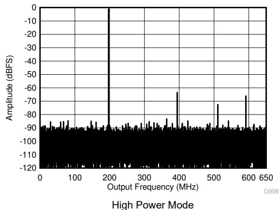
图 5-7. Single Tone FFT at 1497 MHz and -1 dBFS
