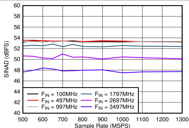
图 5-23. SINAD vs Sample Rate
