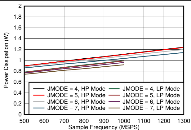
图 5-102. Single Channel, Power Dissipation vs FS for JMODES 4 - 7
