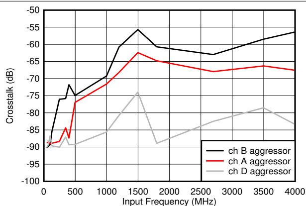
图 5-60. Crosstalk to Channel B vs F_{IN}
