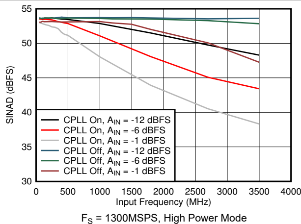
图 5-71. SINAD vs Input Frequency, CPLL and Input Amplitude
