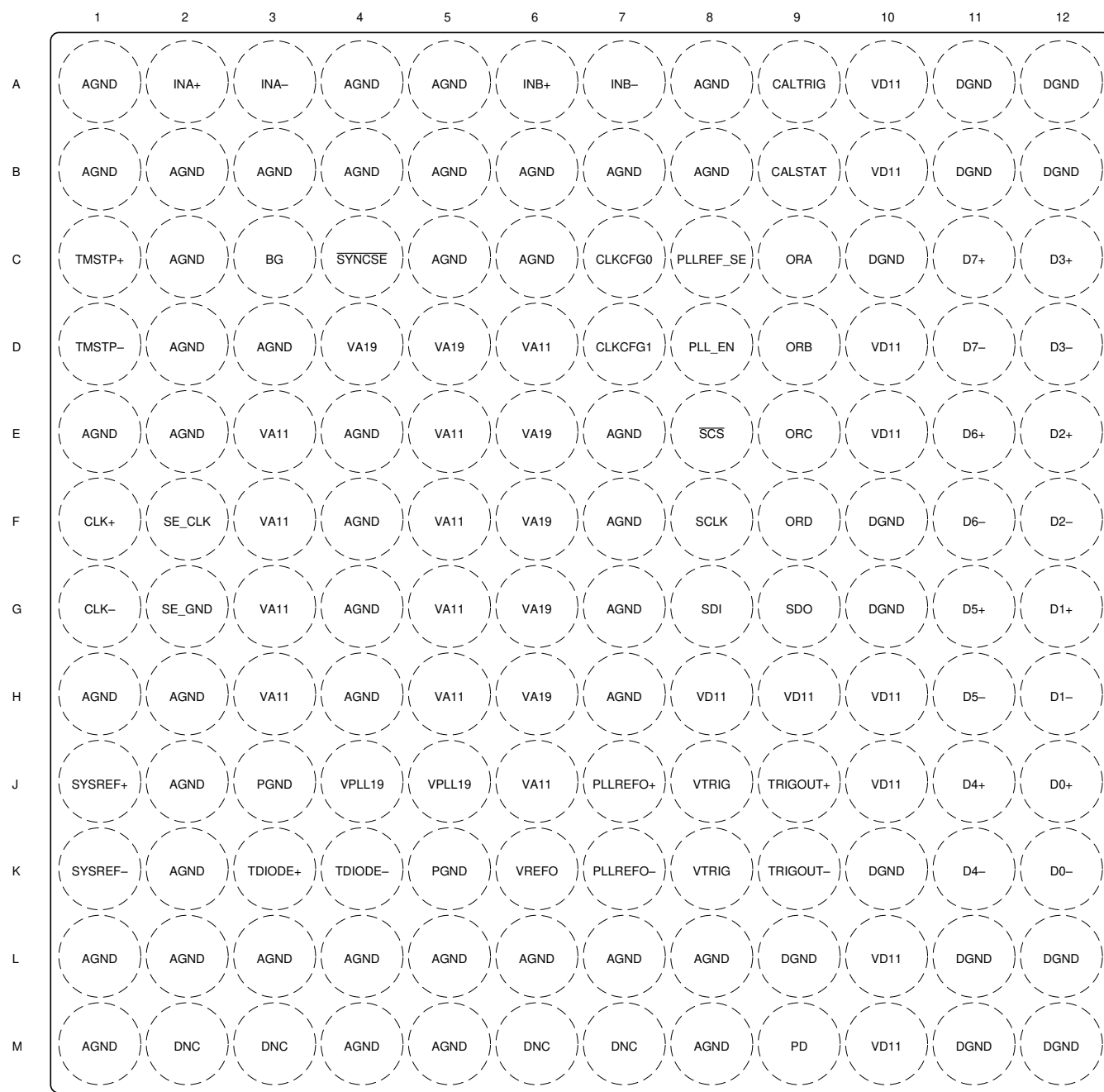
图 4-2. Dual Channel AAV Package, 144-Ball Flip Chip BGA (Top View)
