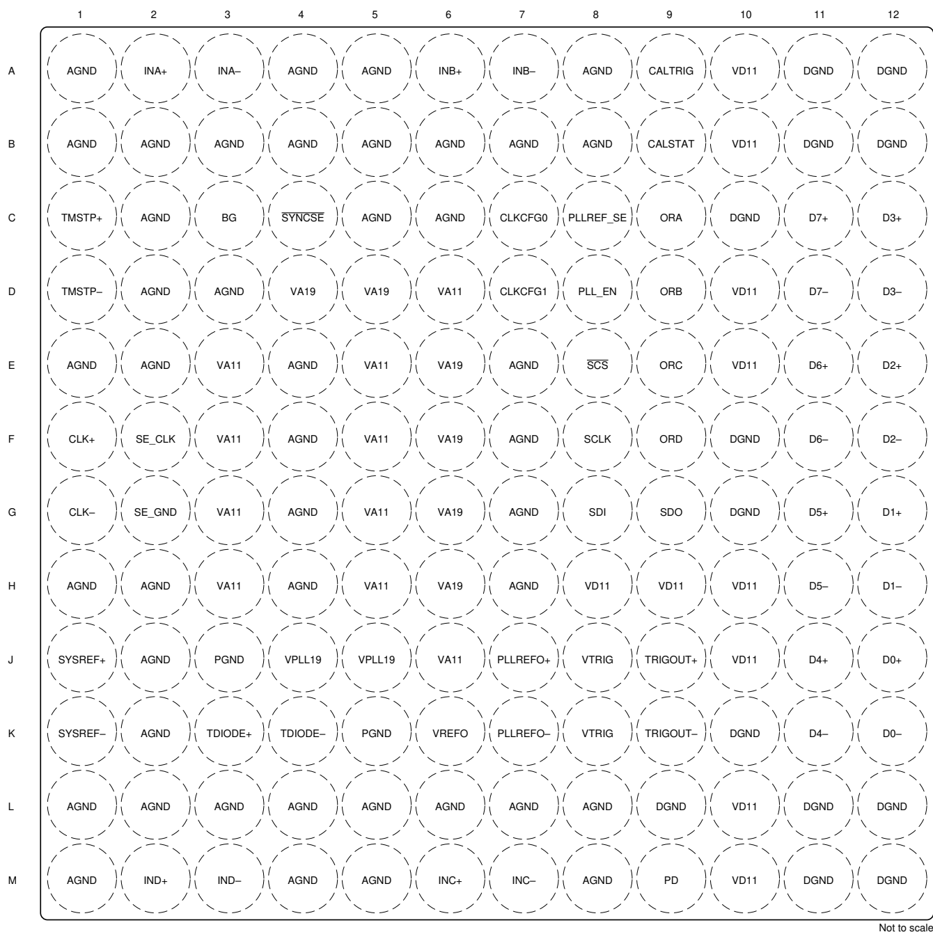
图 4-1. Quad Channel AAV Package, 144-Ball Flip Chip BGA (Top View)
