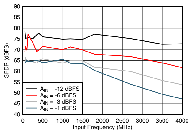
图 5-15. SFDR vs Input Frequency
