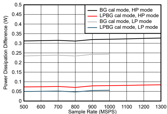
图 5-111. Quad Channel, Power Dissipation Change with Calibration Mode
