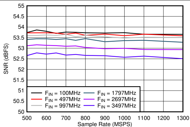
图 5-22. SNR vs Sample Rate
