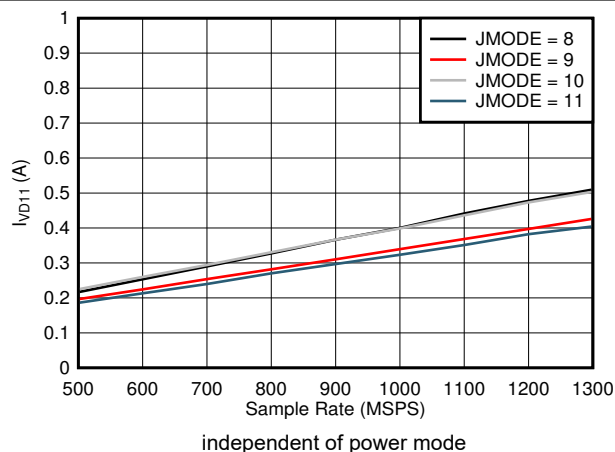
图 5-89. Quad Channel, I_{VD11} vs FS and JMODE 8 - 11
