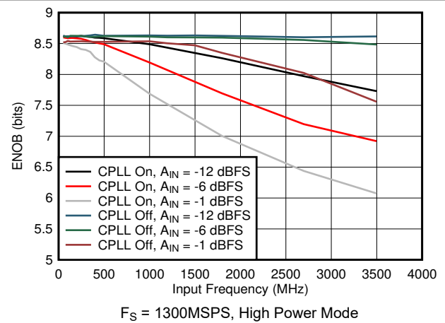
图 5-72. ENOB vs Input Frequency, CPLL and Input Amplitude
