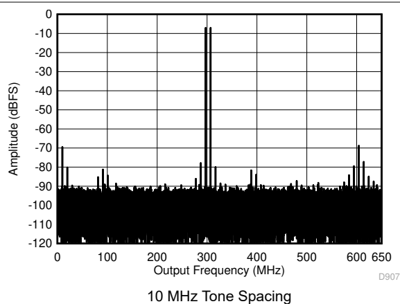
图 5-51. Two Tone FFT at 998 MHz Center
