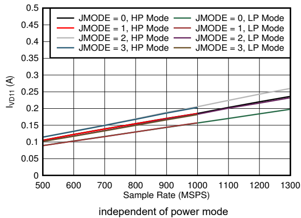
图 5-107. Single Channel, I_{VD11} vs FS and JMODE 0 - 3
