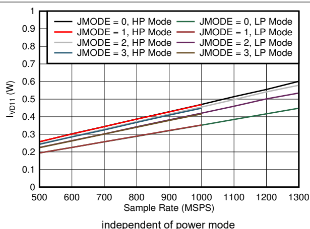
图 5-87. Quad Channel, I_{VD11} vs FS and JMODE 0 - 3
