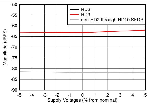
图 5-45. HD2, HD3 and Worst non-HD Spur vs Supply Voltage
