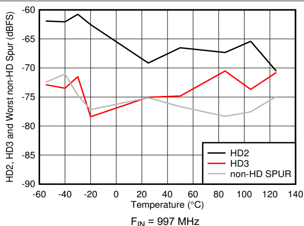
图 5-36. HD2, HD3 and worst non-HD Spur vs Temperature
