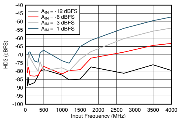
图 5-20. HD3 vs Input Frequency
