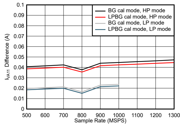
图 5-117. Quad Channel, I_{VA11} Change with Calibration Mode
