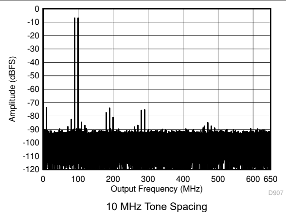
图 5-48. Two Tone FFT at 95.07 MHz Center
