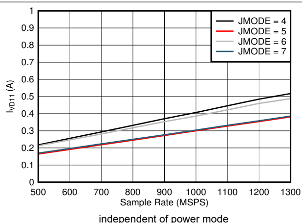
图 5-88. Quad Channel, I_{VD11} vs FS and JMODE 4 - 7
