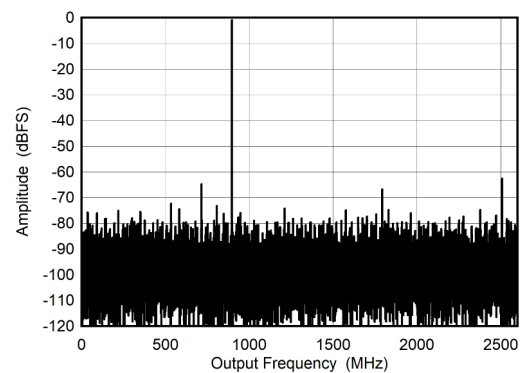
图 5-18. Dual Channel Mode: Single Tone FFT at 897 MHz
