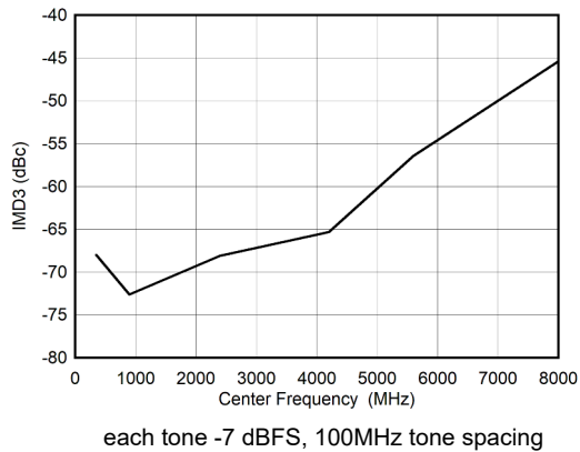
图 5-105. Dual Channel Mode: IMD3 vs Input Frequency
