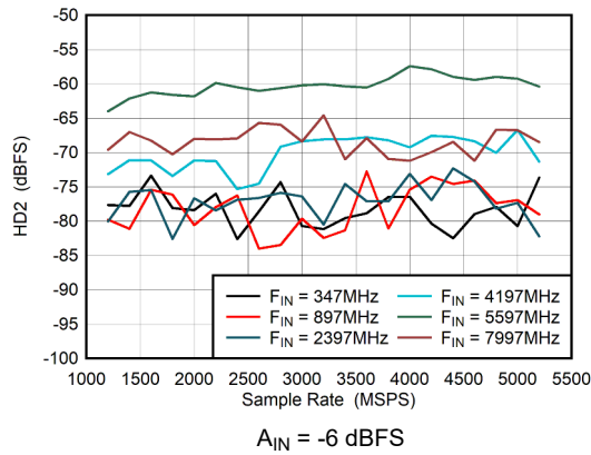
图 5-51. Dual Channel Mode: HD2 vs Sample Rate
