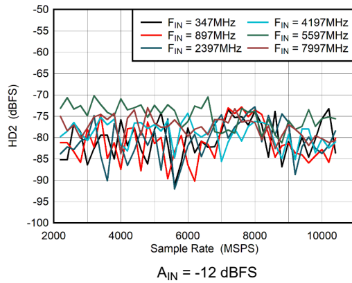
图 5-37. DES Mode: HD2 vs Sample Rate
