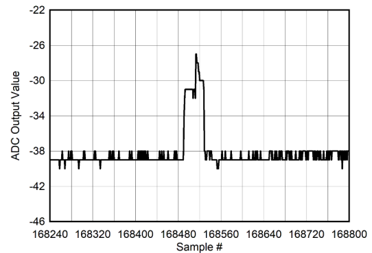
图 5-120. Background Calibration Core Transition (AC Signal Zoomed)
