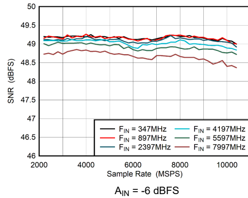
图 5-30. DES Mode: SNR vs Sample Rate
