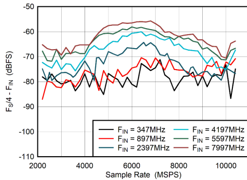
图 5-43. DES Mode: F_S/4 - F_{\text{IN}} vs Sample Rate
