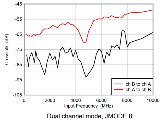
图 5-2. Crosstalk vs Input Frequency
