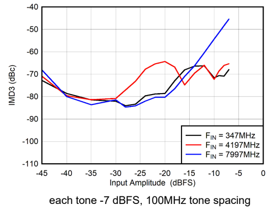
图 5-106. Dual Channel Mode: IMD3 vs Input Amplitude
