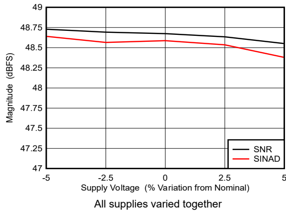
图 5-95. Dual Channel Mode: SNR and SINAD vs Supply Voltage
