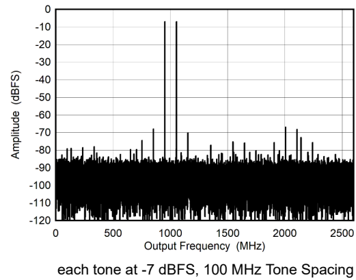
图 5-26. Dual Channel Mode: Two Tone FFT at 4197 MHz
