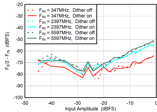
图 5-66. DES Mode: F_{S/2} - F_{\text{IN}} vs Input Amplitude and Dither
