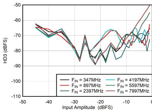
图 5-77. Dual Channel Mode: HD3 vs Input Amplitude
