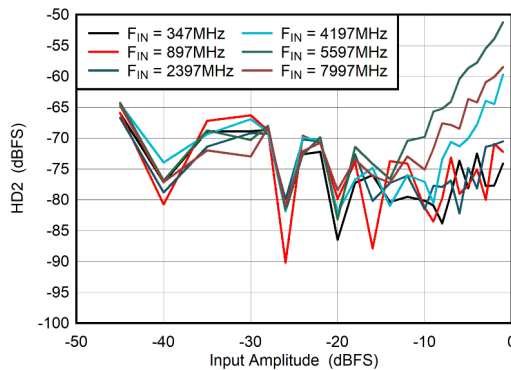
图 5-75. Dual Channel Mode: HD2 vs Input Amplitude
