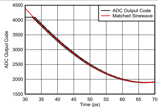
图 5-126. Sinewave Overdrive Recovery
