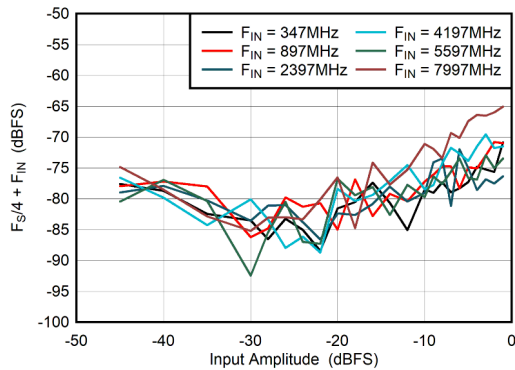
图 5-67. DES Mode: F_s/4 + F_{\text{IN}} vs Input Amplitude
