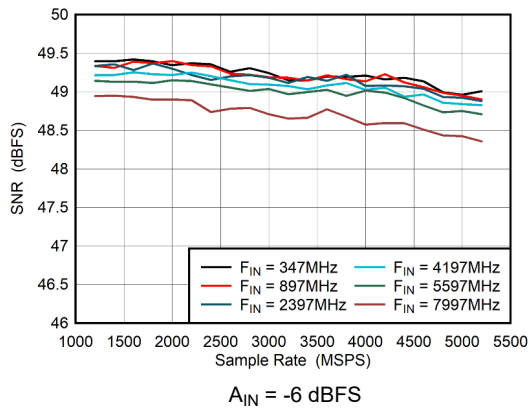
图 5-45. Dual Channel Mode: SNR vs Sample Rate
