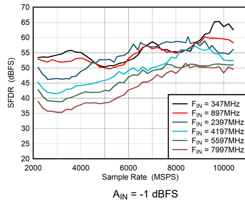
图 5-32. DES Mode: SFDR vs Sample Rate
