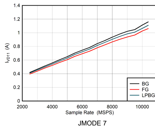
图 5-112. DES Mode: I_{VD11} vs Sample Rate
