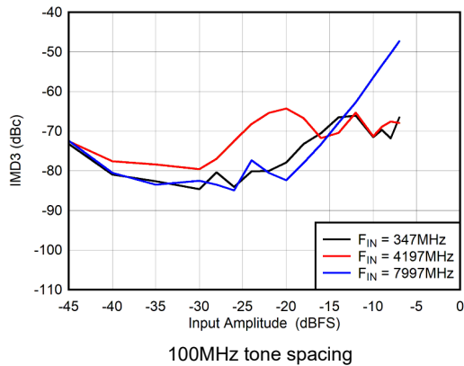
图 5-101. DES Mode: IMD3 vs Input Amplitude
