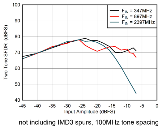
图 5-109. Dual Channel Mode: Two Tone SFDR vs Input Amplitude
