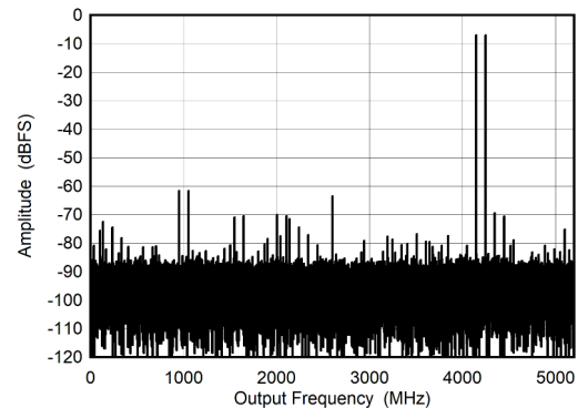
图 5-14. DES Mode: Two Tone FFT at 4197 MHz
