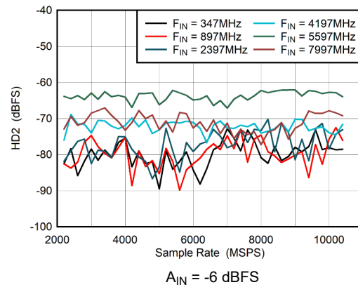
图 5-36. DES Mode: HD2 vs Sample Rate
