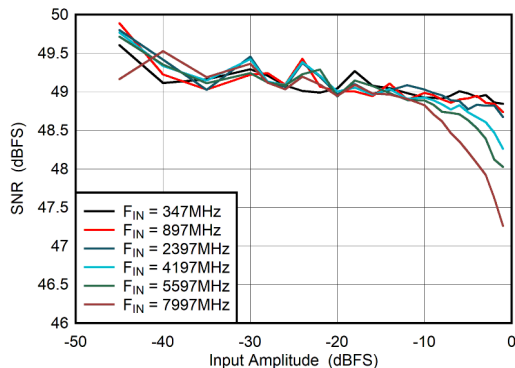
图 5-71. Dual Channel Mode: SNR vs Input Amplitude
