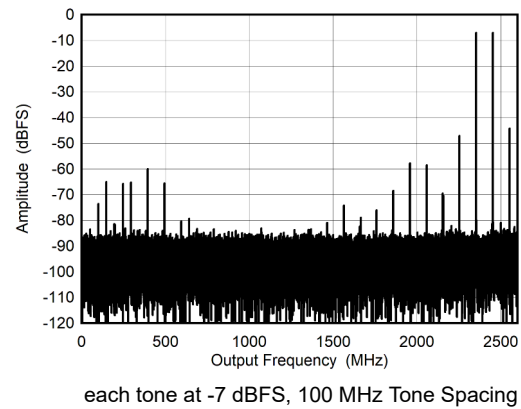
图 5-28. Dual Channel Mode: Two Tone FFT at 7997 MHz
