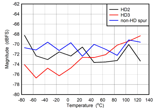
图 5-90. Dual Channel Mode: HD2, HD3 and Worst Spur vs Temperature
