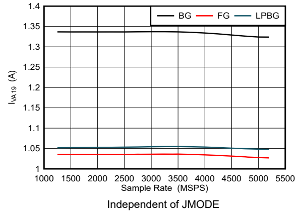
图 5-114. Dual Channel Mode: I_{VA19} vs Sample Rate
