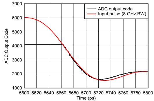
图 5-124. Pulse Overdrive Recovery Zoomed
