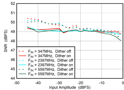
图 5-58. DES Mode: SNR vs Input Amplitude and Dither
