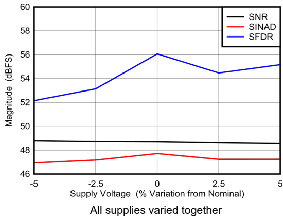
图 5-93. DES Mode: SNR, SINAD and SFDR vs Supply Voltage
