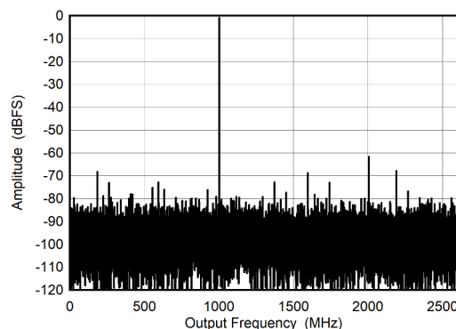
图 5-20. Dual Channel Mode: Single Tone FFT at 4197 MHz
