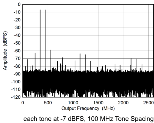
图 5-27. Dual Channel Mode: Two Tone FFT at 5597 MHz
