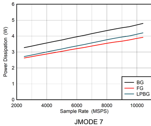
图 5-113. DES Mode: Power Dissipation vs Sample Rate
