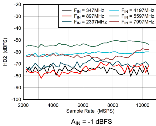
图 5-35. DES Mode: HD2 vs Sample Rate
