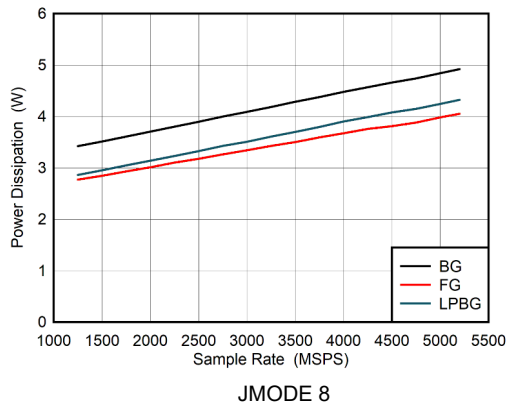
图 5-117. Dual Channel Mode: Power Dissipation vs Sample Rate
