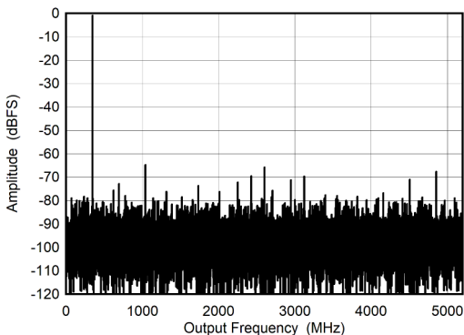
图 5-5. DES Mode: Single Tone FFT at 347 MHz
