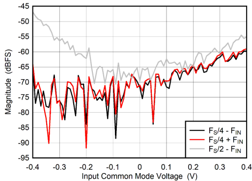
图 5-99. DES Mode: F_S/2 - F_{\text{IN}} , F_S/4 \pm F_{\text{IN}} vs Input Common Mode Voltage
