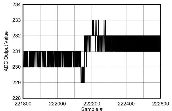
图 5-122. Background Calibration Core Transition (DC Signal Zoomed)
