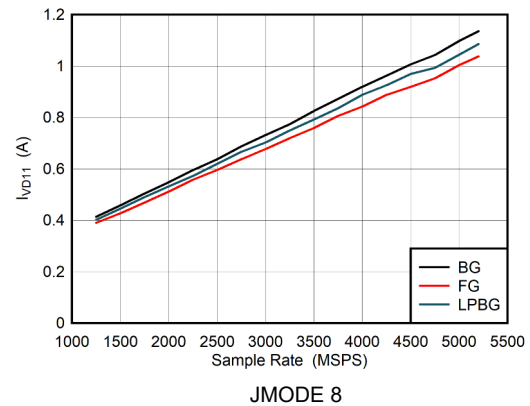
图 5-116. Dual Channel Mode: I_{VD11} vs Sample Rate
