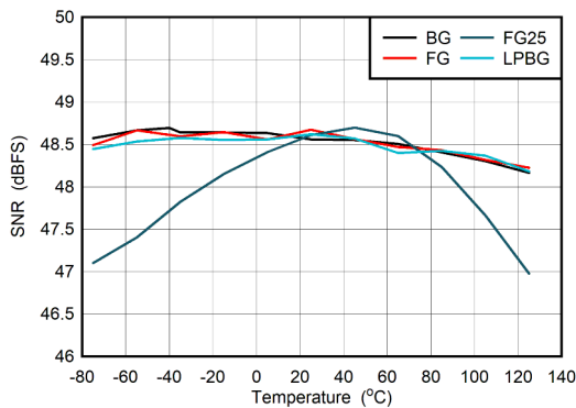
图 5-89. Dual Channel Mode: SNR, SINAD and SFDR vs Temperature
