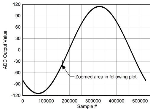
图 5-119. Background Calibration Core Transition (AC Signal)
