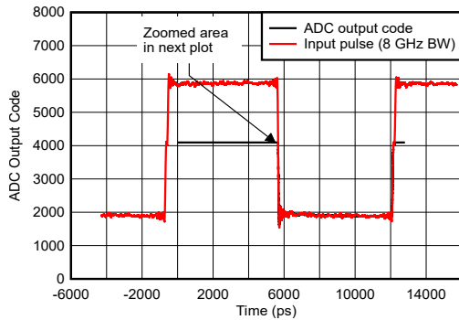
图 5-123. Pulse Overdrive Recovery
