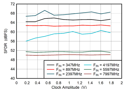
图 5-84. Dual Channel Mode: SFDR vs Clock Amplitude
