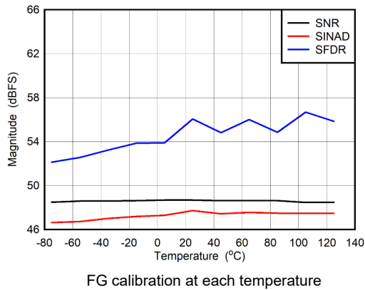
图 5-85. DES Mode: SNR, SINAD and SFDR vs Temperature
