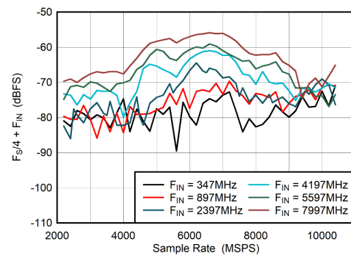
图 5-42. DES Mode: F_S/4 + F_{\text{IN}} vs Sample Rate
