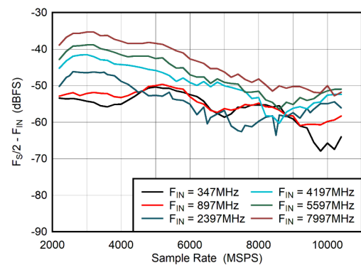
图 5-41. DES Mode: F_S/2 - F_{\text{IN}} vs Sample Rate
