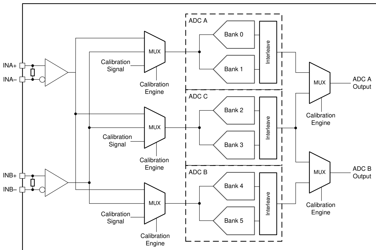
图 6-14. ADC08DJ5200RF Calibration System Block Diagram
