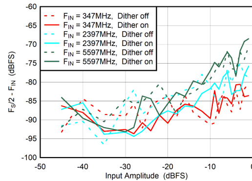
图 5-80. Dual Channel Mode: F_{S/2} - F_{\text{IN}} vs Input Amplitude and Dither
