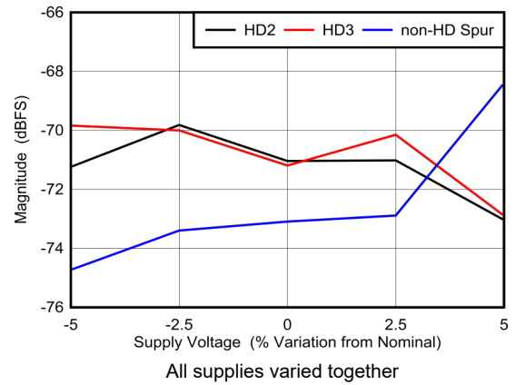
图 5-94. DES Mode: HD2, HD3 and Worst Spur vs Supply Voltage
