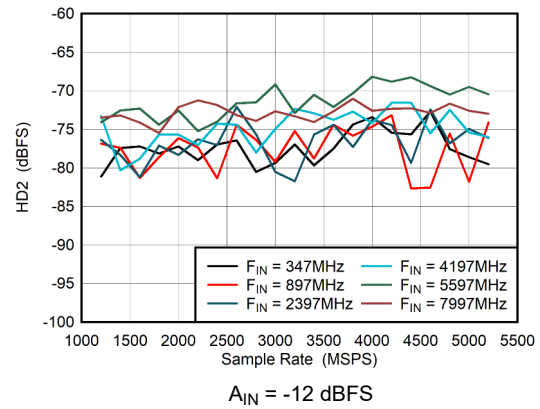
图 5-52. Dual Channel Mode: HD2 vs Sample Rate
