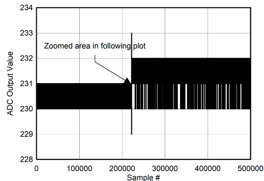
图 5-121. Background Calibration Core Transition (DC Signal)
