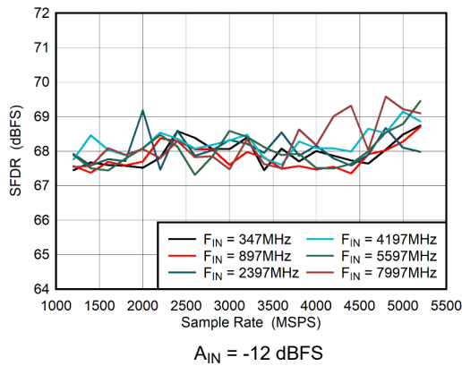
图 5-49. Dual Channel Mode: SFDR vs Sample Rate
