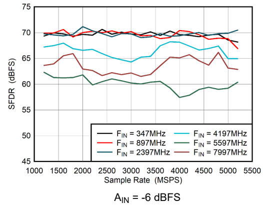
图 5-48. Dual Channel Mode: SFDR vs Sample Rate
