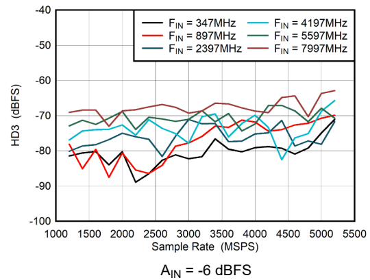
图 5-54. Dual Channel Mode: HD3 vs Sample Rate
