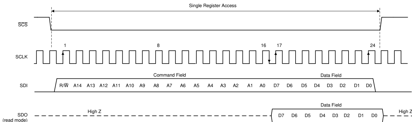
图 6-15. Serial Interface Protocol: Single Read/Write
