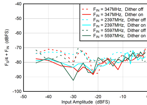
图 5-68. DES Mode: F_s/4 + F_{\text{IN}} vs Input Amplitude and Dither
