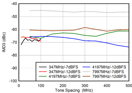
图 5-107. Dual Channel Mode: IMD3 vs Tone Spacing
