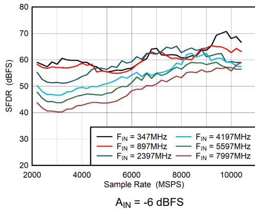
图 5-33. DES Mode: SFDR vs Sample Rate
