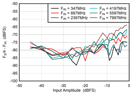
图 5-69. DES Mode: F_s/4 - F_{\text{IN}} vs Input Amplitude
