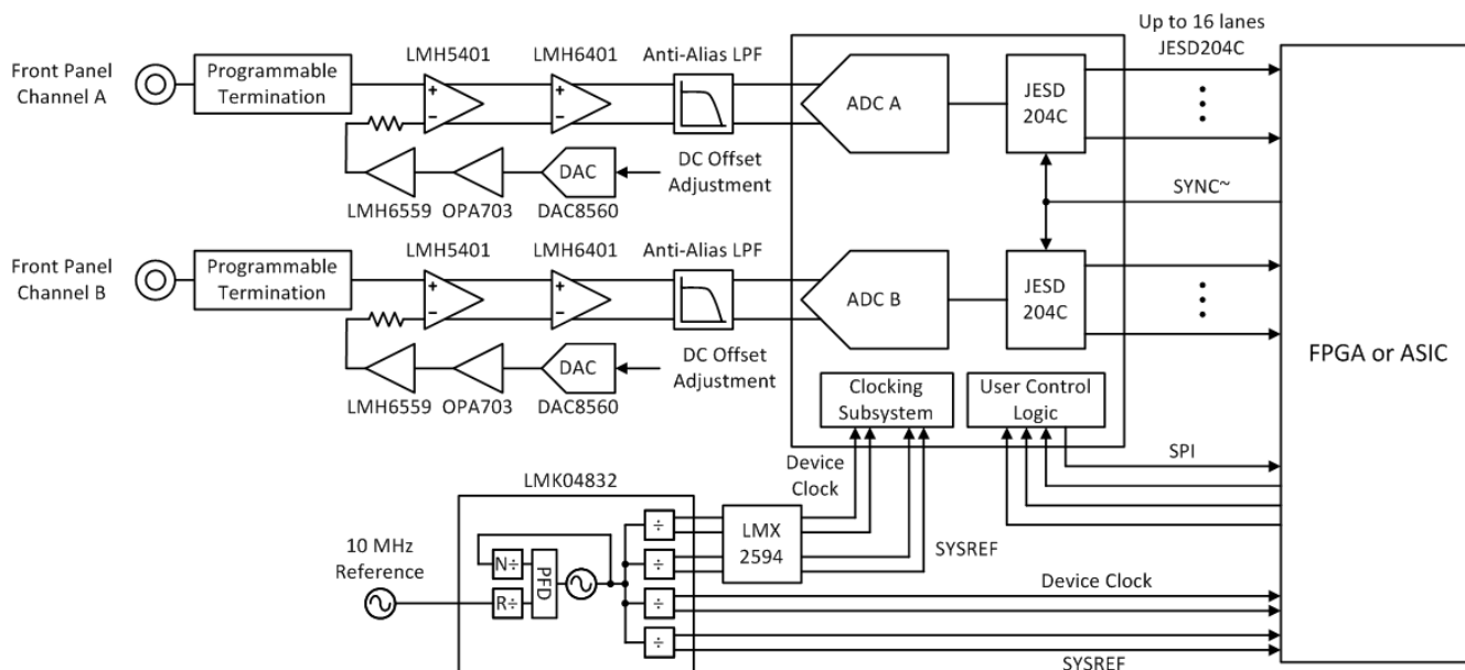
图 7-1. Typical Configuration for Reconfigurable Oscilloscope
