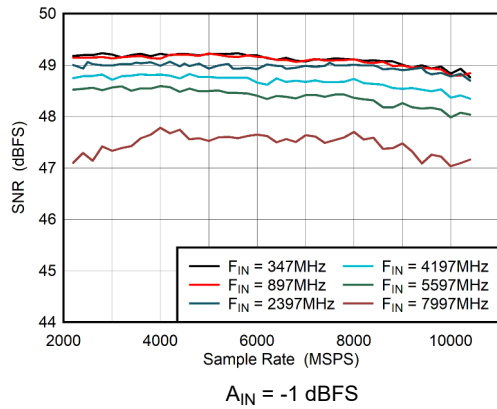
图 5-29. DES Mode: SNR vs Sample Rate
