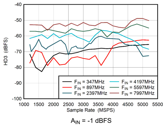
图 5-53. Dual Channel Mode: HD3 vs Sample Rate
