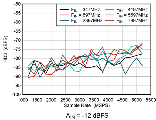
图 5-55. Dual Channel Mode: HD3 vs Sample Rate
