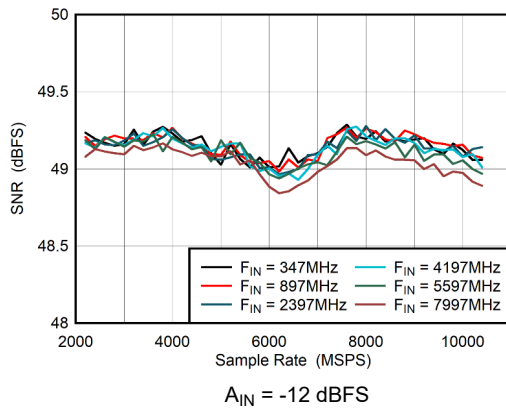
图 5-31. DES Mode: SNR vs Sample Rate
