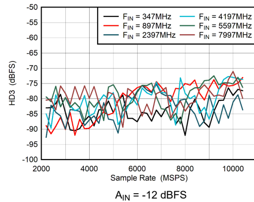
图 5-40. DES Mode: HD3 vs Sample Rate
