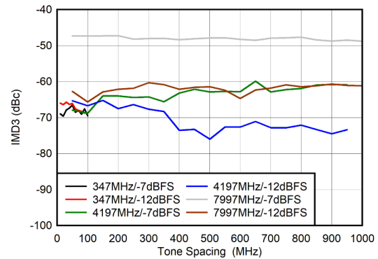
图 5-102. DES Mode: IMD3 vs Tone Spacing
