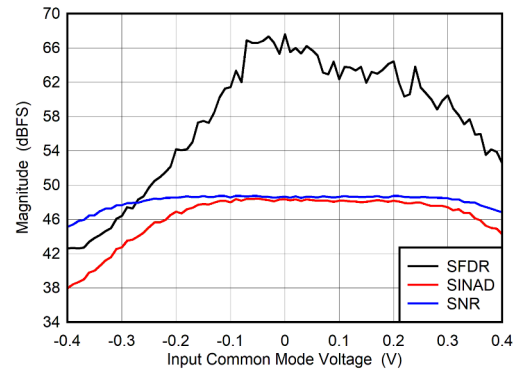
图 5-98. DES Mode: SNR, SFDR and SINAD vs Input Common Mode Voltage
