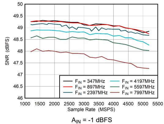
图 5-44. Dual Channel Mode: SNR vs Sample Rate
