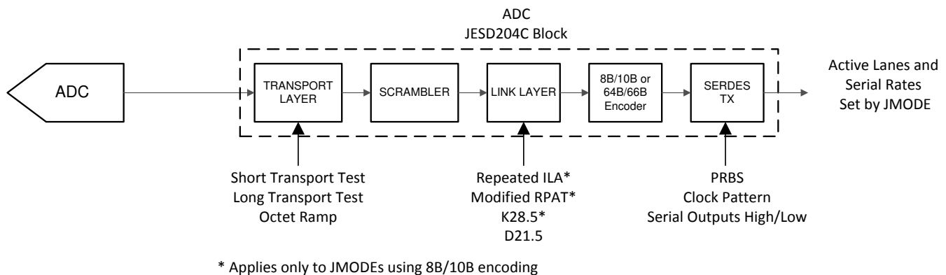
图 6-13. Test Mode Insertion Points
