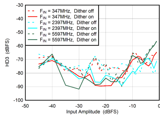
图 5-64. DES Mode: HD3 vs Input Amplitude and Dither
