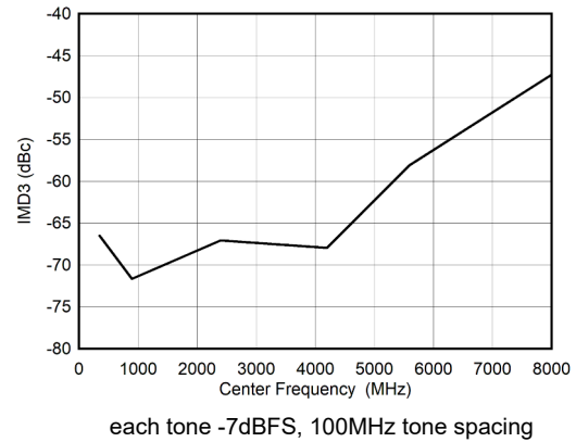
图 5-100. DES Mode: IMD3 vs Input Frequency
