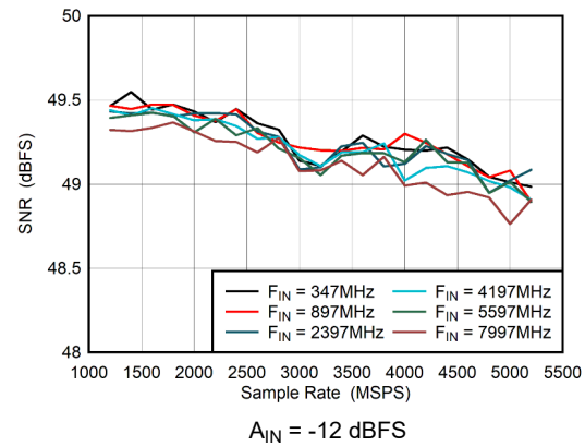
图 5-46. Dual Channel Mode: SNR vs Sample Rate
