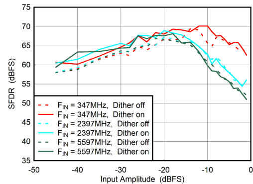
图 5-60. DES Mode: SFDR vs Input Amplitude and Dither
