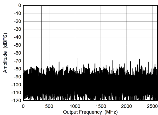
图 5-17. Dual Channel Mode: Single Tone FFT at 347 MHz
