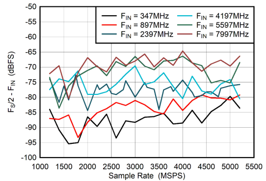
图 5-56. Dual Channel Mode: F_s/2 - F_{\text{IN}} vs Sample Rate
