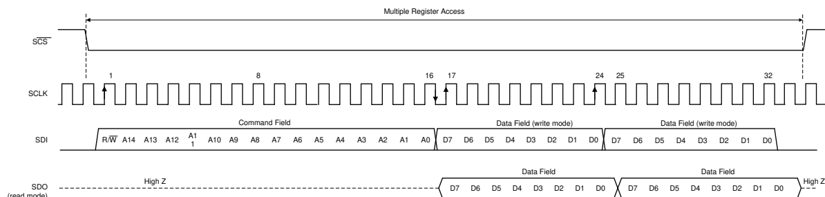
图 6-16. Serial Interface Protocol: Streaming Read/Write
