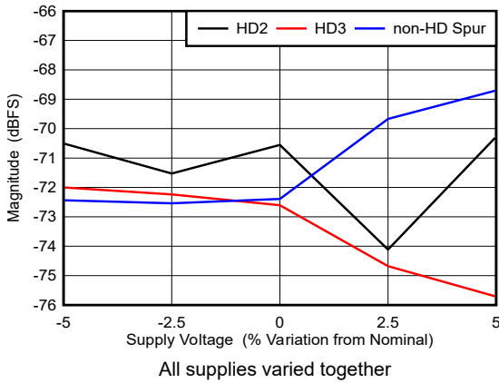
图 5-97. Dual Channel Mode: HD2, HD3 and Worst Spur vs Supply Voltage
