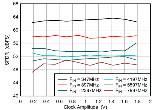
图 5-82. DES Mode: SFDR vs Clock Amplitude
