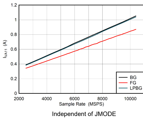
图 5-111. DES Mode: I_{VA11} vs Sample Rate
