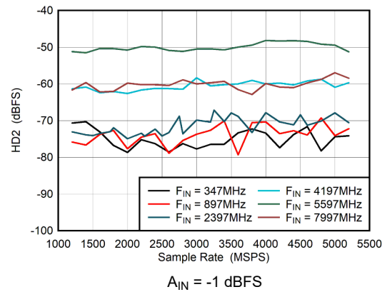
图 5-50. Dual Channel Mode: HD2 vs Sample Rate
