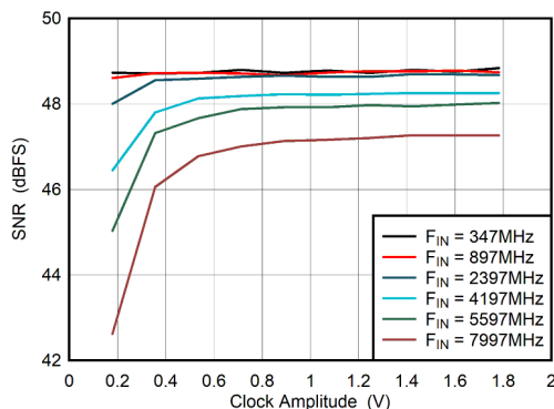
图 5-83. Dual Channel Mode: SNR vs Clock Amplitude
