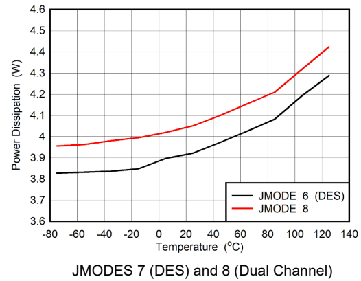
图 5-118. Power Dissipation vs Temperature
