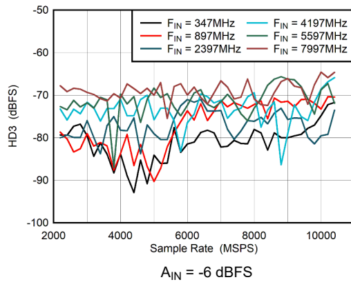
图 5-39. DES Mode: HD3 vs Sample Rate
