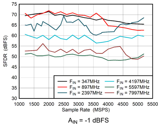
图 5-47. Dual Channel Mode: SFDR vs Sample Rate
