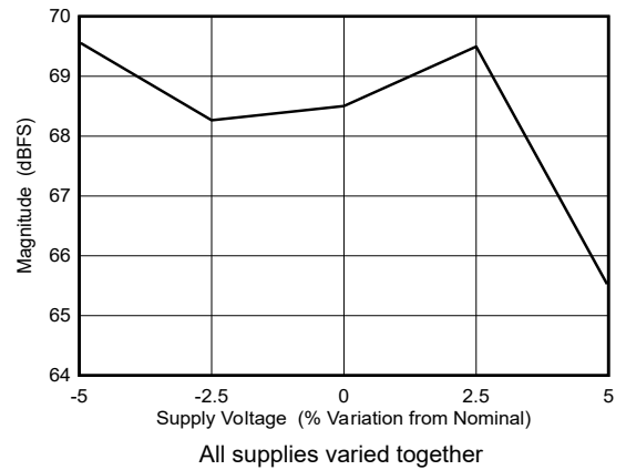
图 5-96. Dual Channel Mode: SFDR vs Supply Voltage
