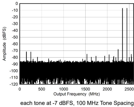
图 5-25. Dual Channel Mode: Two Tone FFT at 897 MHz
