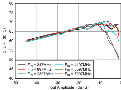
图 5-73. Dual Channel Mode: SFDR vs Input Amplitude
