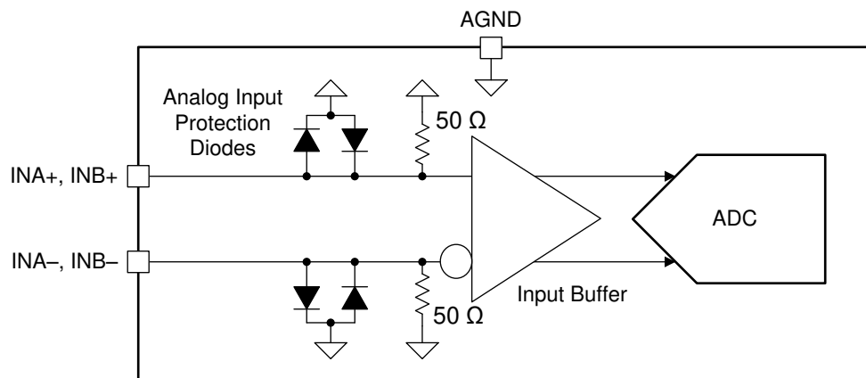
图 6-1. ADC08DJ5200RF Analog Input Internal Termination and Protection Diagram
