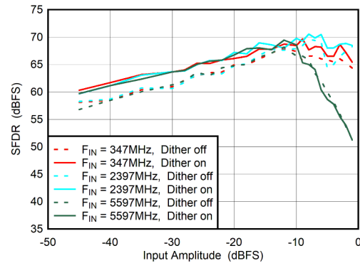
图 5-74. Dual Channel Mode: SFDR vs Input Amplitude and Dither
