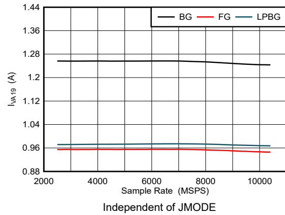
图 5-110. DES Mode: I_{VA19} vs Sample Rate
