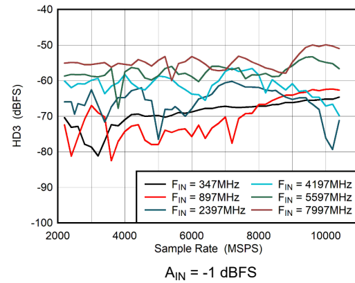
图 5-38. DES Mode: HD3 vs Sample Rate
