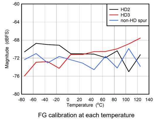
图 5-86. DES Mode: HD2, HD3 and Worst Spur vs Temperature
