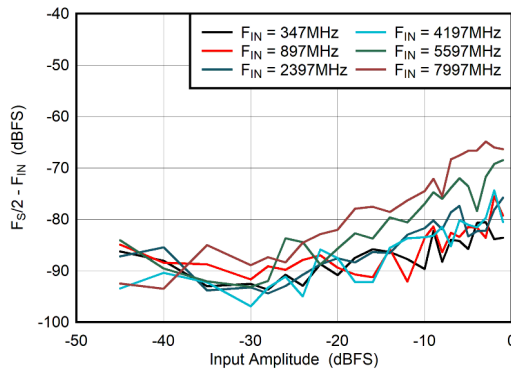
图 5-79. Dual Channel Mode: F_{S/2} - F_{\text{IN}} vs Input Amplitude
