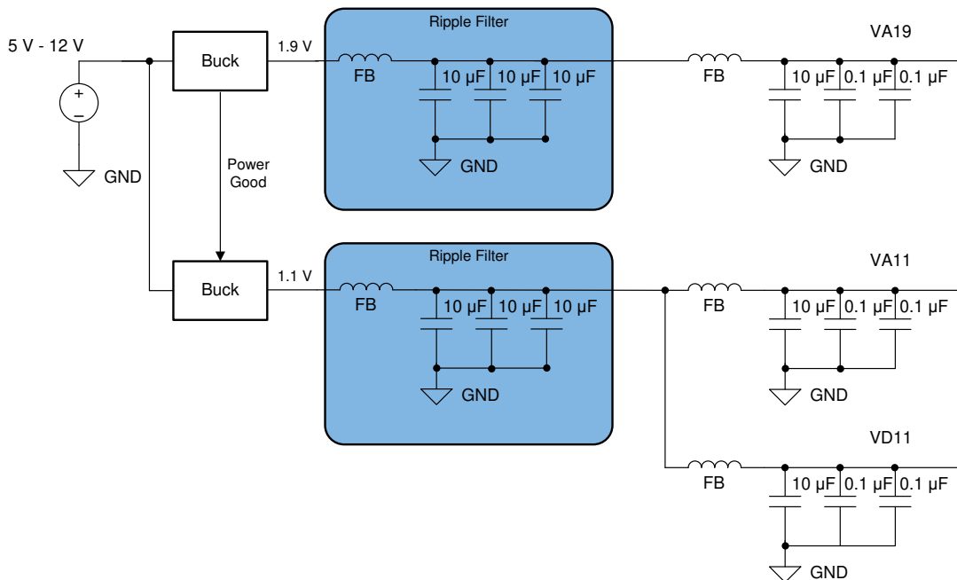
图 7-2. LDO Linear Regulator Approach Example
