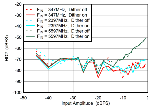
图 5-76. Dual Channel Mode: HD2 vs Input Amplitude and Dither
