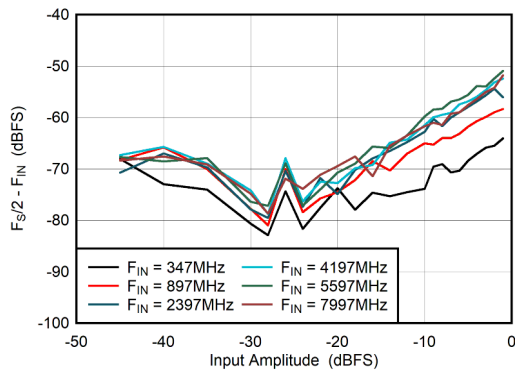
图 5-65. DES Mode: F_{S/2} - F_{\text{IN}} vs Input Amplitude
