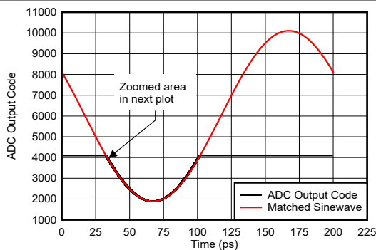
图 5-125. Sinewave Overdrive Recovery
