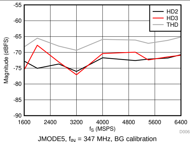
Figure 19. HD2, HD3, THD vs Sampling Rate
