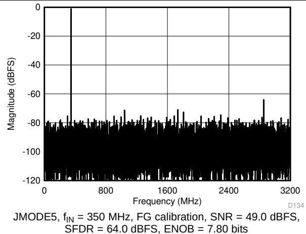
Figure 21. Single-Tone FFT at A_{\text{IN}} = -1\text{ dBFS}
