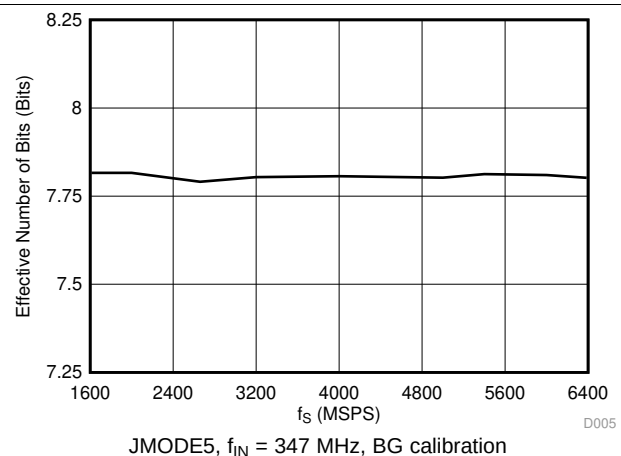
Figure 15. ENOB vs Sampling Rate
