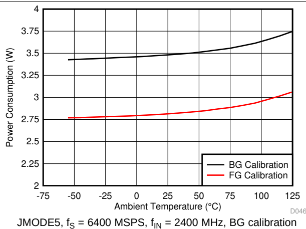
Figure 48. Power Consumption vs Temperature
