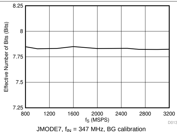
Figure 14. ENOB vs Sampling Rate
