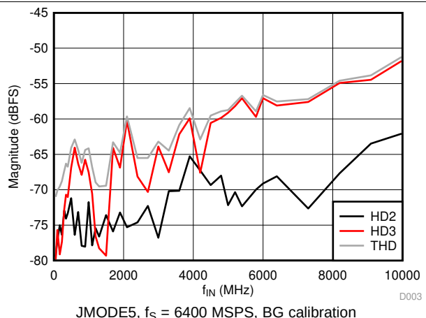
Figure 13. HD2, HD3, THD vs Input Frequency
