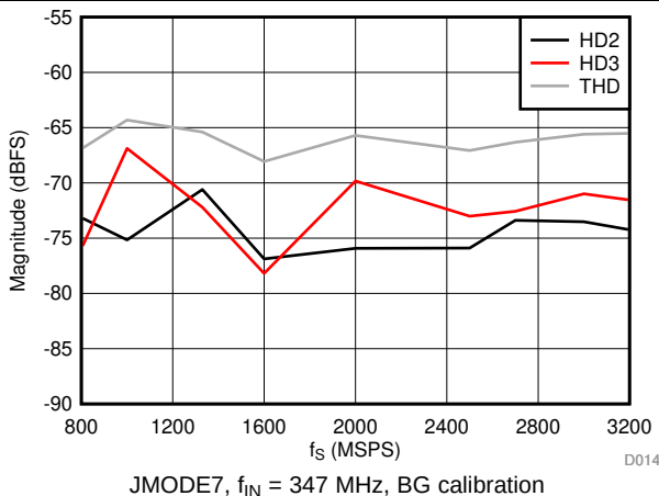
Figure 18. HD2, HD3, THD vs Sampling Rate
