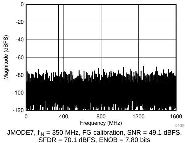
Figure 20. Single-Tone FFT at A_{\text{IN}} = -1\text{ dBFS}
