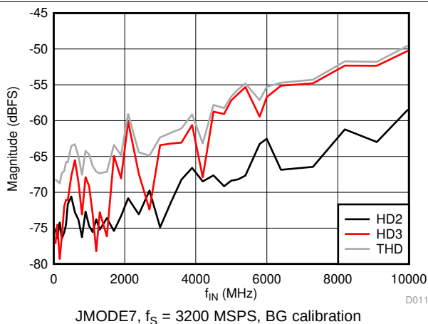
Figure 12. HD2, HD3, THD vs Input Frequency
