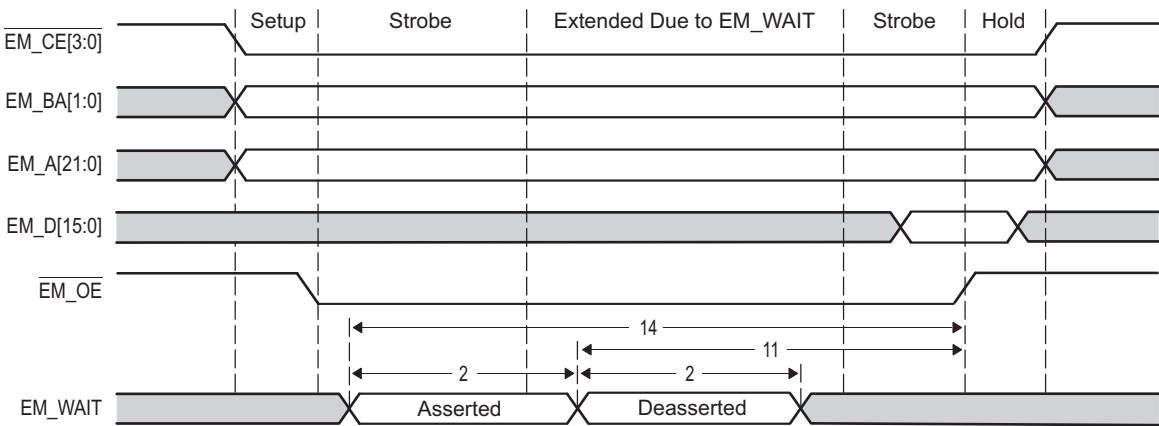
图 11-54. EMIF16 \text{EM\_WAIT} Read Timing Diagram
