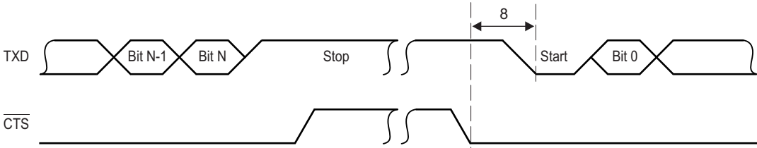
图 11-40. UART CTS (Clear-to-Send Input) — Autoflow Timing Waveform
