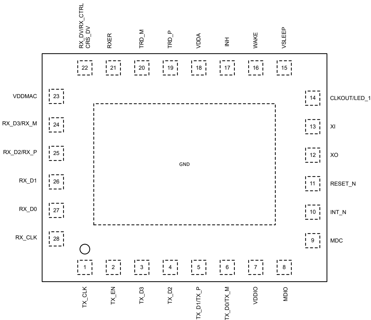
Figure 4-1. DP83TC813S-Q1 Pin Diagram
