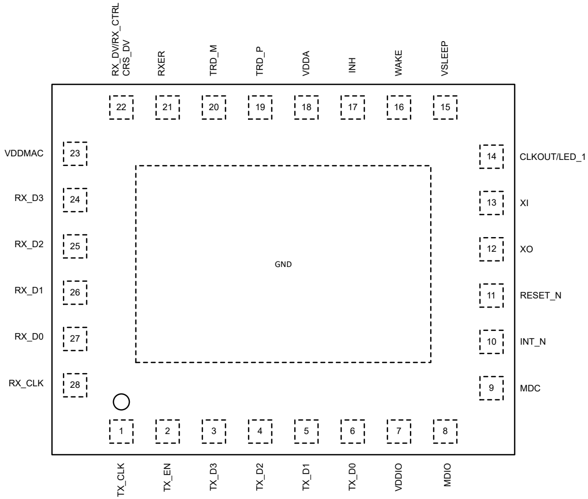
Figure 4-2. DP83TC813R-Q1 Pin Diagram
