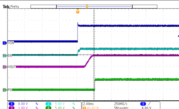
V_{IN} = 12V I_{OUT} = 8A 图 7-11. EN Start-Up – With Load
