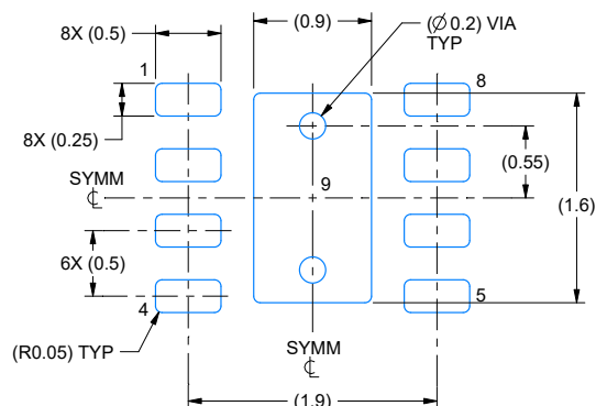
LAND PATTERN EXAMPLE SCALE:20X
