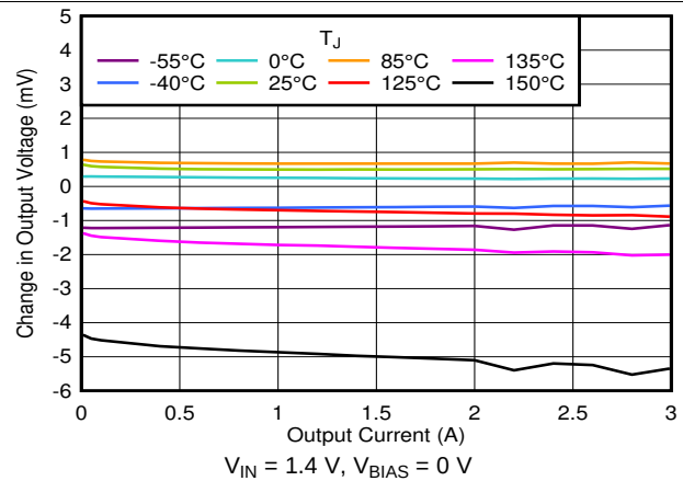
图 26. Load Regulation Without Bias
