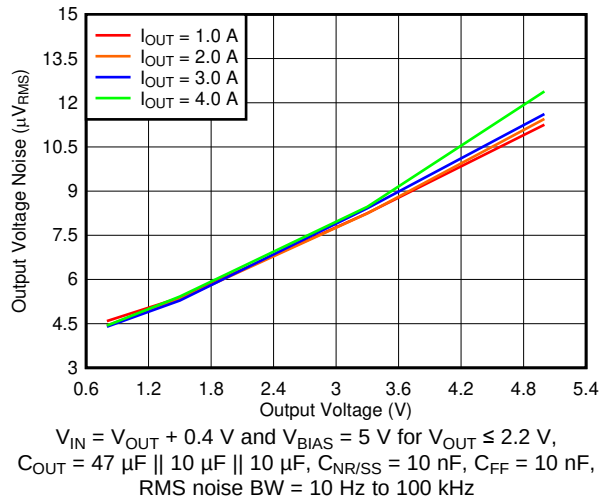
图 9. Output Voltage Noise vs Output Voltage and I_{OUT}
