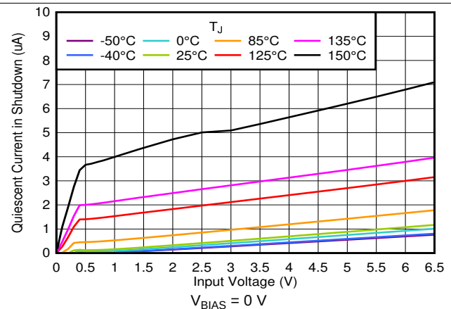
图 30. Shutdown Current vs Input Voltage
