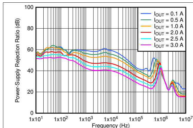
图 55. PSRR vs Frequency and I_{OUT} for V_{OUT} = 5.0 V
