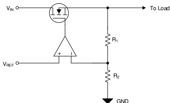
图 40. Simplified Regulation Circuit
