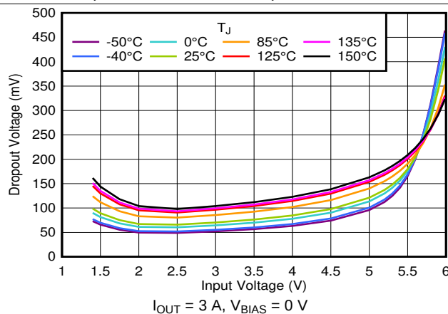
图 20. Dropout Voltage vs Input Voltage Without Bias
