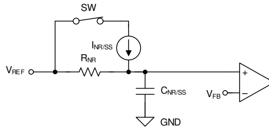
图 41. Simplified Soft-Start Circuit
