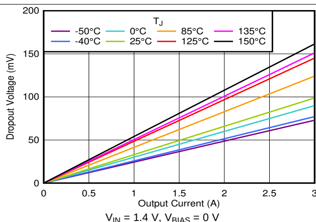
图 22. Dropout Voltage vs Output Current Without Bias
