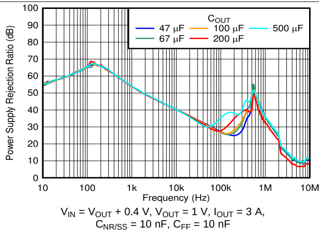
图 7. PSRR vs Frequency and C_{OUT}
