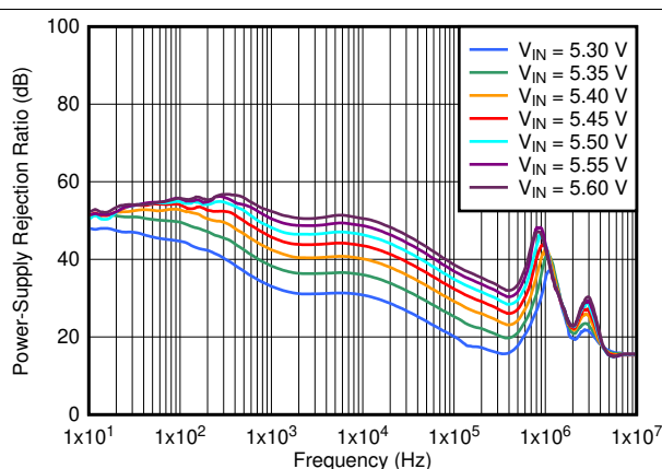
图 56. PSRR vs Frequency and V_{IN} for V_{OUT} = 5.0 V at I_{OUT} = 4.0 A
