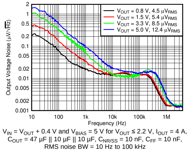
图 10. Output Voltage Noise vs Frequency and V_{OUT}
