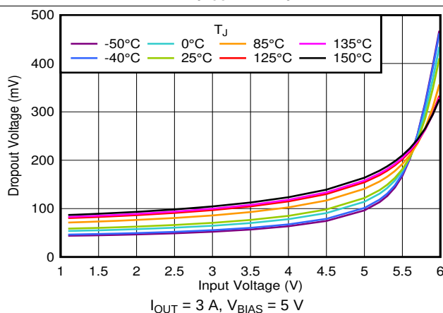
图 21. Dropout Voltage vs Input Voltage With Bias
