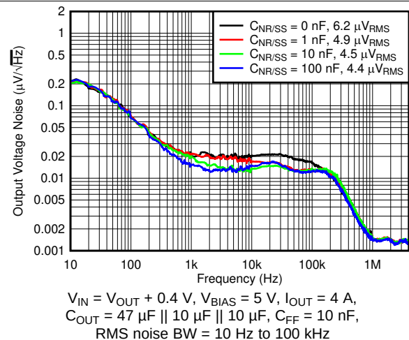
图 12. Output Voltage Noise vs Frequency and C_{NR/SS}
