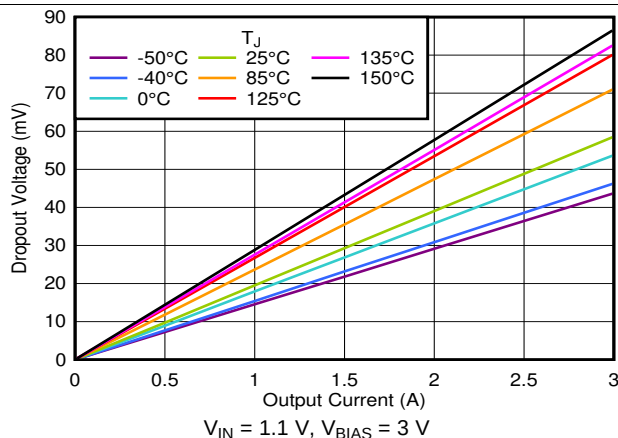
图 23. Dropout Voltage vs Output Current With Bias
