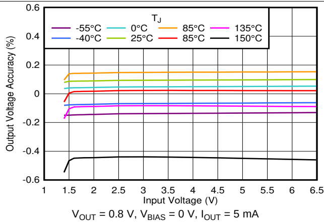
图 27. Line Regulation Without Bias
