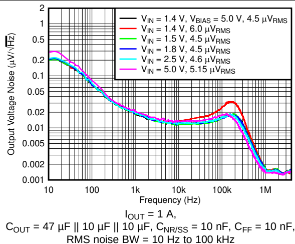
图 11. Output Voltage Noise vs Frequency and V_{IN}
