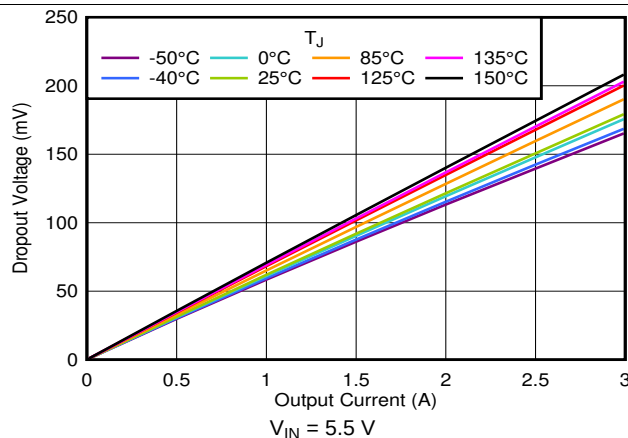
图 24. Dropout Voltage vs Output Current (High V_{IN} )
