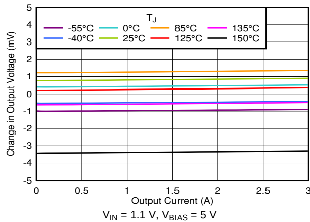
图 25. Load Regulation With Bias
